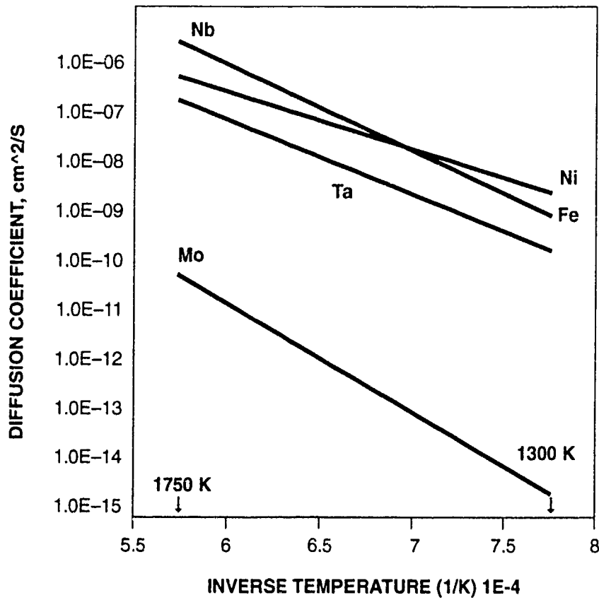
Figure 3. The diffusion coefficient of sulfur in several elements.
