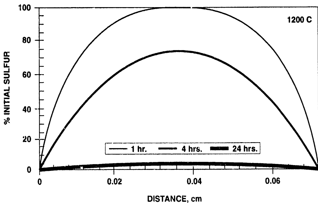
Figure 7. The position dependent concentration of sulfur in a 0.038cm (30mil) thick specimen hydrogen annealed at 1200°C.
