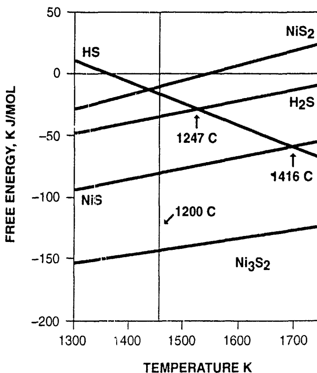
Figure 2. Gibbs free energies of formation for several compounds of sulfur.
