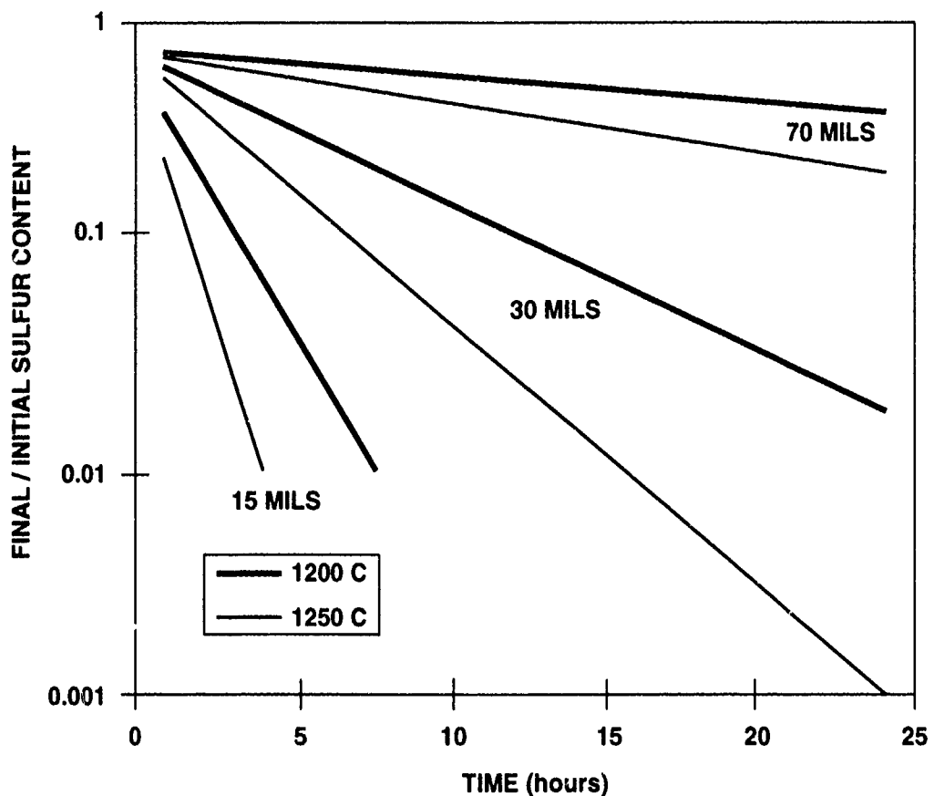
Figure 8. The calculated average composition of 0.038, 0.076, and 0.178cm (15, 30, and 70 mil) thick sheet annealed at 1200 and 1250°C.
