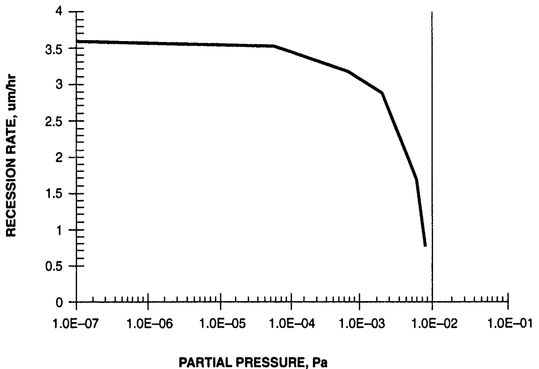
Figure 4. Calculated recession rate of a nickel specimen versus the environmental partial pressure of nickel.
