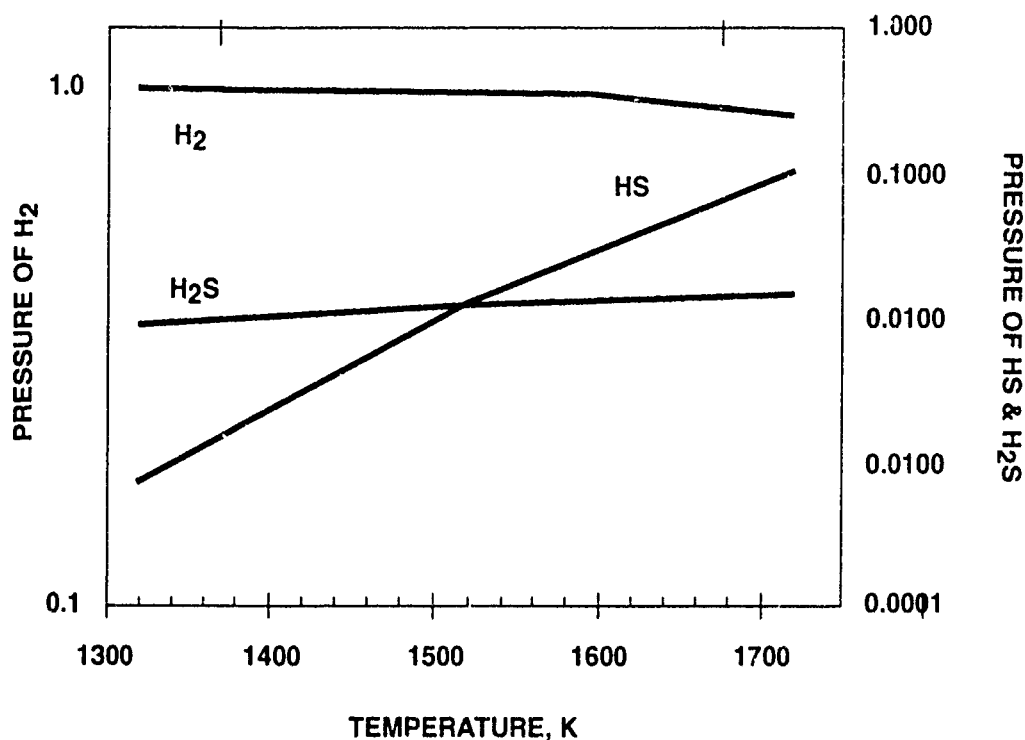
Figure 5. The calculated equilibrium partial pressures of HS, H_2S , and H_2 during the desulfurization of nickel.
