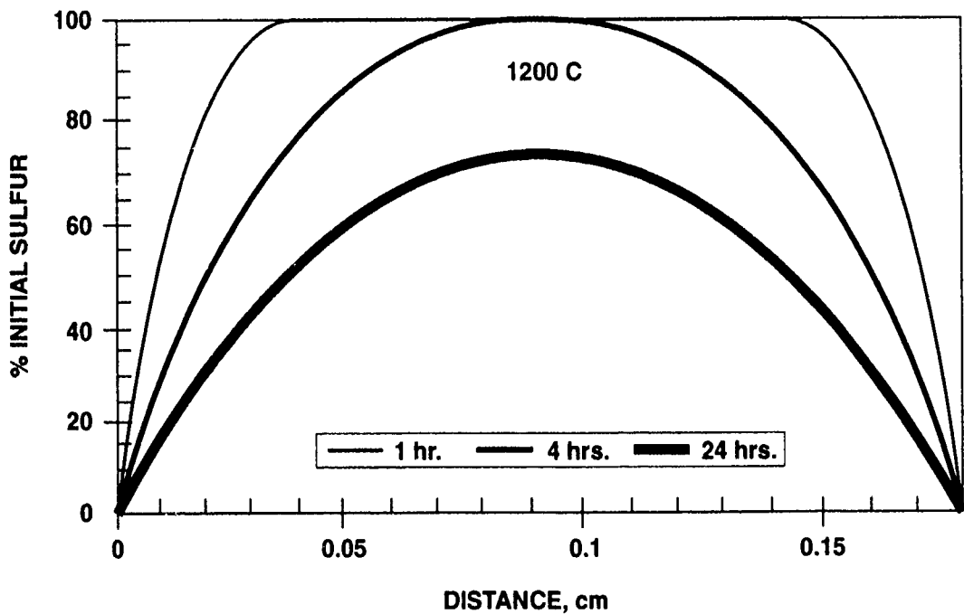
Figure 6. The position dependent concentration of sulfur in a 0.178cm (70 mil) thick specimen hydrogen annealed at 1200°C.
