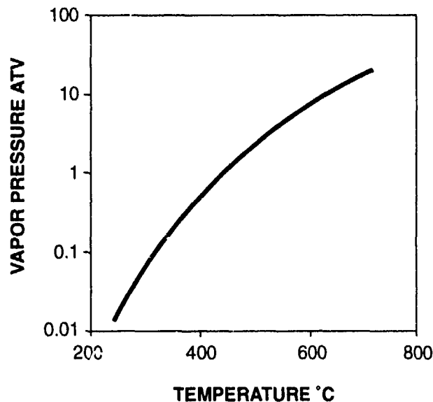
Figure 1. Vapor pressure of elemental sulfur as a function of temperature.
