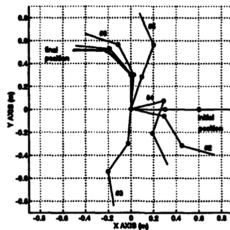
Figure 10: Animation of the 3-link manipulator. Experiment #5.
