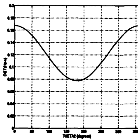
Figure 3: Determinant of M_{pd} for the 2-link manipulator.
