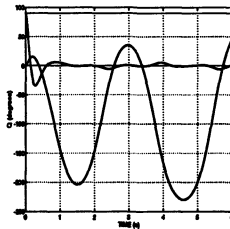
Figure 12: Response of the 2-link manipulator. Experiment #2 with control law from [1].
