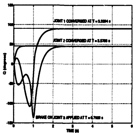
Figure 9: Response of the 3-link manipulator. Experiment #4.
