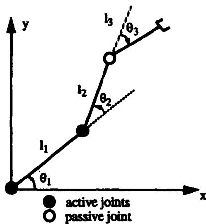
Figure 1: Three-link manipulator with one passive joint.
