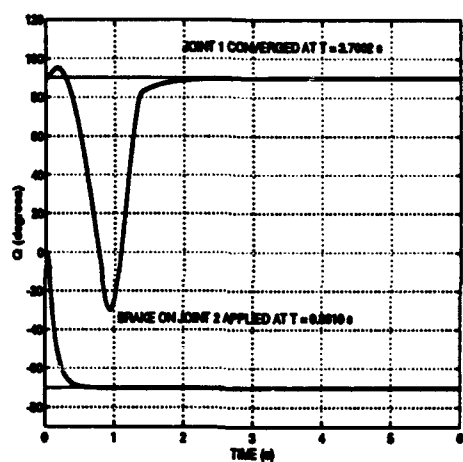
Figure 8: Response of the 2-link manipulator. Experiment #3.
