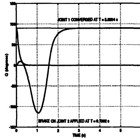
Figure 5: Response of the 2-link manipulator. Experiment #1.
