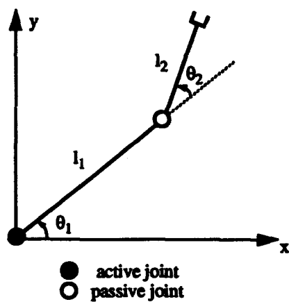
Figure 2: Two-link manipulator with one passive joint.
