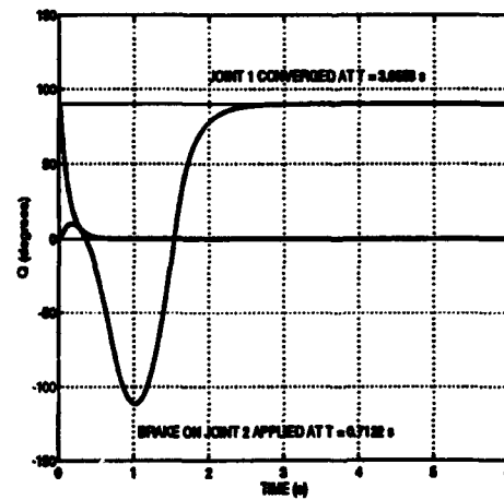
Figure 6: Response of the 2-link manipulator. Experiment #2.
