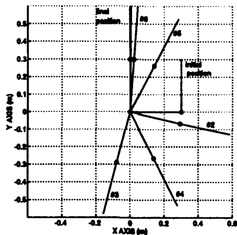
Figure 7: Animation of the 2-link manipulator. Experiment #2.
