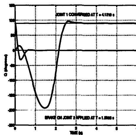
Figure 11: Response of the 2-link manipulator. Experiment #1 with control law from [1].
