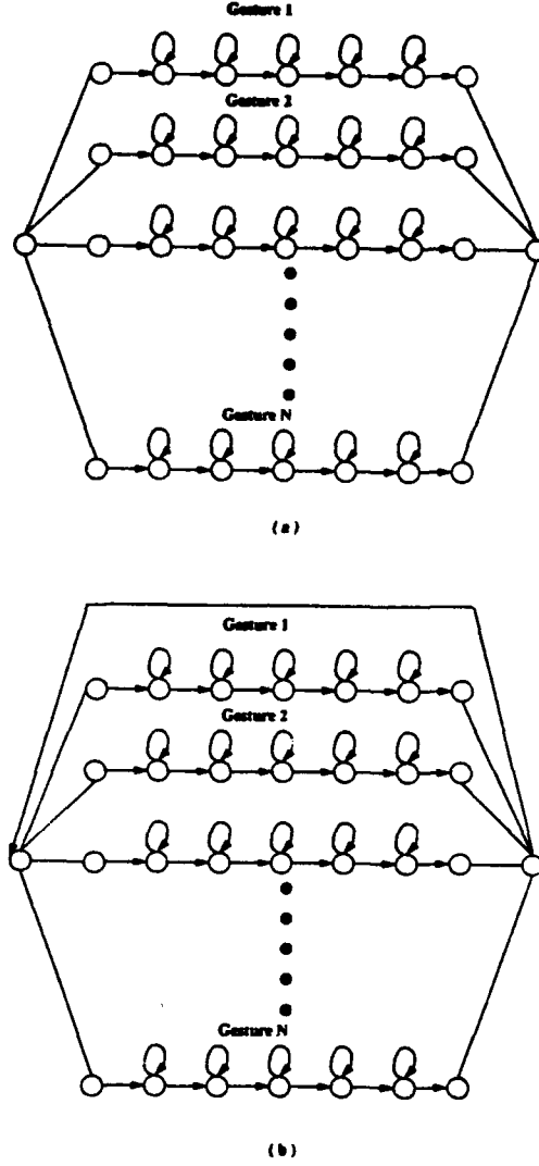
Figure 1: HMM networks for gesture recognition without adding knowledge source.
