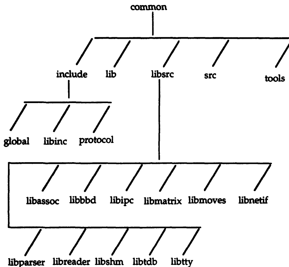
Figure 4.3.2.2 Masscomp MCC common directory structure
