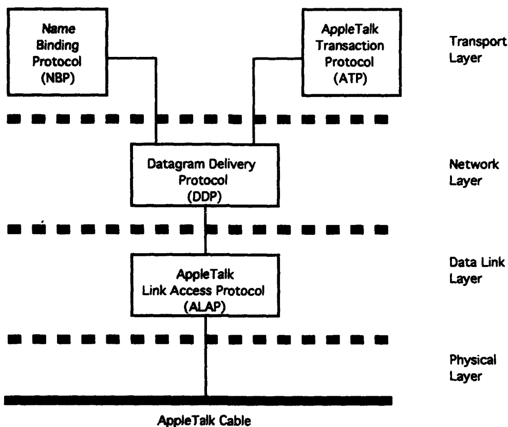
Figure 3.1.2.1 AppleTalk protocols used by the MCC system
