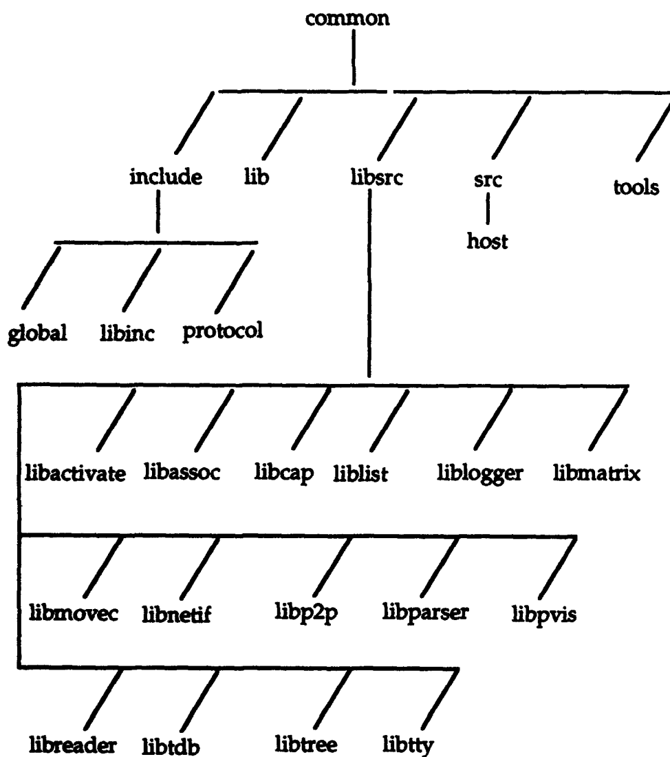
Figure 4.1.2.2 MIPS MCC /saf/common directory structure
