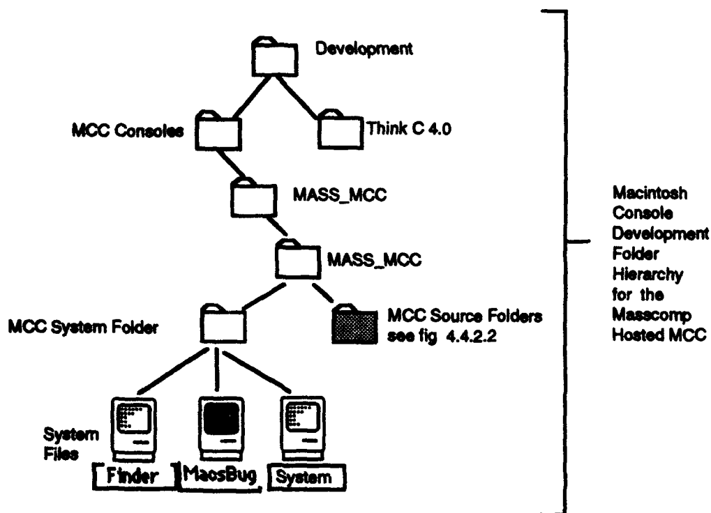
Figure 4.4.2.1 Top Level Macintosh Development Folder Structure
