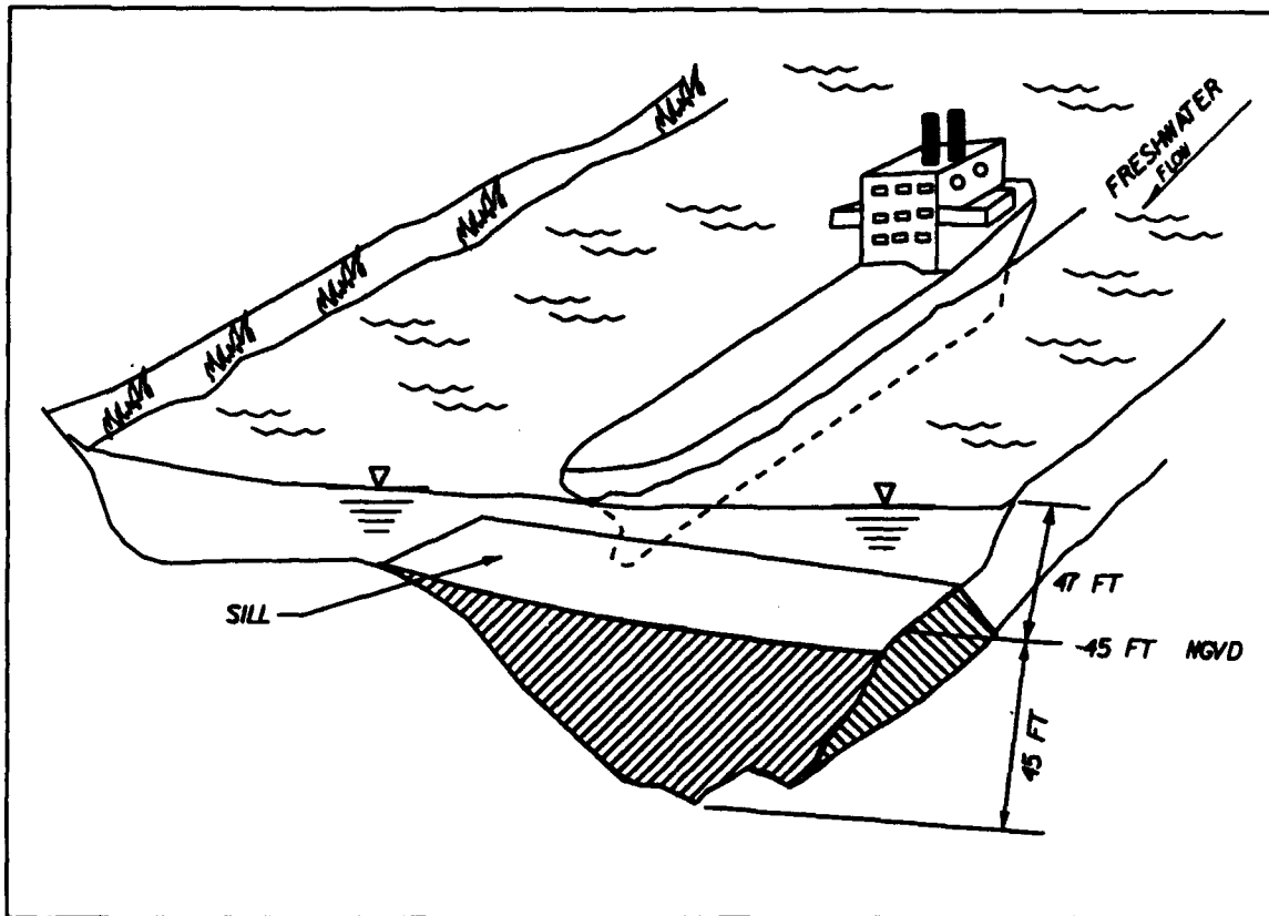
Figure 6. Salt barrier sill in the Mississippi River
