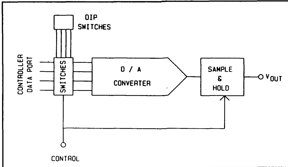
Figure 23. DAC block diagram
