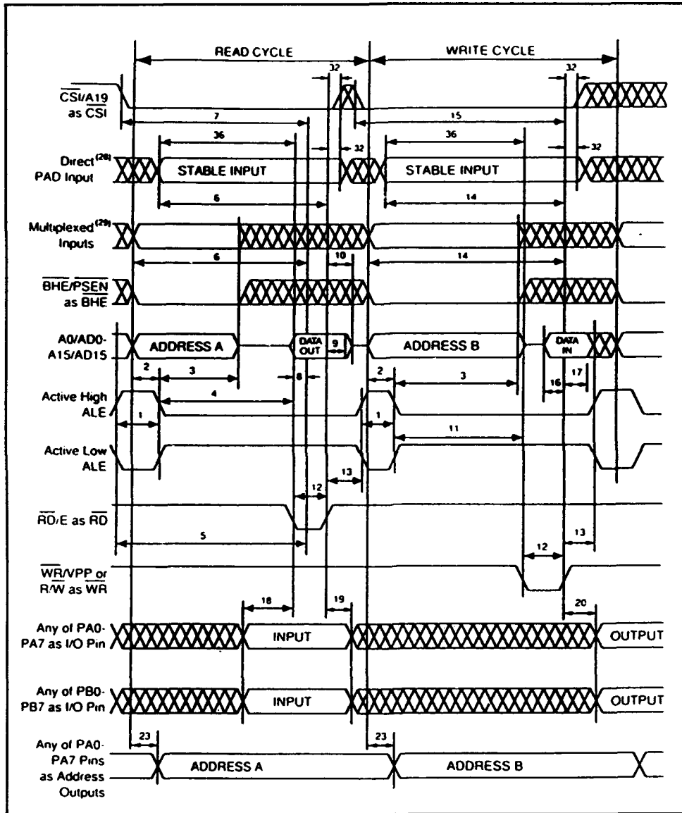
Figure C5. Programmable logic device timing - read and write
