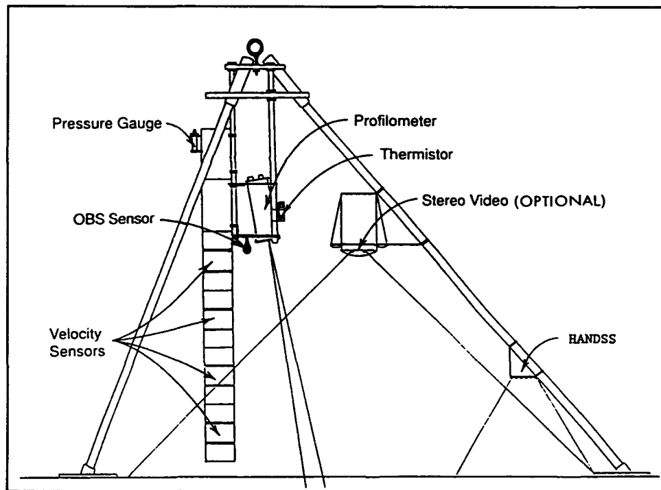
Figure 14. ARMS tripod
