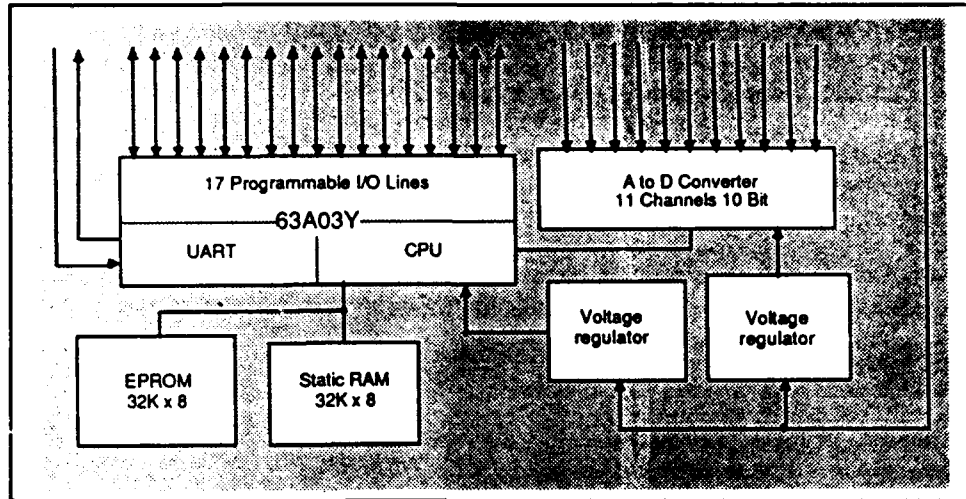
Figure 4. Tattletale V
