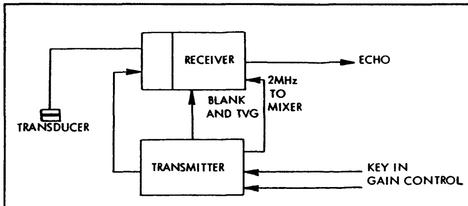
Figure 2. ACP electronic characteristics
