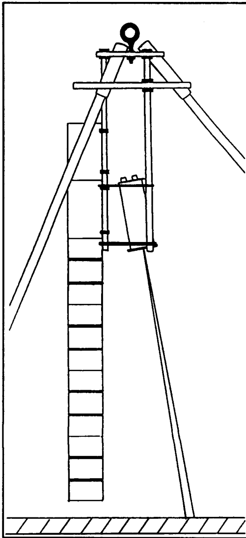
Figure 13. BASS-ACP positioning
