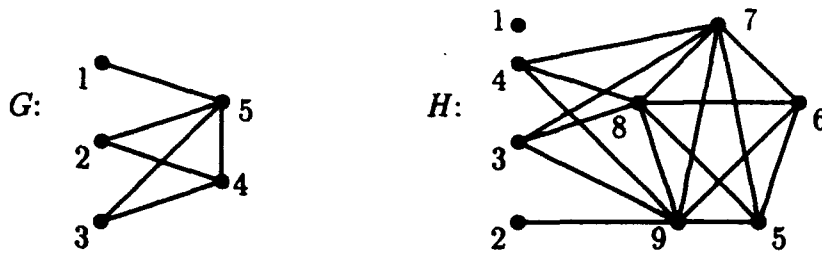
FIG. 1. Two split graphs. Both are threshold graphs, as well.
