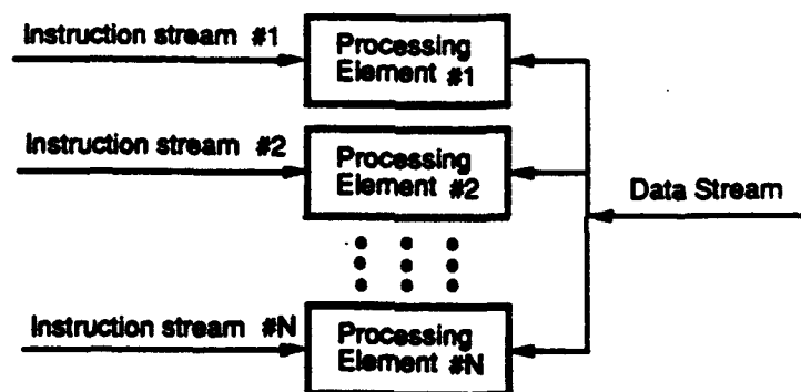
c) MISD computer
