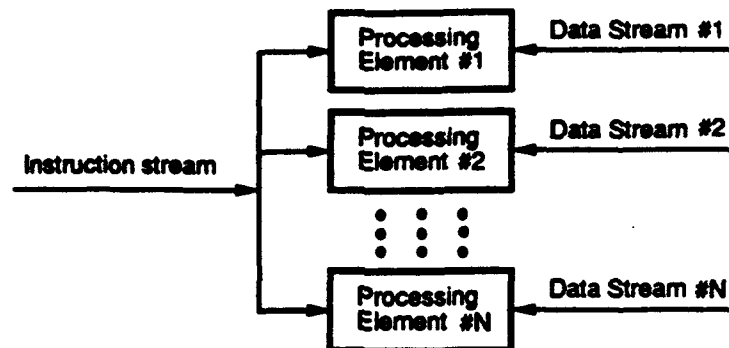
b) SIMD computer
