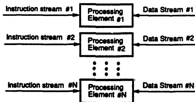
d) MIMD computer
