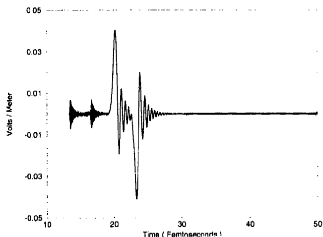
Fig. 4. A transmitted pulse induced by an incident signal as shown in Fig. 2, but at optical frequencies and just micrometers into the medium.
