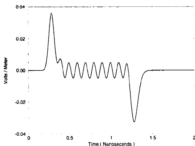
Fig. 3. The pulse of Fig. 2 after passage through 1 cm of pure water.
