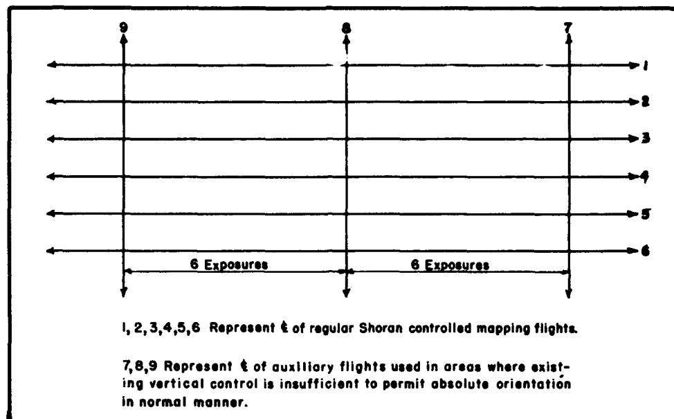
FIG. 4-1. FLIGHT PLAN FOR USE IN SHORAN MULTIPLEX MAPPING OF AREAS WITH LITTLE OR NO VERTICAL CONTROL.
