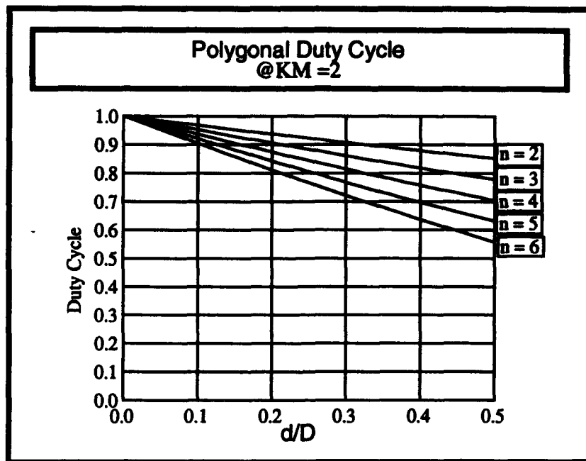
Figure 24 - Duty Cycle
