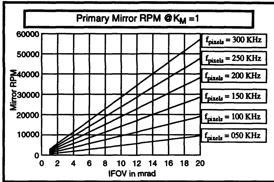
Figure 21 - Mirror RPM
