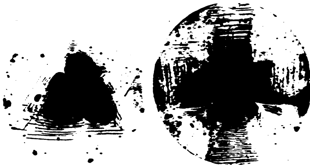
Fig. 1. Press patterns on Cu-crystal (after Tamman and Muller). Left: octahedron face, magnification 52X; right: cube face, magnification 88X.
