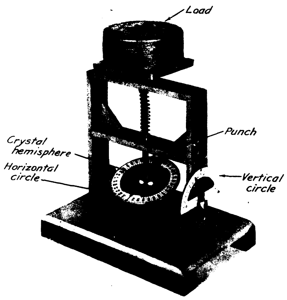
174-3-23 Fig. 3. Pressing goniometer with horizontal and vertical circles.
