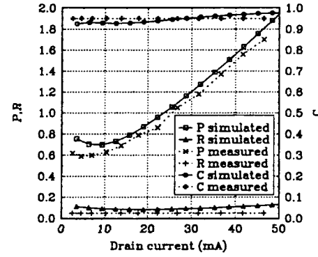
Fig. 4 Measured and modelled noise source parameters as a function of the drain current ( V_{off} = -0.5 \text{ V} , L_g = 0.25 \mu\text{m} , d = 25 \text{ nm} , Z = 160 \mu\text{m} , U_{ds} = 1 \text{ V} , v_{sat} = 2.6 \cdot 10^7 \text{ cm}^2/\text{s} , \gamma = 1.25 , \delta = 2.7 , D_H = 25 \text{ cm}^2/\text{s} )
