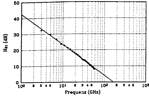
Fig. 1 Current gain versus frequency for a 0.25 \mu\text{m} InAlAs/InGaAs HEMT ( U_{ds} = 1.2 \text{ V} , U_{gs} = -0.25 \text{ V} , I_d = 45 \text{ mA} , Z = 160 \mu\text{m} )
