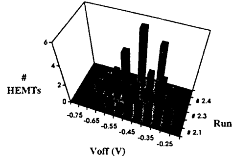
Fig. 2 Threshold voltage distribution of 3 HEMT process runs
