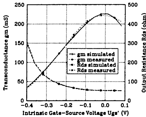
Fig. 5 Transconductance and output resistance vs. gate-source voltage modelled and measured ( U_{ds} = 1 \text{ V} , L_g = 0.25 \mu\text{m} , Z = 160 \mu\text{m} , )
