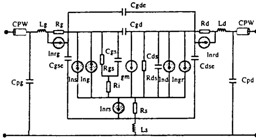
Fig. 3 Small-signal and noise equivalent circuit
