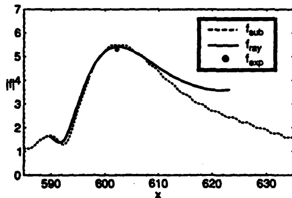
Fig. 5 - Superposition of backwards wave and specular contributions to the form function based on Eq. (2), a modified PWS result, and experiments.
