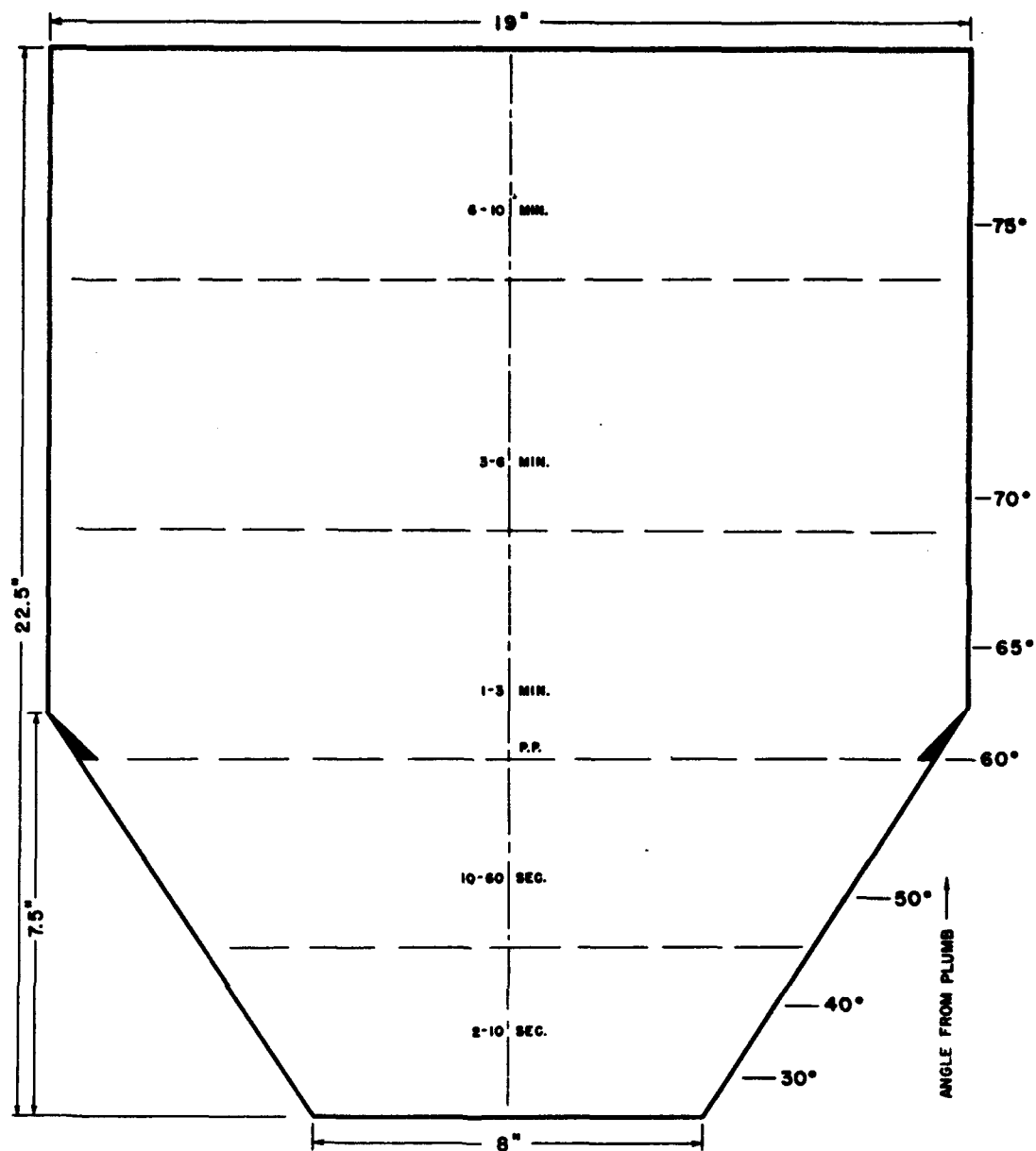
Fig. 23. Exposure time for tri-metron rectification using modified Bausch and Lomb rectifier.
