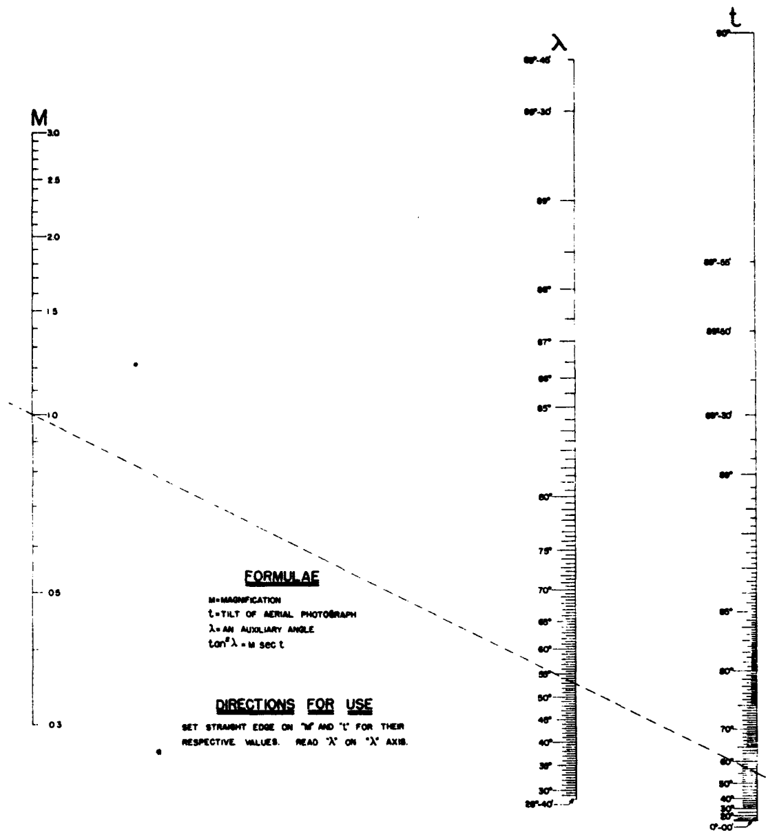
Fig. 14. Nomogram for determination of value of λ for settings on modified Bausch and Lomb rectifier.
