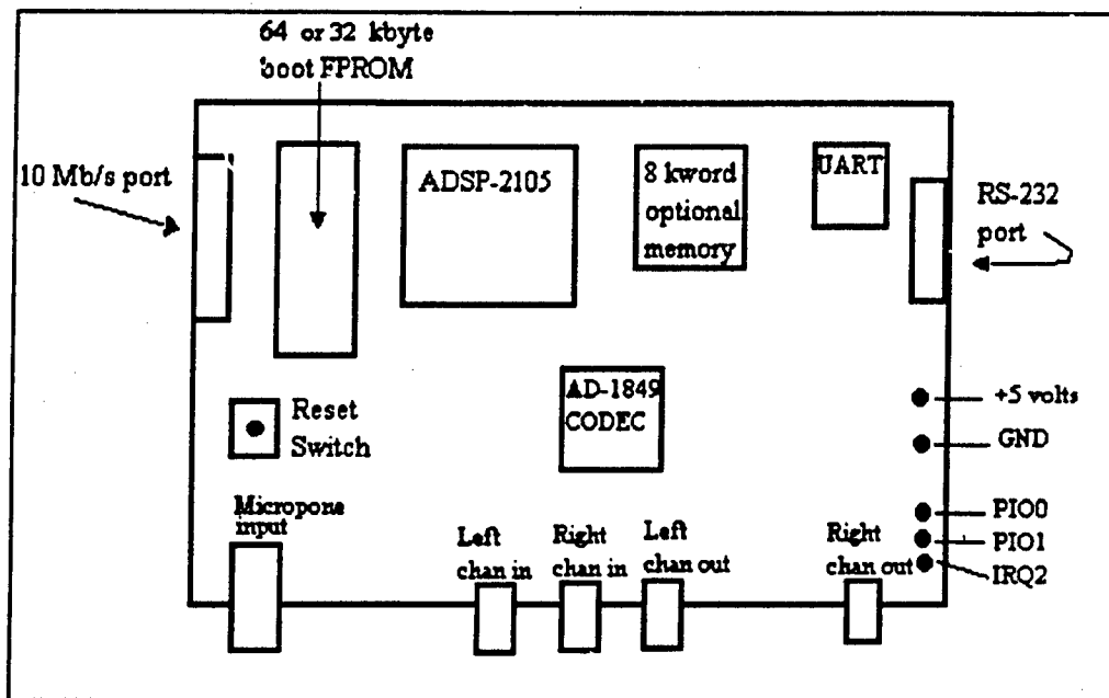
Figure 3 EMB-1601A Board Layout
