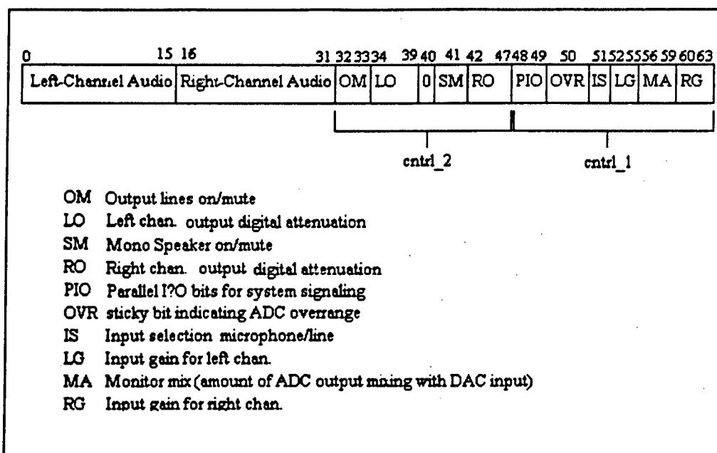
Figure 8 16-Bit Stereo Data Word
