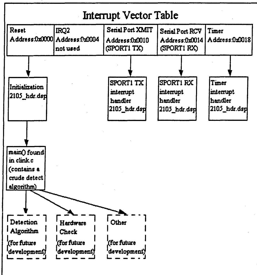
Figure 6 Program Structure Chart
