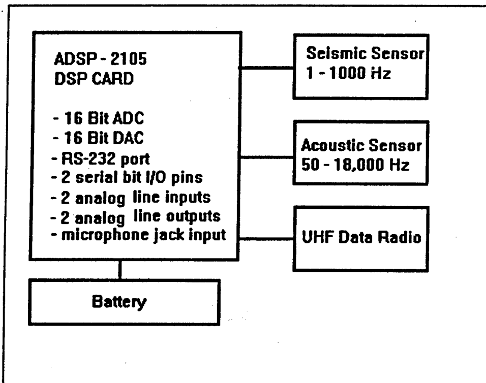
Figure 1 Unattended ground Sensor
