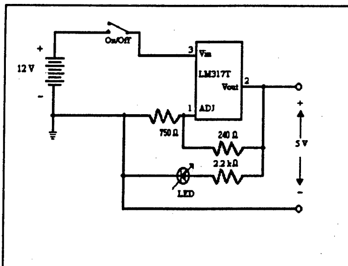
Figure 5 +5 volt DSP Power Supply
