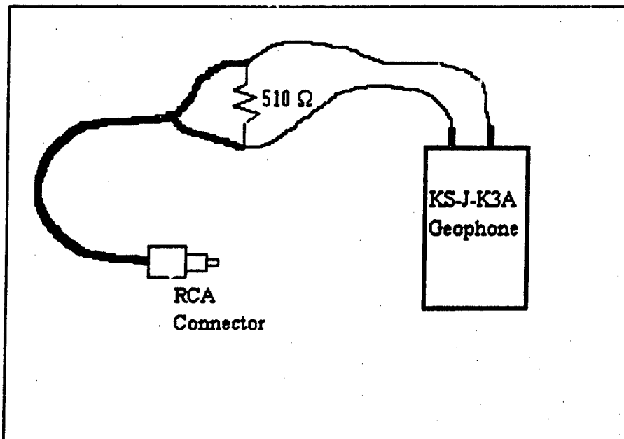
Figure 4 HS-J-K3A Geophone with RCA Connector.
