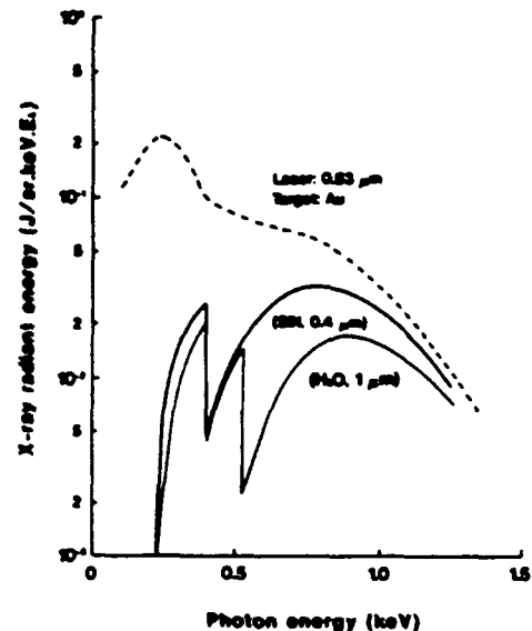
Fig. 8. X-ray spectra of a source, level 1 (after the SiN window, and level 2 (after the water layer).
