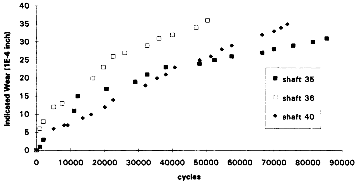
Figure 9. Indicated wear for 69.4 ksi test for Coating II applied by NAWCADWAR versus X1200S liner with fluid contamination.
