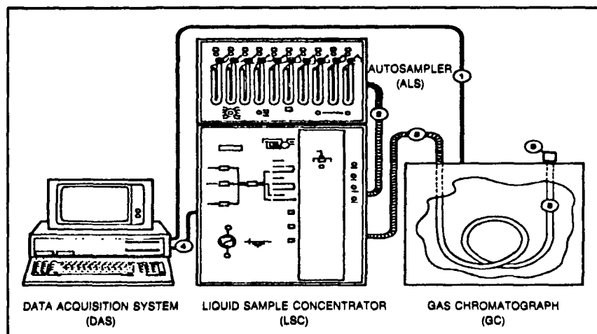
Schematic for computer-controlled Instrument.
