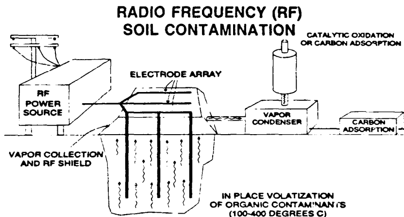
Diagram of RF soil venting.
