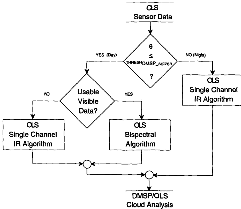
Figure 10. DMSP/OLS Cloud Analysis Algorithm Approach
