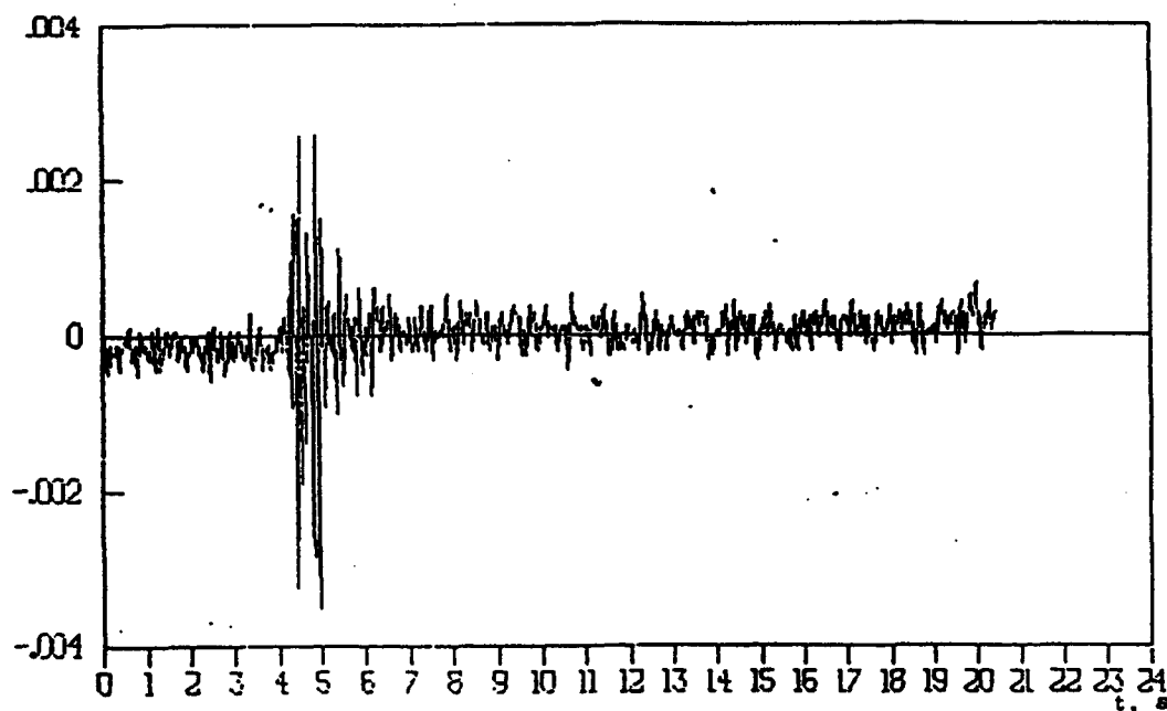
Figure 41: Underground explosion detonated on August 29, 1993; point No. 3. Variations of seismic wave acceleration vs. time. High frequency filter was used.
