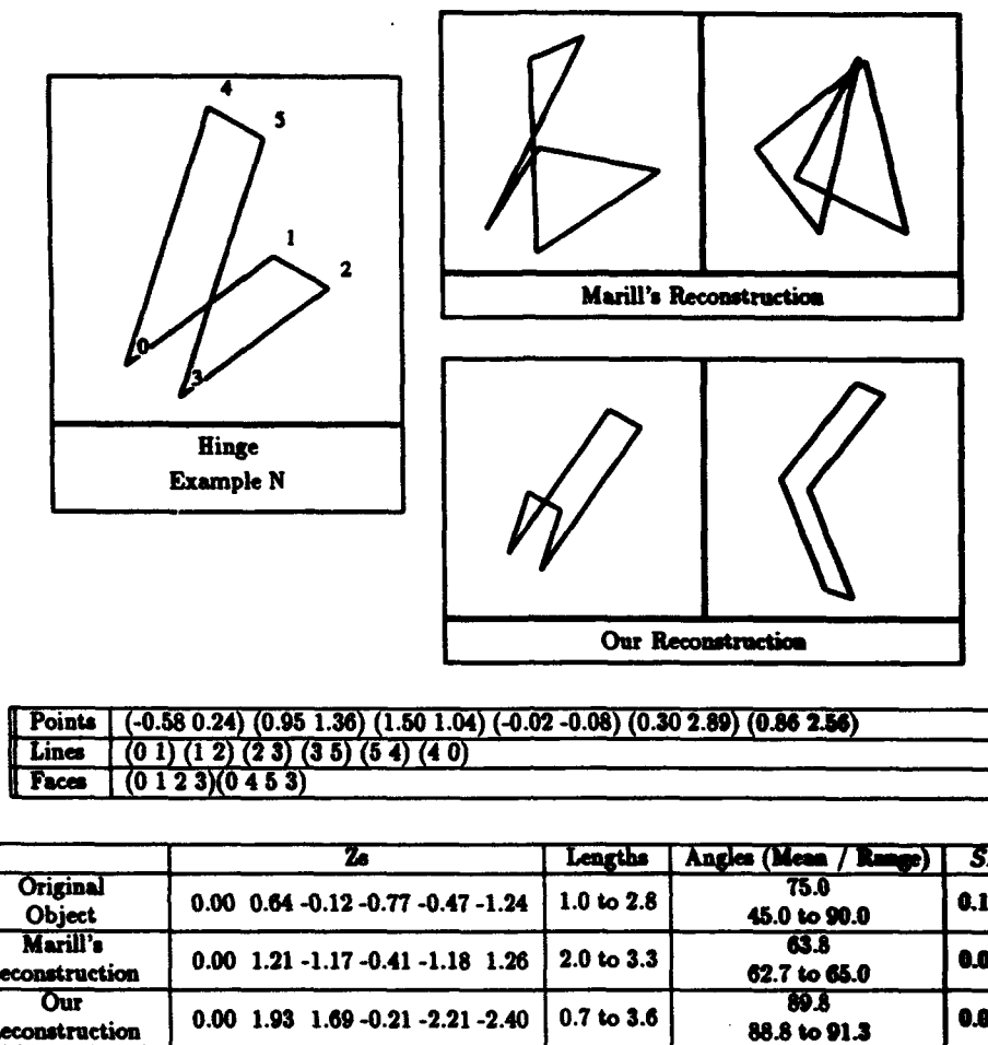
Fig. 6 Example N. The SDA of Marill's unacceptable reconstruction is again significantly lower than that of the psychologically plausible original object.
