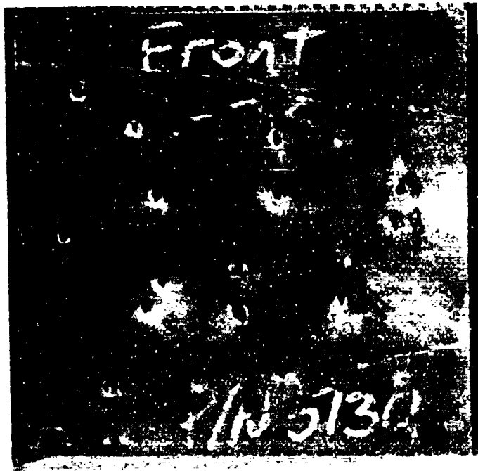
ARL•MD Ballistic Test Number 012-93. Front Side. 0.197 inch thick AerMet 100™ Steel versus U.S. 0.30 caliber AP M2 projectile. (Austenitized @ 1625°F, 1 hour, air cool; -100°F, 1 hour, air warm; Aged @ 875°F, 1 hour, air cool.)
