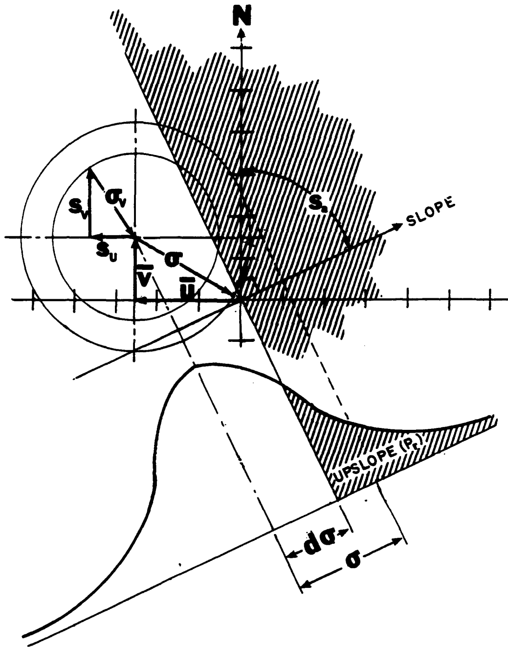
Figure 6. Geometry of the Problem of Computing Upslope Probability Given the Vector Mean Wind Components \bar{U} , \bar{V} and Standard Deviations S_u and S_v . Probability of Upslope P_u is Obtained Knowing the Standardized Distance d\sigma Along the x Axis of the Univariate Normal Distribution. This Distance is Governed by the Perpendicular to the Line of the Azimuth Angle S_s of the Slope of the Terrain of a Given RTNEPH Box.
