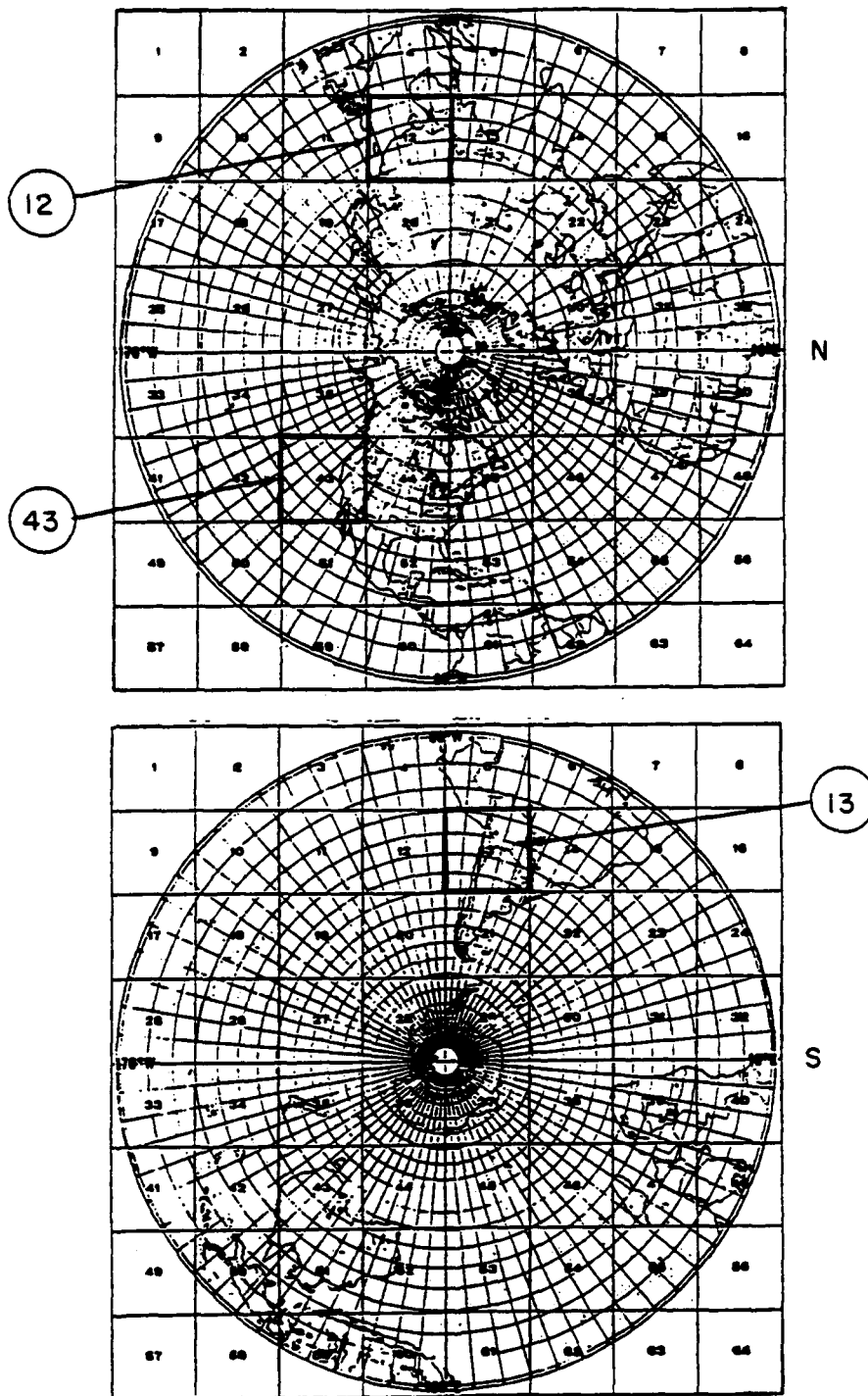
Figure 2. The Northern (Top) and Southern (Bottom) Polar Stereographic Map Projections used for Archiving the RTNEPH Data. The 64 Mesh Large Boxes Within Each Map are Indicated. The RTNEPH Grid Boxes 12 and 43 in the Northern Hemisphere and Box Number 13 in the Southern Hemisphere are the Areas of Study.
