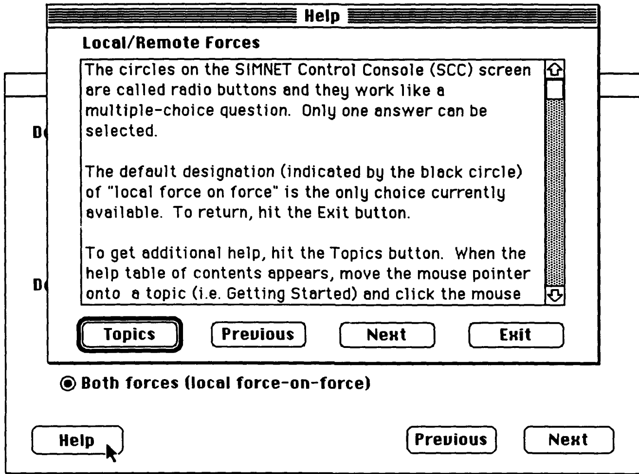
Figure 3.6 Help Screen
