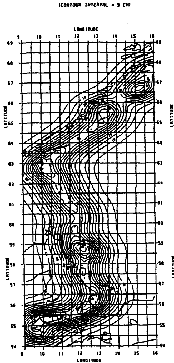
Figure 5.9 Height Bias Function Plot using Scandinavian GPS Traverse Data/UELN Heights
