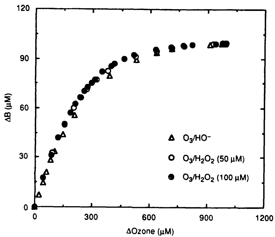
Figure 27. Efficiency Comparisons of the O_3/H_2O_2 /Dark System with Different Concentrations of H_2O_2 .
