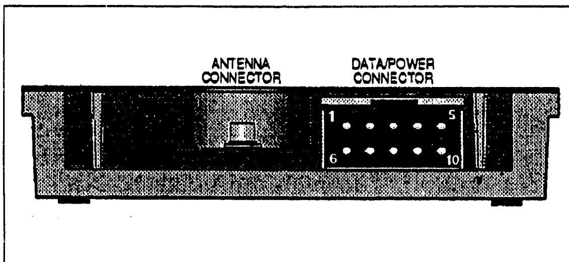
Figure 32. Side View Of The PVT-6 Showing The Pin Numbering Order. (Motorola, 1992, p. 3-2)
