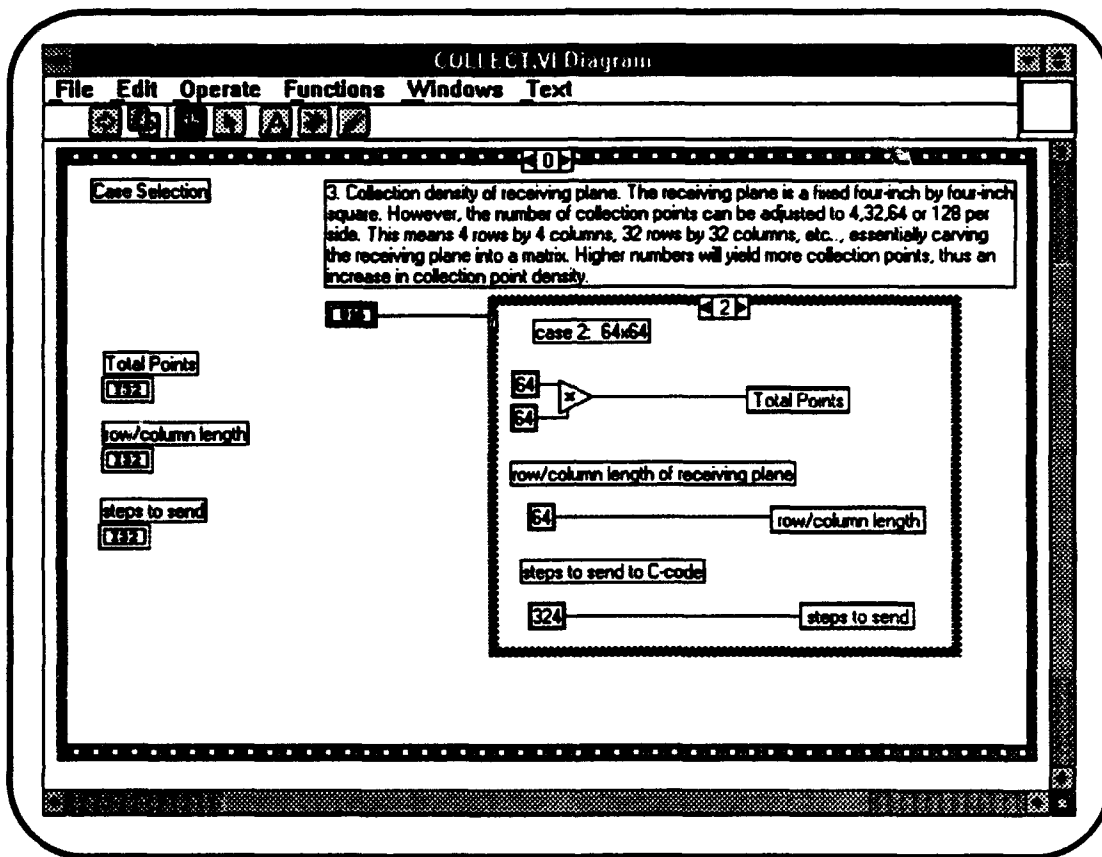
Figure 6. Block Diagram 02. 64x64 Collection Density Setup.
