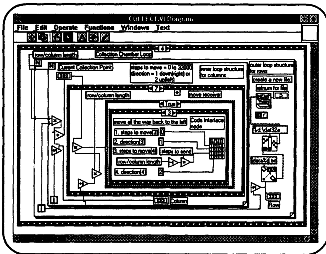
Figure 25. Block Diagram 47T3. Move Receiver Left.
