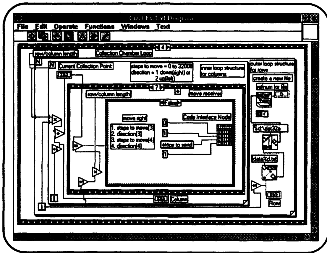
Figure 27. Block Diagram 47F. Move Receiver Right.
