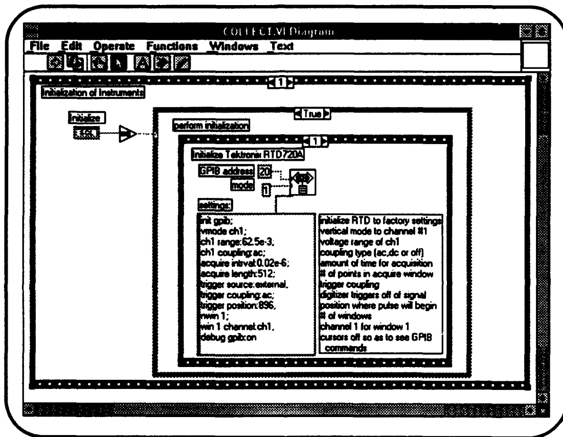
Figure 10. Block Diagram 1T1. Initialization of Tektronix RTD720A.
