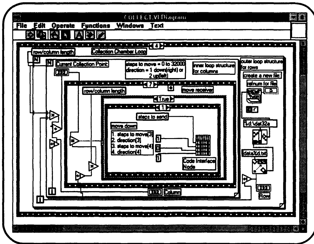
Figure 23. Block Diagram 47T1. Move Receiver Down.
