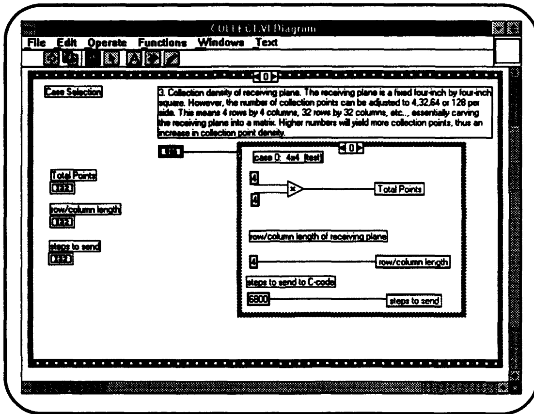
Figure 4. Block Diagram 00. 4x4 Collection Density Setup.
