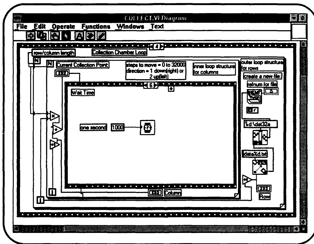
Figure 21. Block Diagram 46. Wait Time of 1.0 Seconds.
