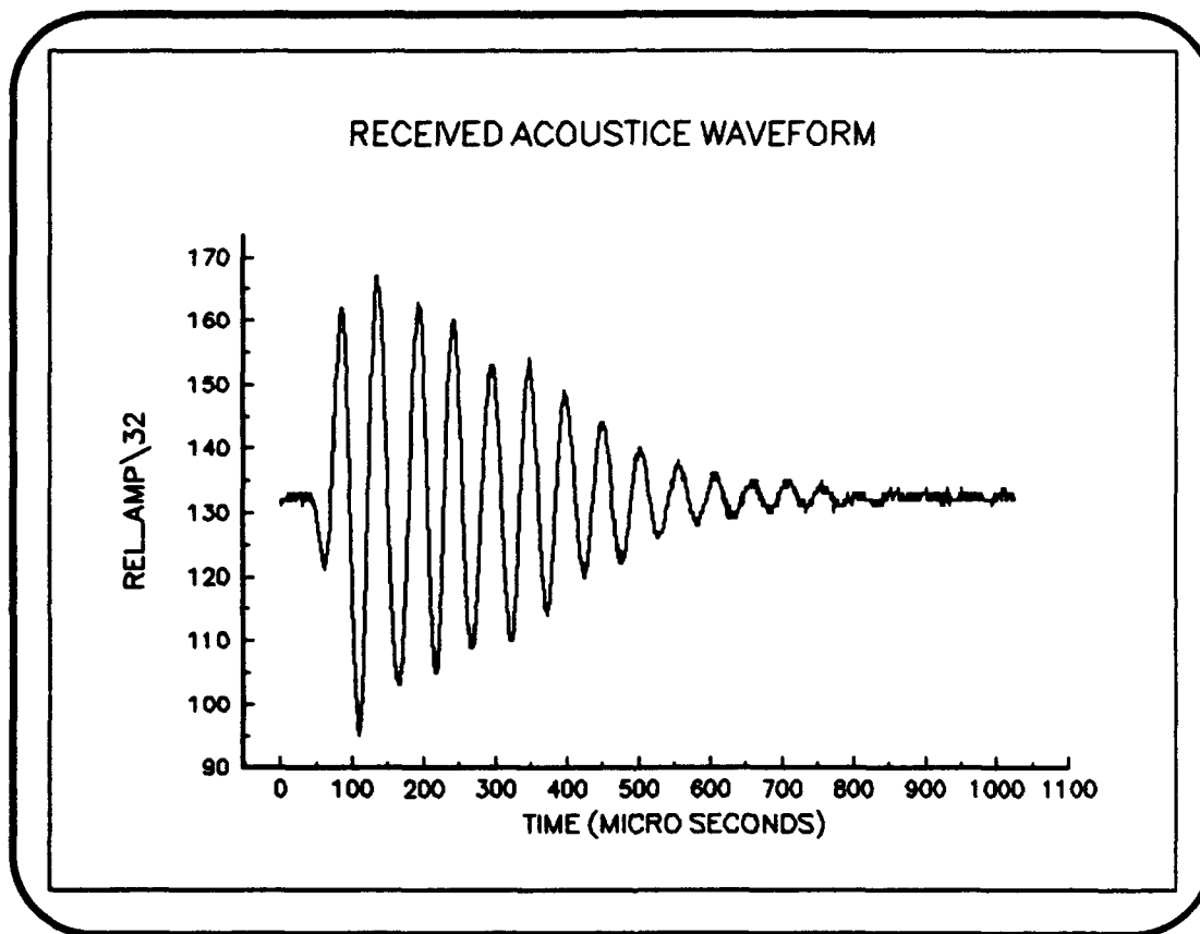
Figure 29. Waveform Pulse from a 64x64 Collection Density.
