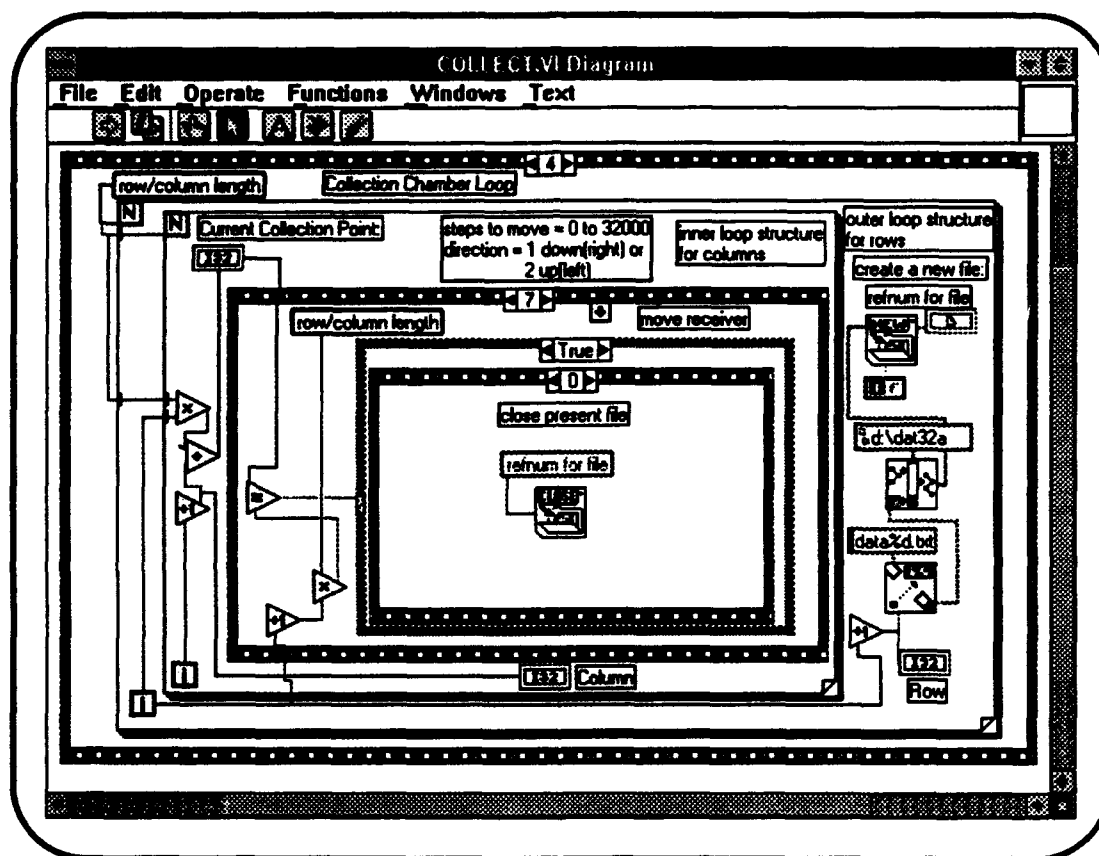
Figure 22. Block Diagram 47T0. Close Current File.
