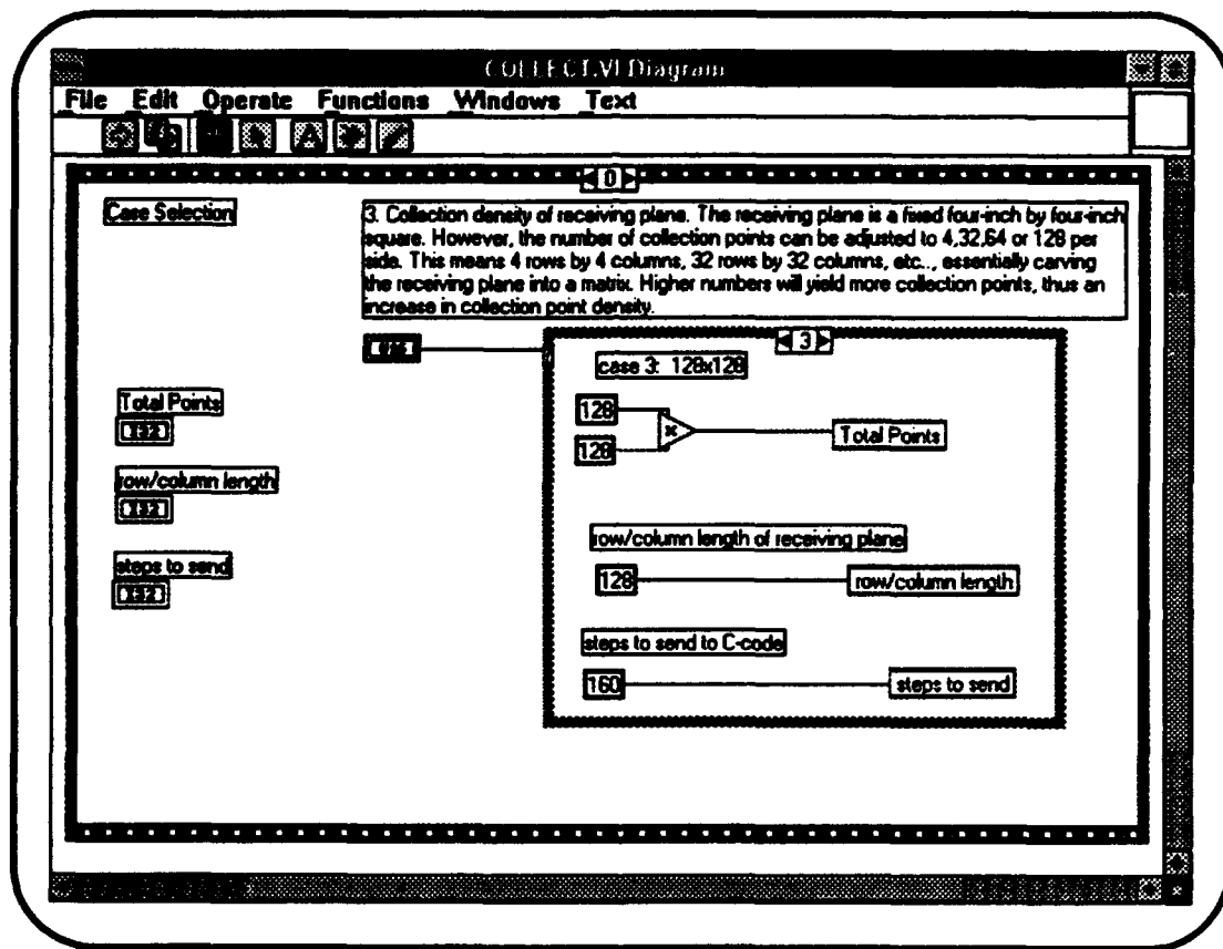
Figure 7. Block Diagram 03. 128x128 Collection Density Setup.
