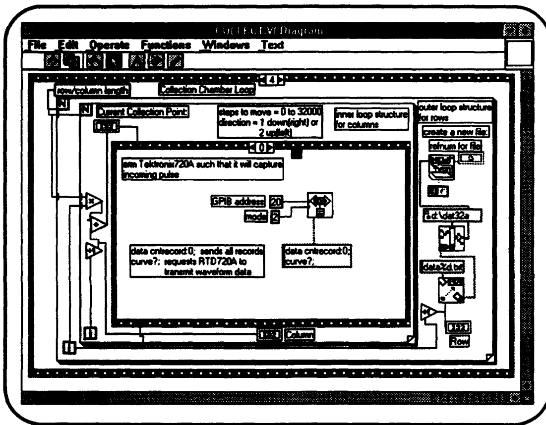
Figure 15. Block Diagram 40. Arming of the Tektronix RTD720A.
