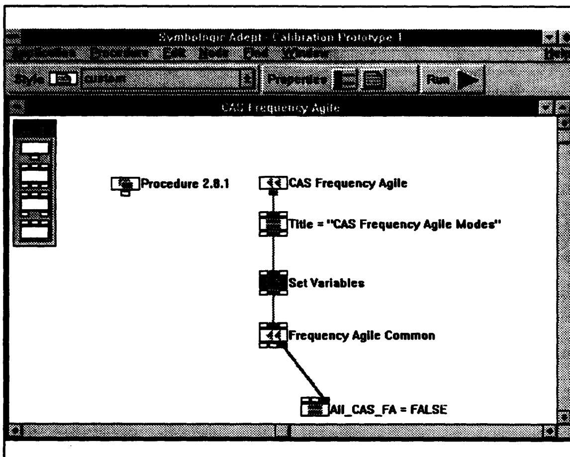
Figure 9 Adept Procedure Utilizing a Custom Node
