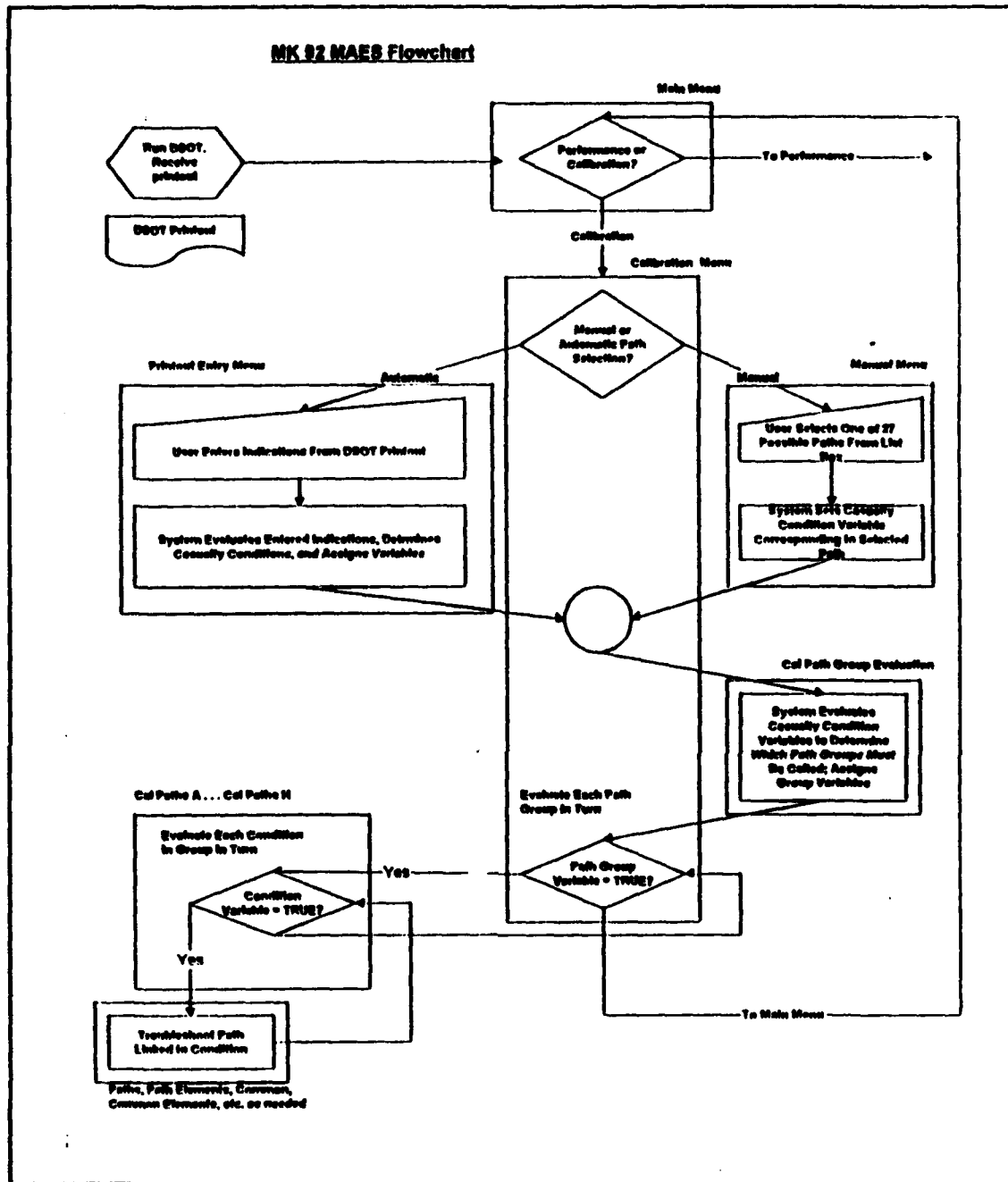
Figure 5 MK92 MAES Flowchart
