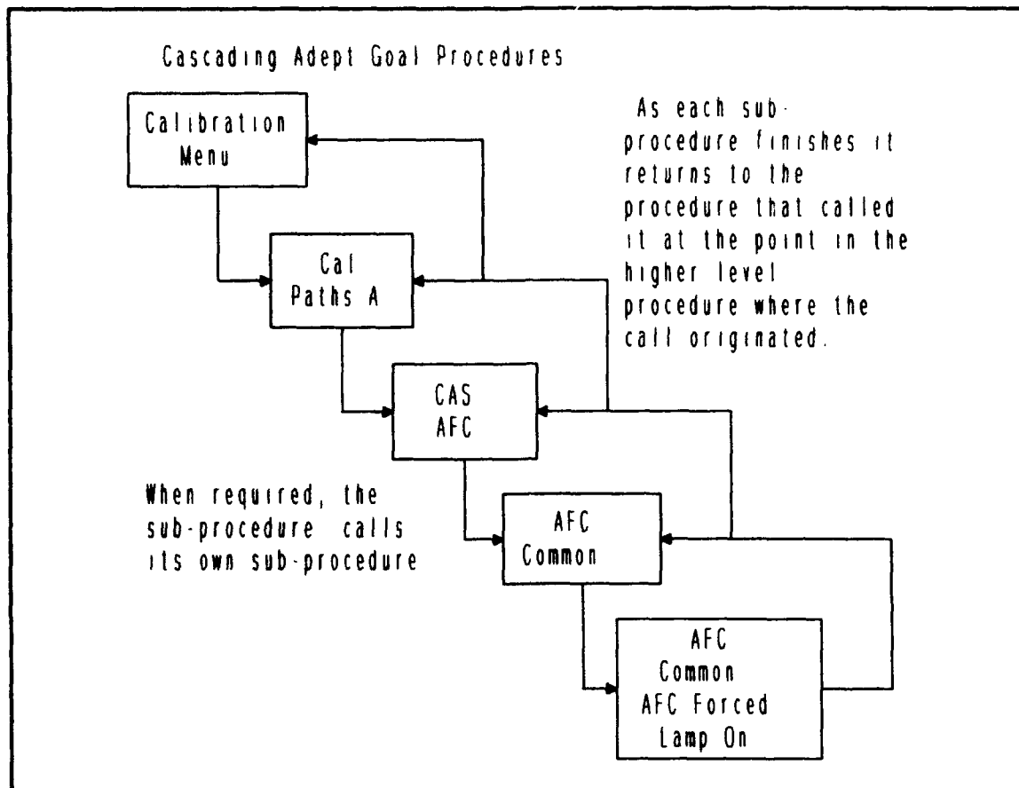
Figure 3 Cascading Adept Goal Procedures
