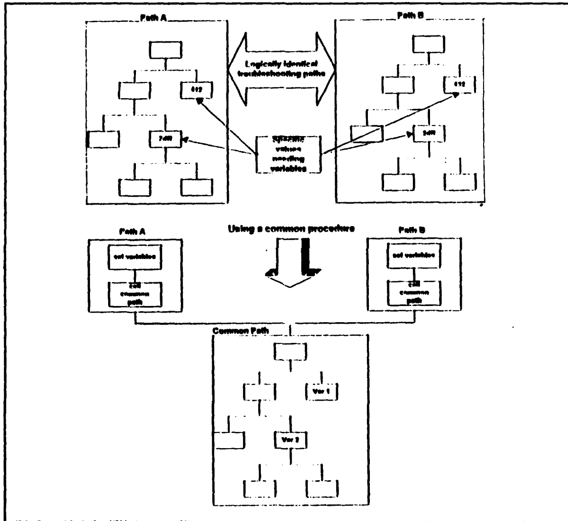
Figure 4 Genesis of a Common Procedure
