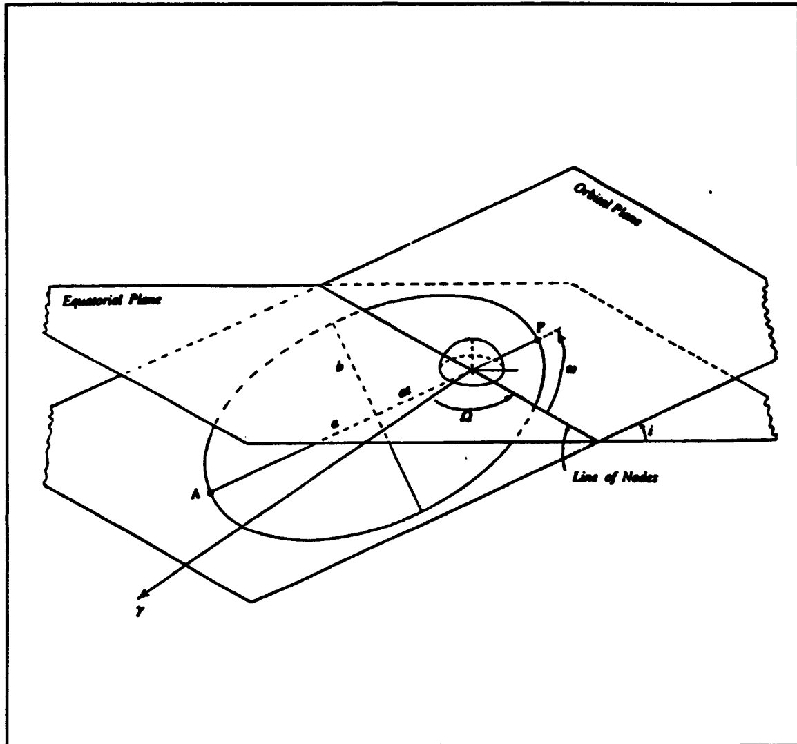
Figure 4. Orbital Elements [Ref. 7:p. 98]
