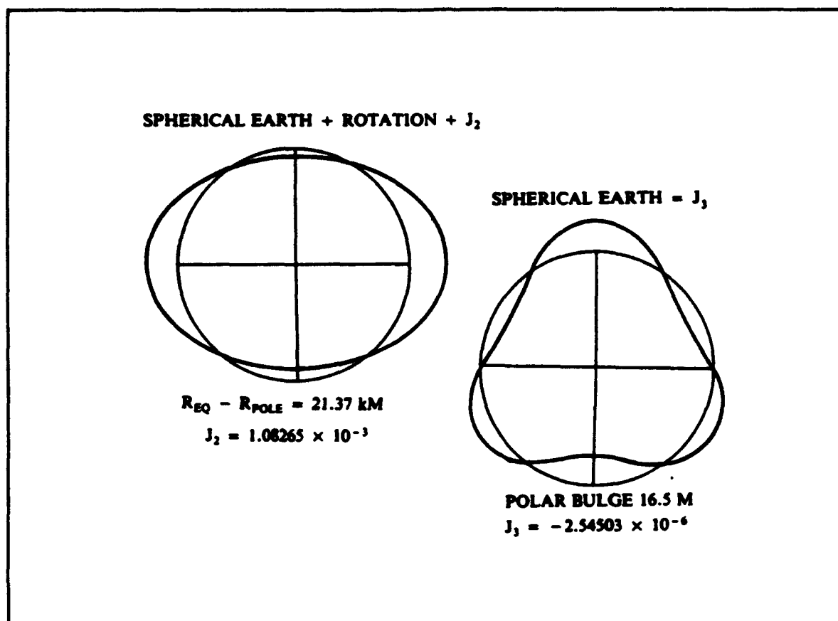
Figure 9. Earth's Zonal Harmonics [Ref. 12:p. 292]
