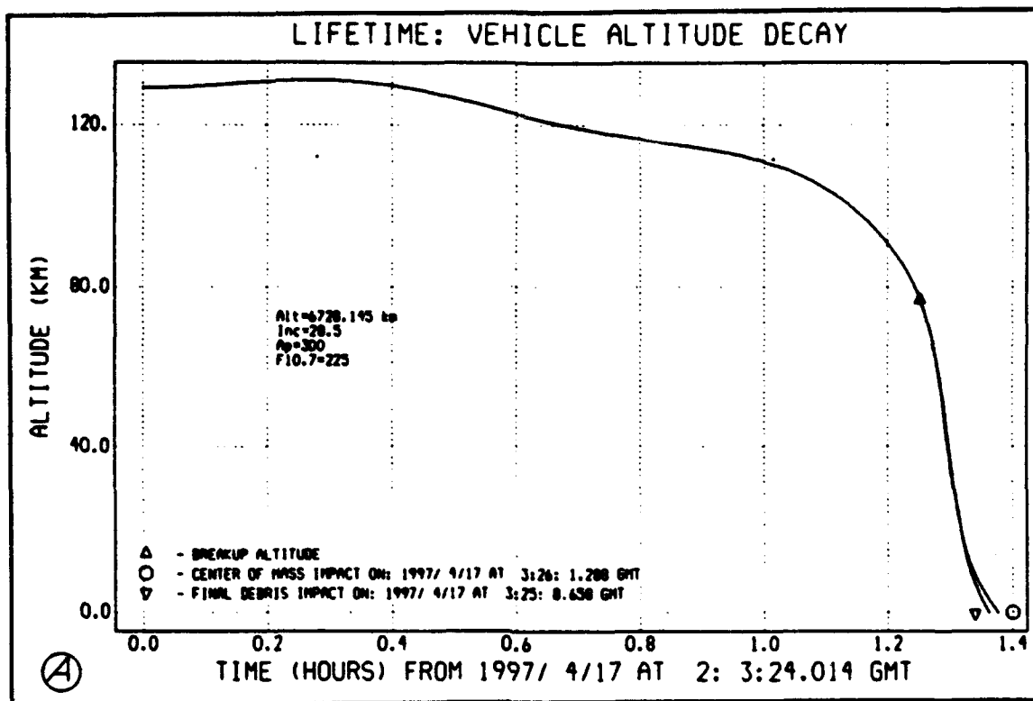
Figure 14. Vehicle Altitude Decay History
