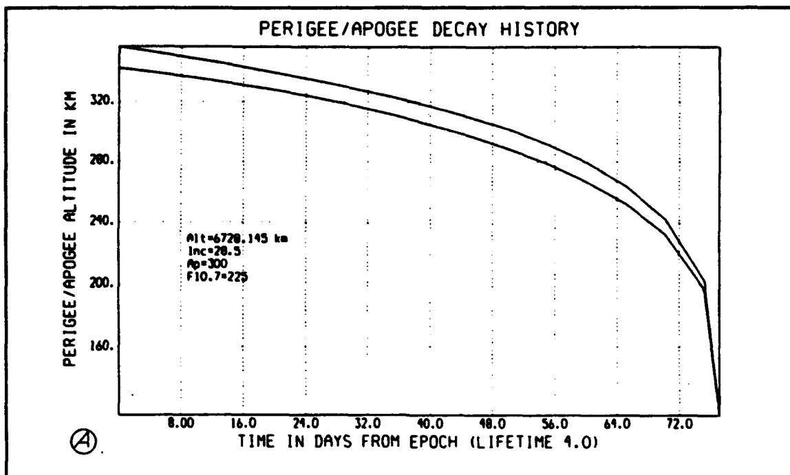
Figure 12. Plot of PANSAT Perigee/Apogee Decay History
