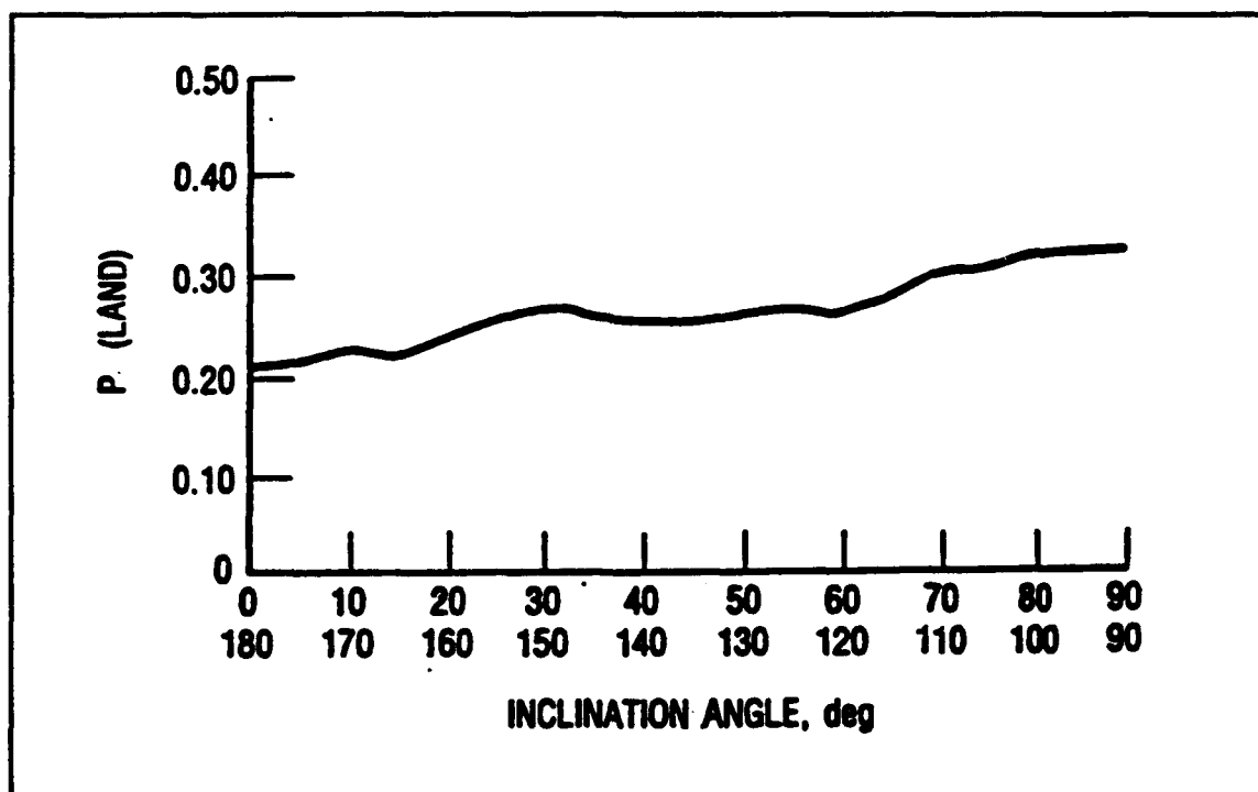
Figure 29. Probability of Land Impact vs. Inclination Angle [Ref. 19:p. B-3]
