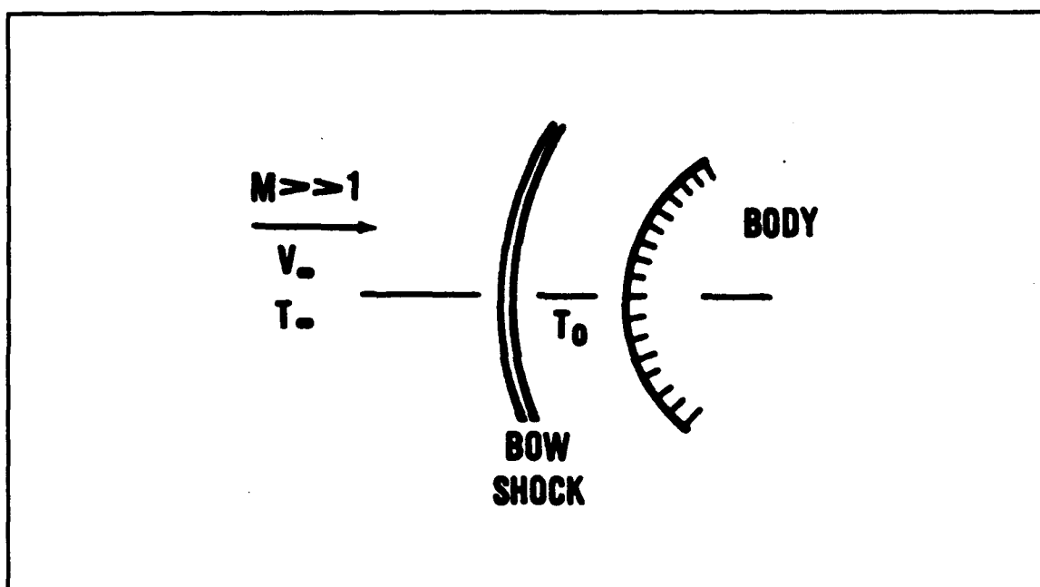
Figure 25. Shock wave and Stagnation Temperature on a Reentering Vehicle
