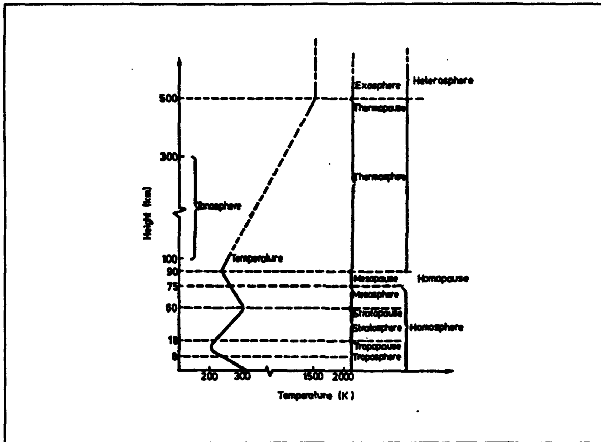
Figure 5. Structural Breakdown of Earth's Atmosphere [Ref. 9:p. 278]
