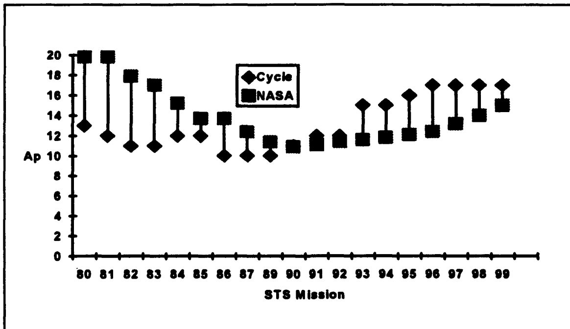
Figure 20. NASA Ap Values vs. Predicted Values
