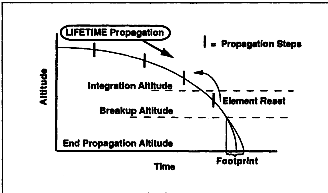
Figure 10. Illustration of Integration and Breakup Model [Ref. 15]
