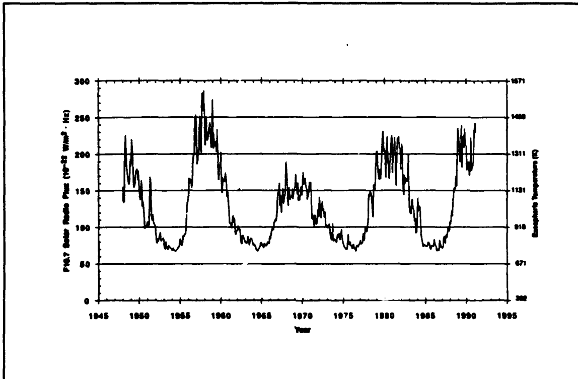
Figure 6. Observed Monthly Mean Radio Flux at 10.7 cm [Ref. 8:p. 209].
