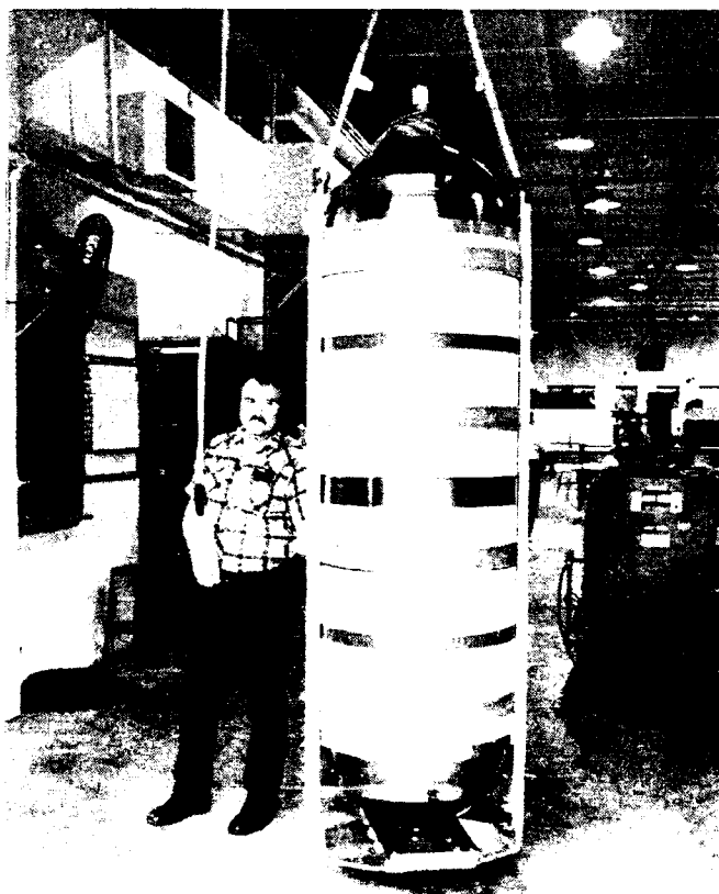
Figure 74. 26-inch-housing cylindrical hull mounted inside the pressure-test fixture.
