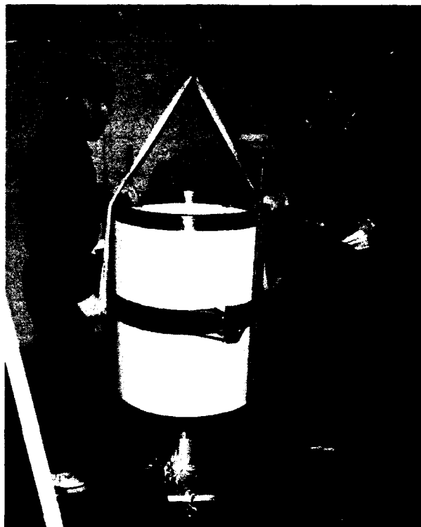
Figure 33. Epoxy bonding of central stiffening joint ring to first cylinder bay.
