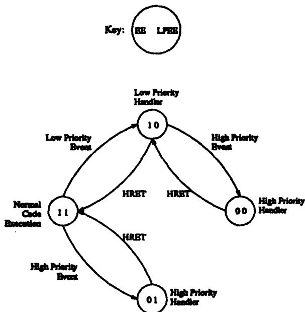
Figure 16: Event State Transition Diagram
