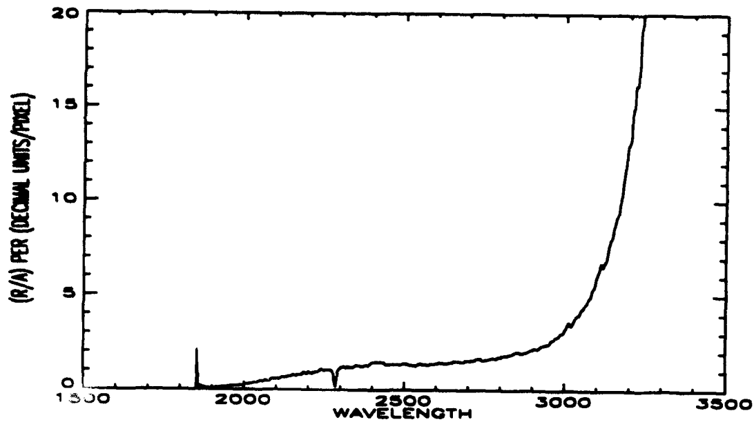
Figure 20: FER-IR sensitivity curve.
