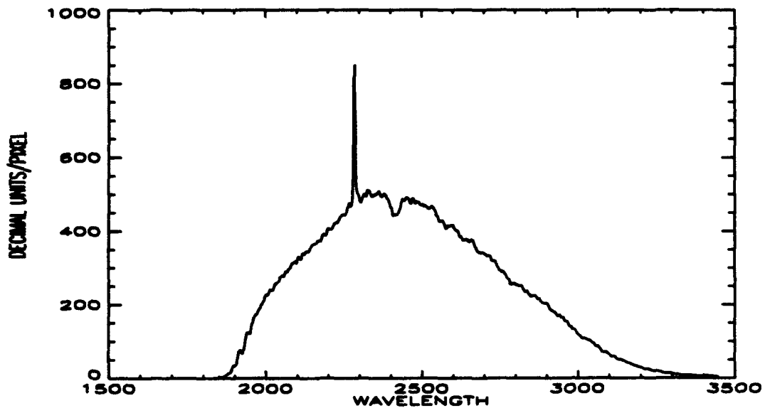
Figure 16: MUSTANG output for Deuterium lamp.
