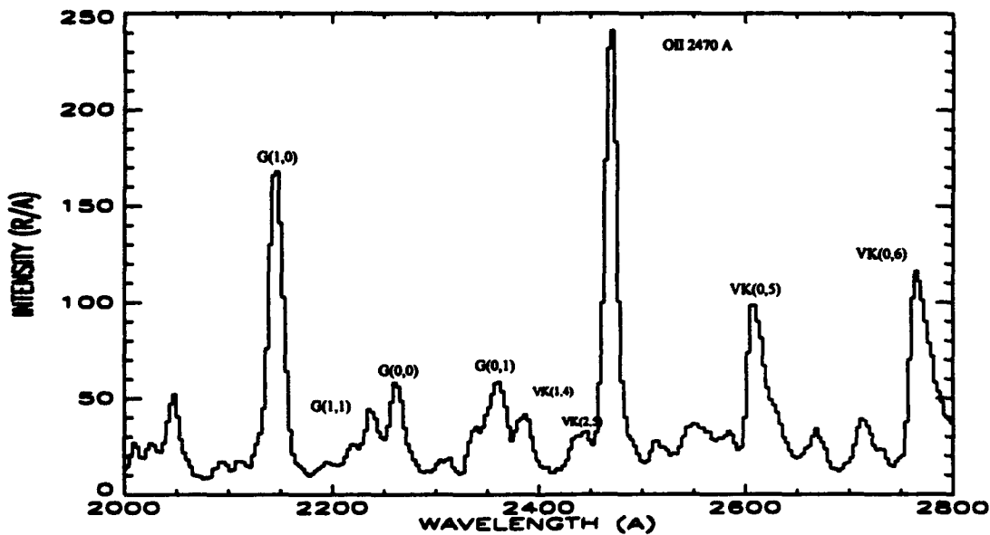
Figure 24: Representative spectrum taken at 180 km.
