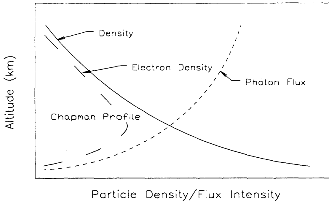
Figure 2: Electron production curve.
