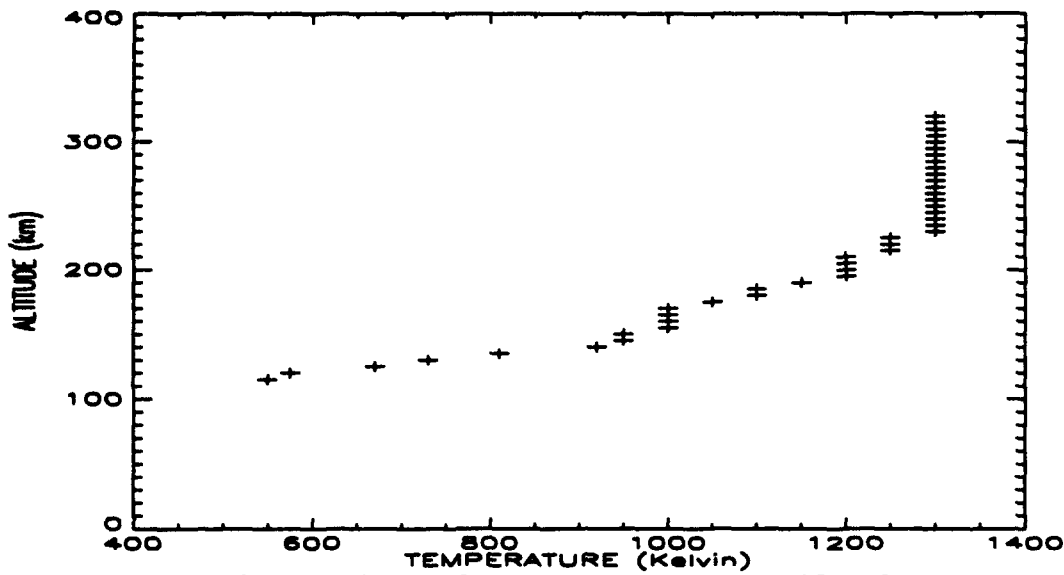
Figure 27: The estimated temperature profile for the downleg.
