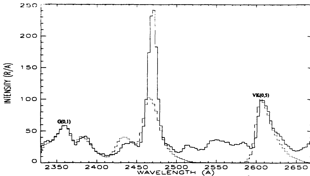
Figure 29: Estimating contribution to 2470 Å feature by NO \gamma and N 2 VK emissions. The solid line is the observed intensity, the dashed line is the sum of NO \gamma and N 2 VK.
