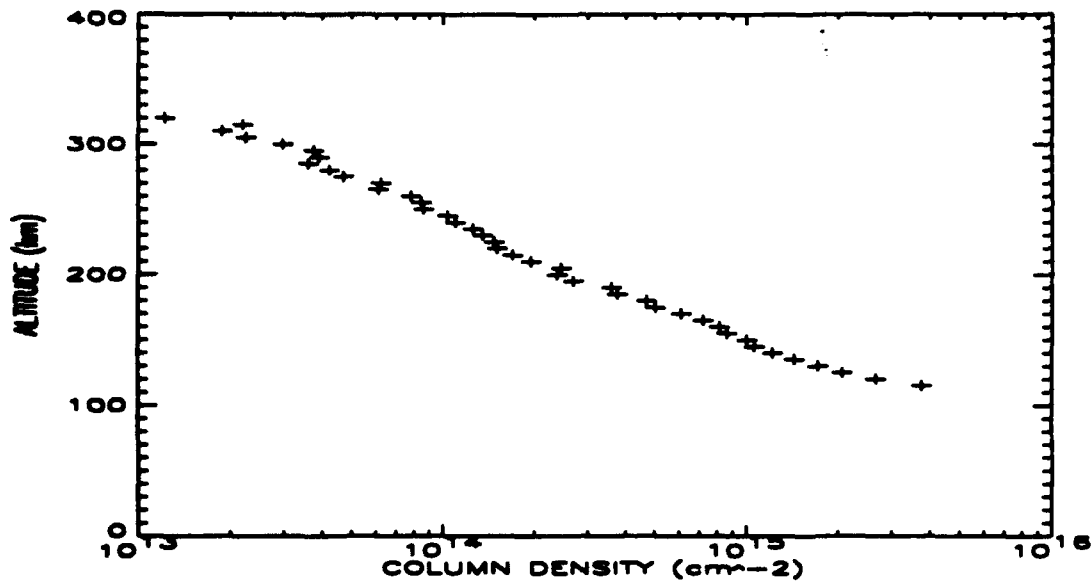
Figure 31: Estimated nitric oxide column density.
