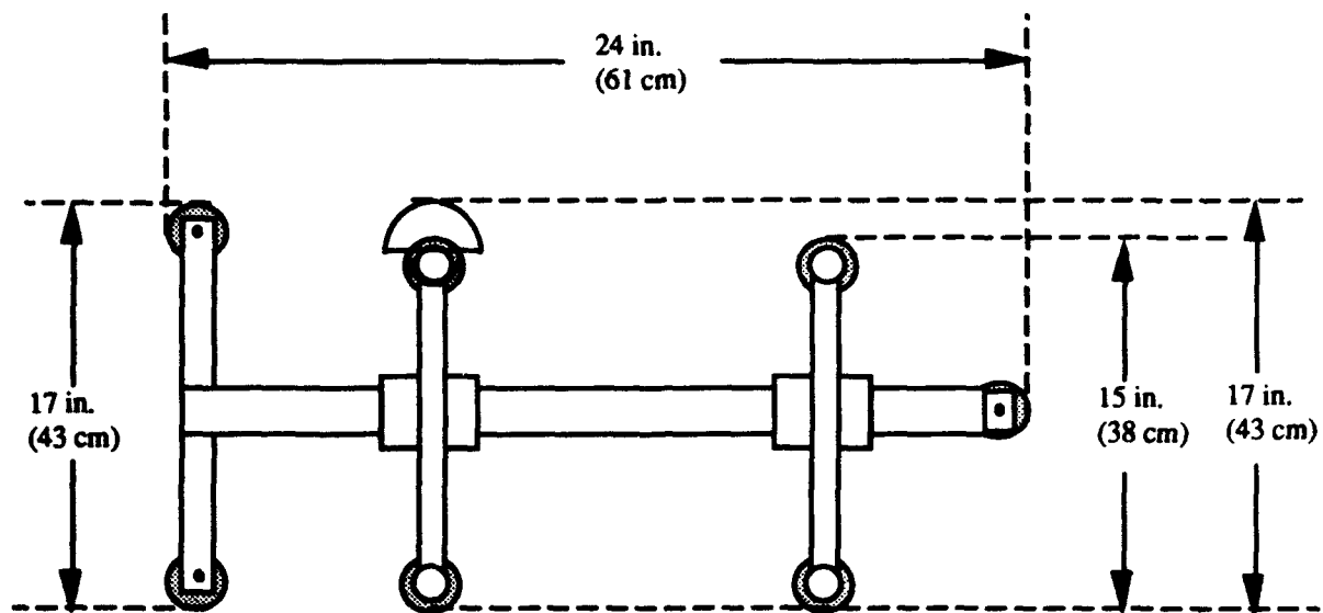
FIGURE 4. ROBOT DIMENSIONS (OVERHEAD VIEW)
