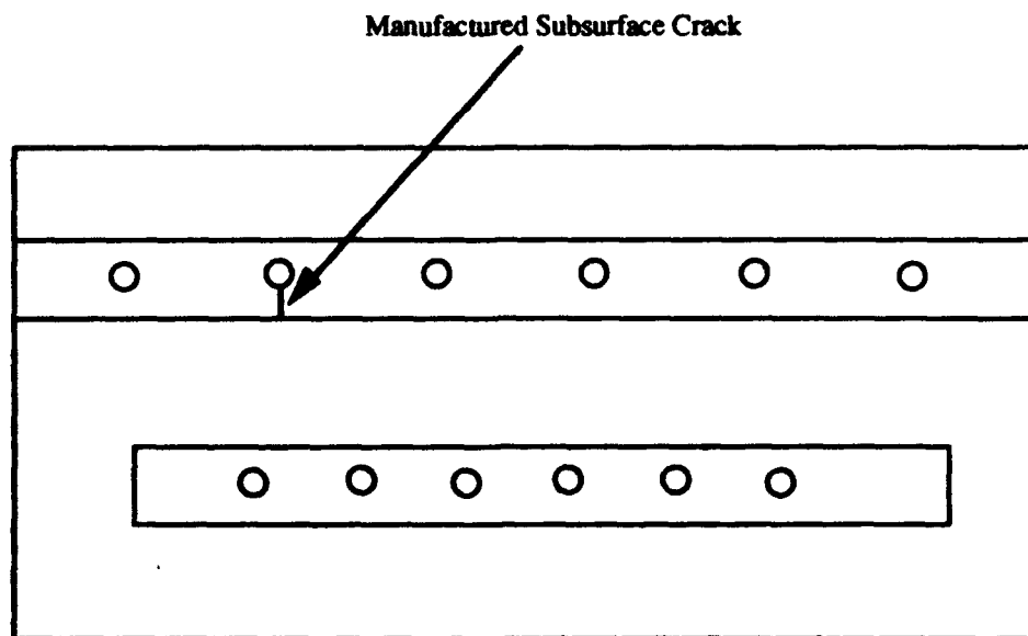
FIGURE 34. CALIBRATION STANDARD (BACK)
