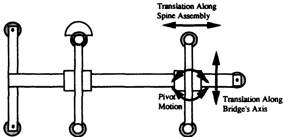
FIGURE 8. STABILIZER BRIDGE MOTIONS
