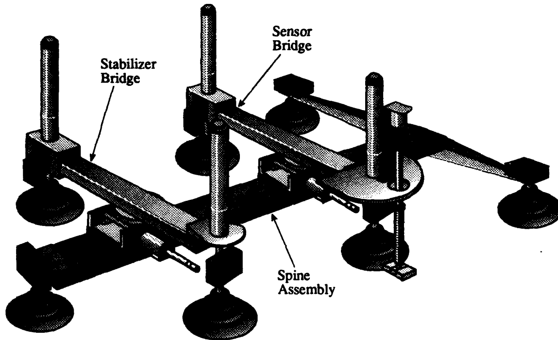
FIGURE 3. DRAWING OF THE CRUCIFORM ROBOT
