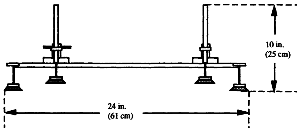
FIGURE 5. ROBOT DIMENSIONS (SIDE VIEW)
