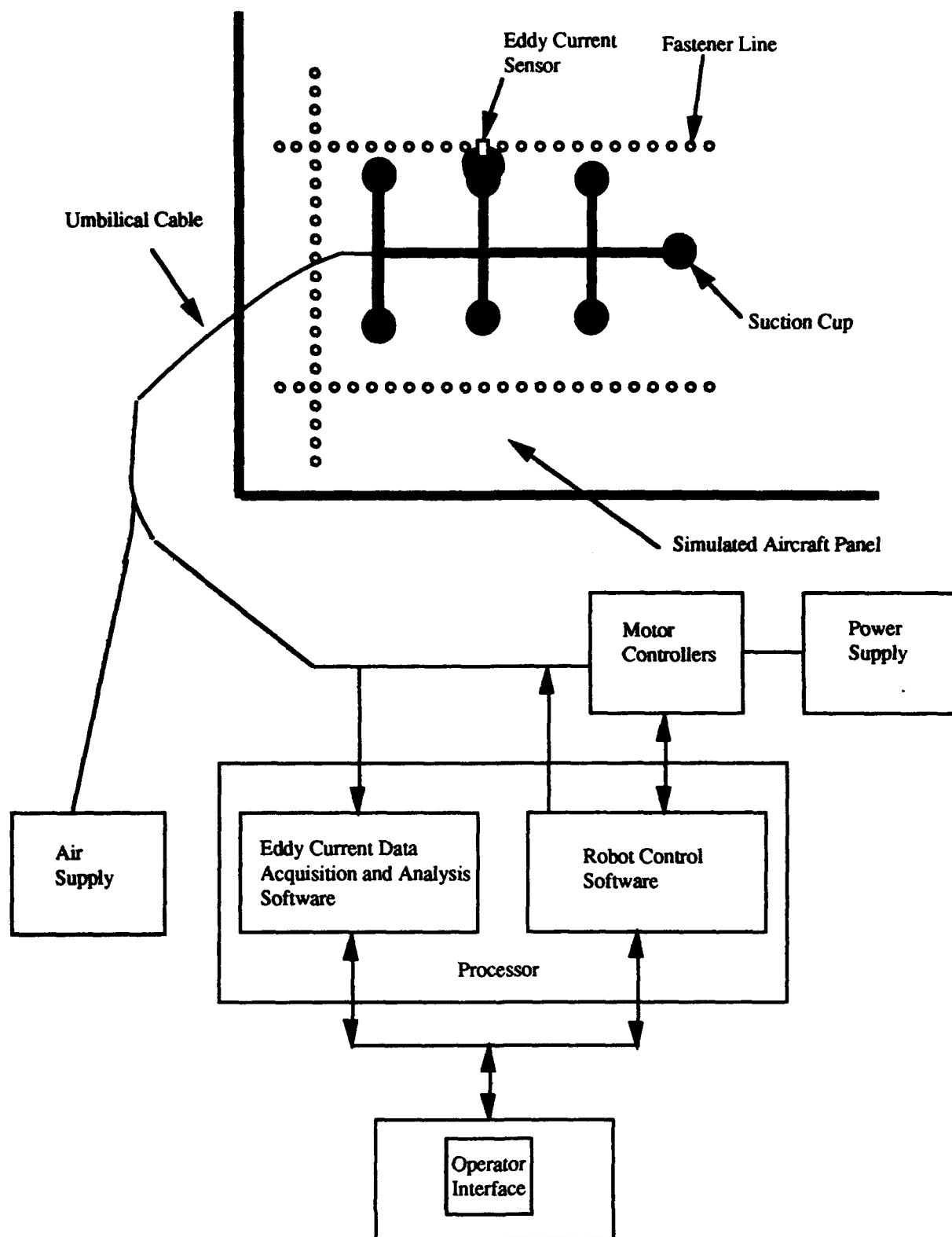
FIGURE 1. PROTOTYPE ROBOTIC SYSTEM
