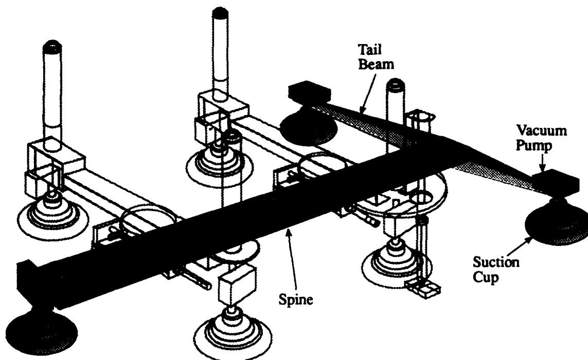
FIGURE 12. DRAWING OF THE SPINE ASSEMBLY
