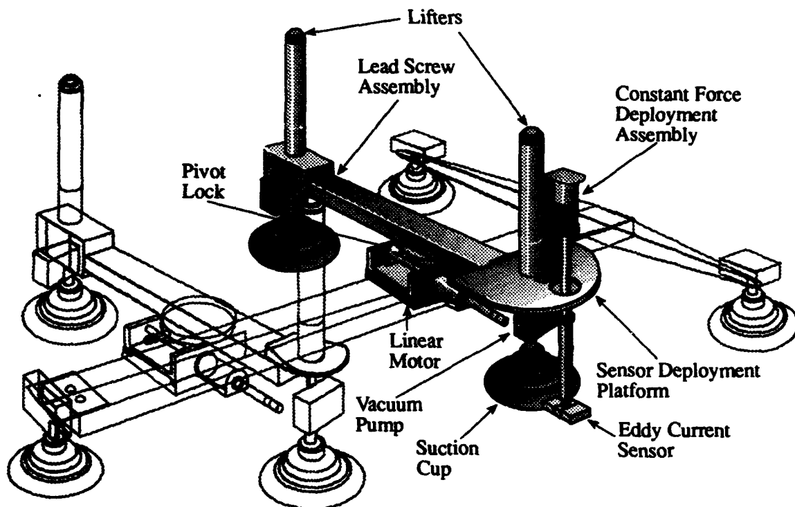
FIGURE 11. DRAWING OF THE SENSOR BRIDGE
