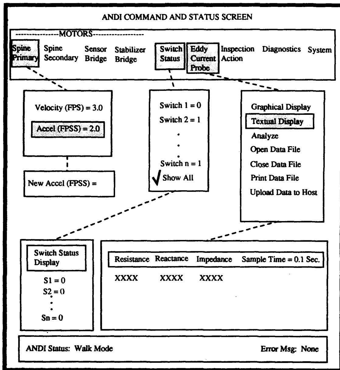
FIGURE 40. OPERATOR INTERFACE
