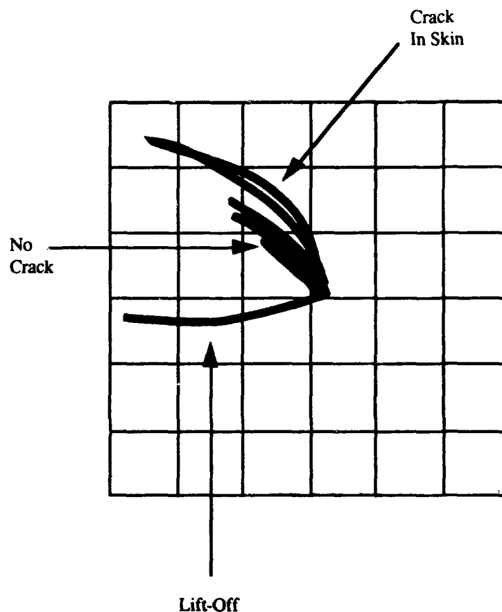
FIGURE 36. EDDY CURRENT INSTRUMENT DISPLAY FOR SURFACE CRACK
