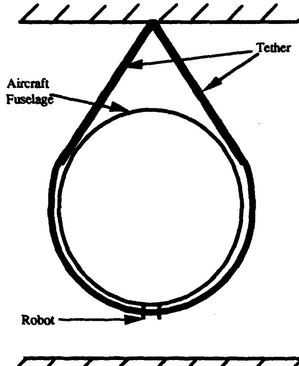
FIGURE 30. SPECIAL-CASE TETHER
