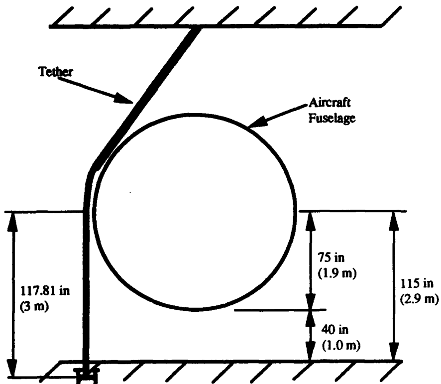
FIGURE 29. TETHER LIMITATION
