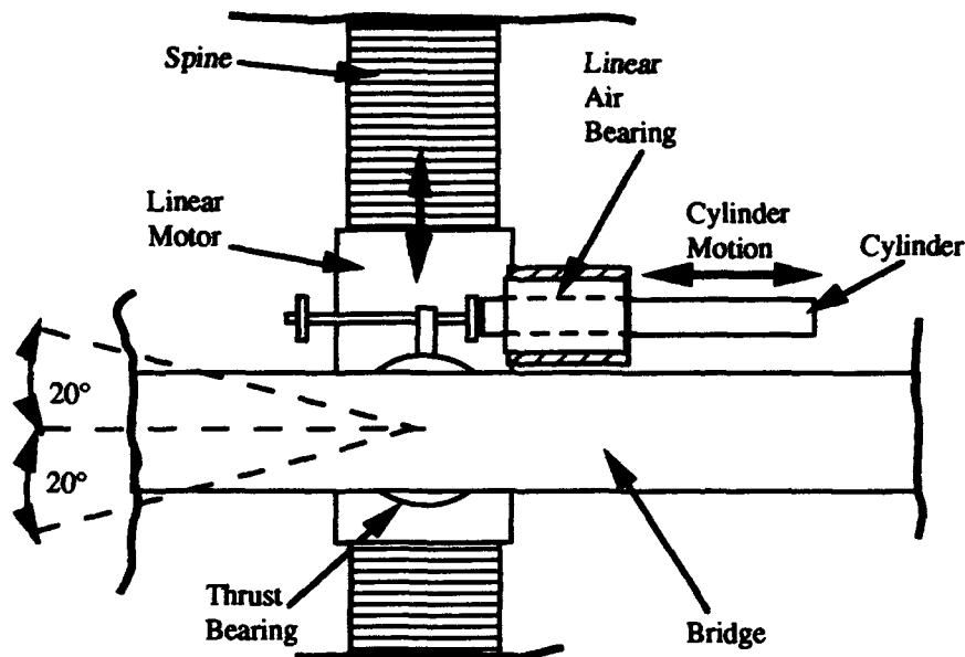
FIGURE 9. PIVOT LOCK SCHEMATIC (UNLOCKED)
