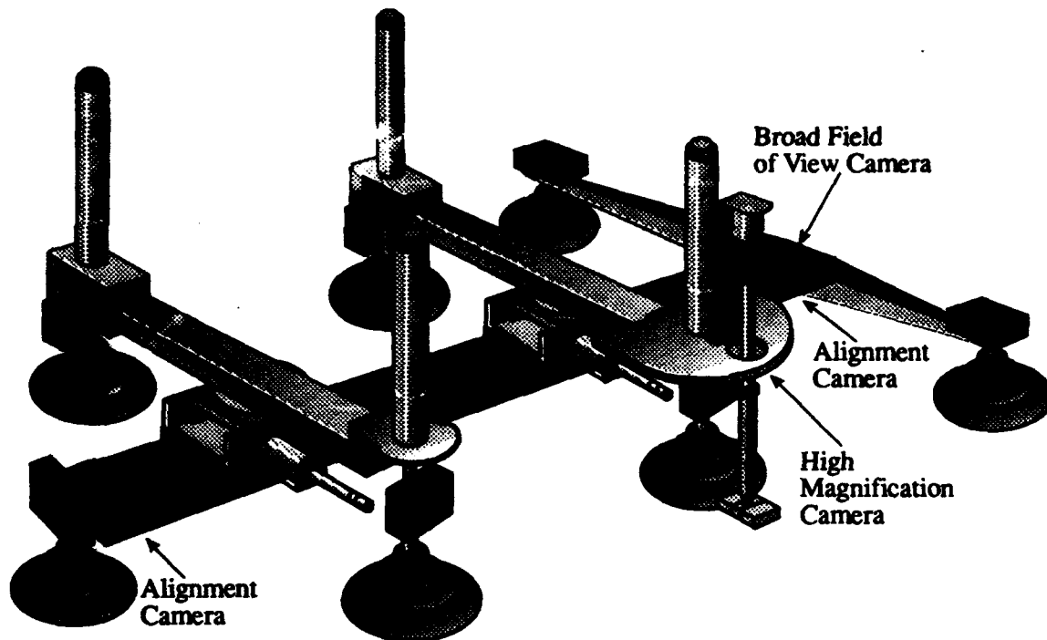
FIGURE 32. CAMERA PLACEMENT
