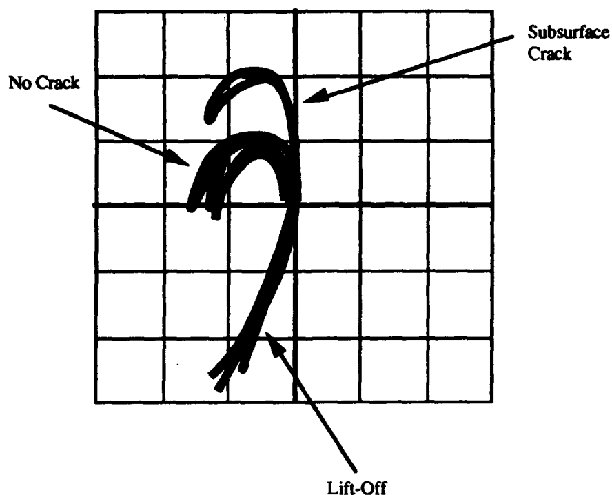
FIGURE 35. EDDY CURRENT INSTRUMENT DISPLAY FOR SUBSURFACE CRACK
