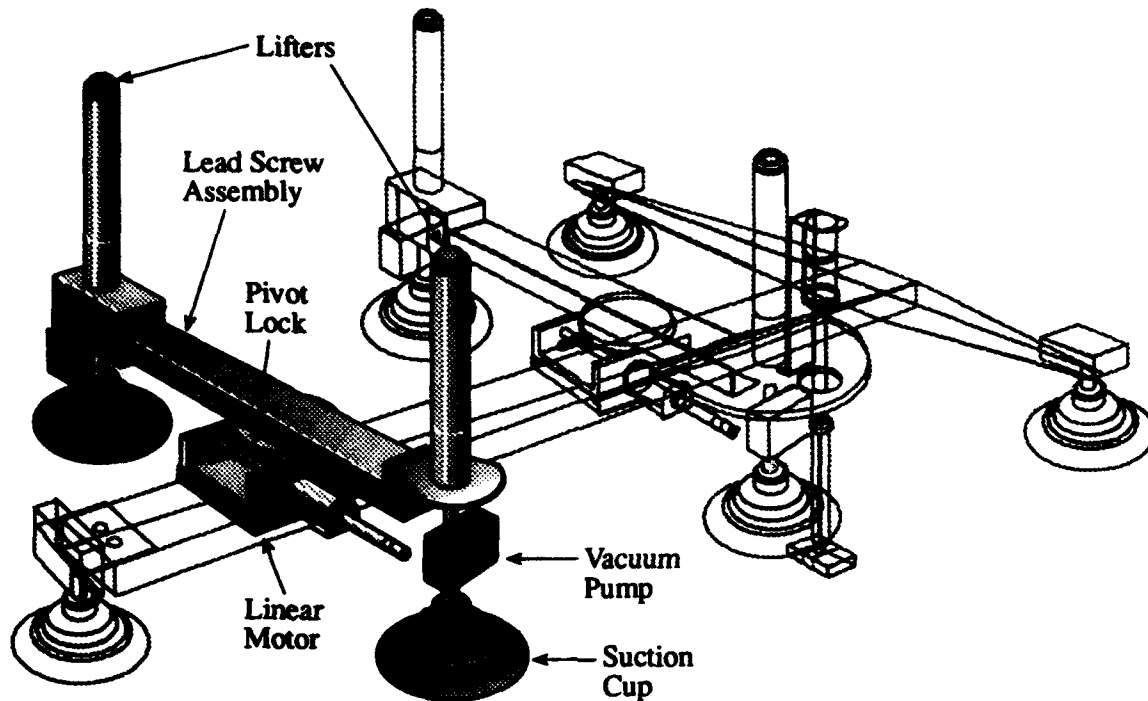
FIGURE 7. DRAWING OF THE STABILIZER BRIDGE
