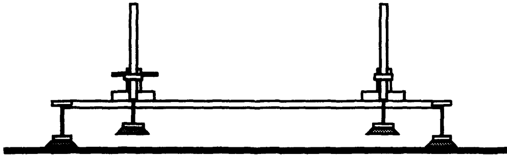
FIGURE 16. UNALIGNED ROBOT (SIDE VIEW)
