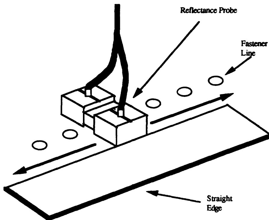
FIGURE 31. REFLECTANCE EDDY CURRENT SENSOR
