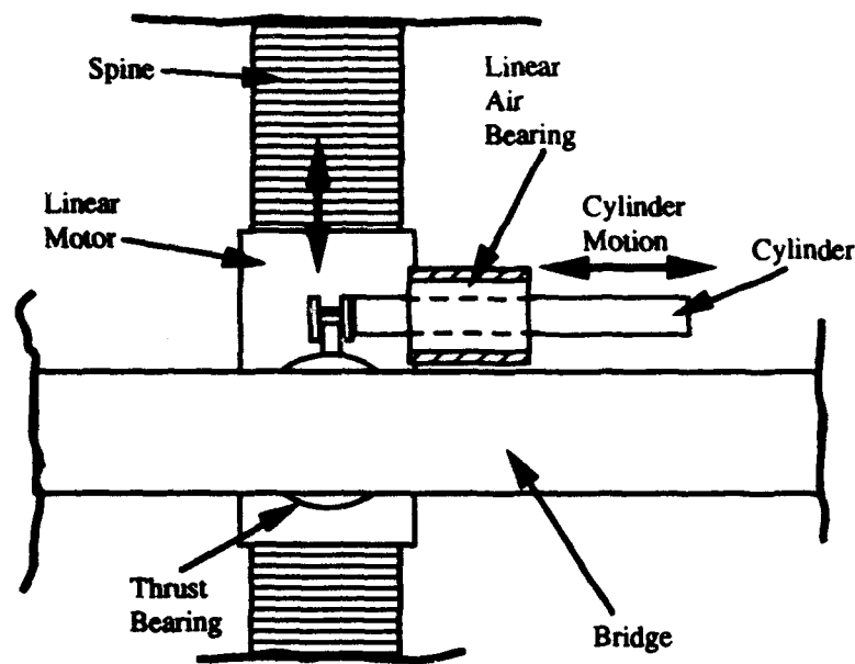
FIGURE 10. PIVOT LOCK SCHEMATIC (LOCKED)
