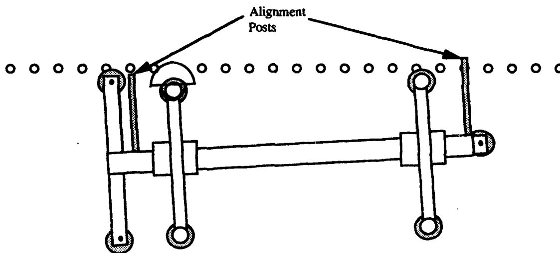
FIGURE 15. UNALIGNED ROBOT (OVERHEAD VIEW)
