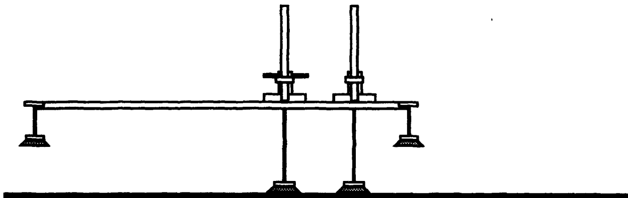
FIGURE 24. WALKING MOTION: SPINE ASSEMBLY RAISED
