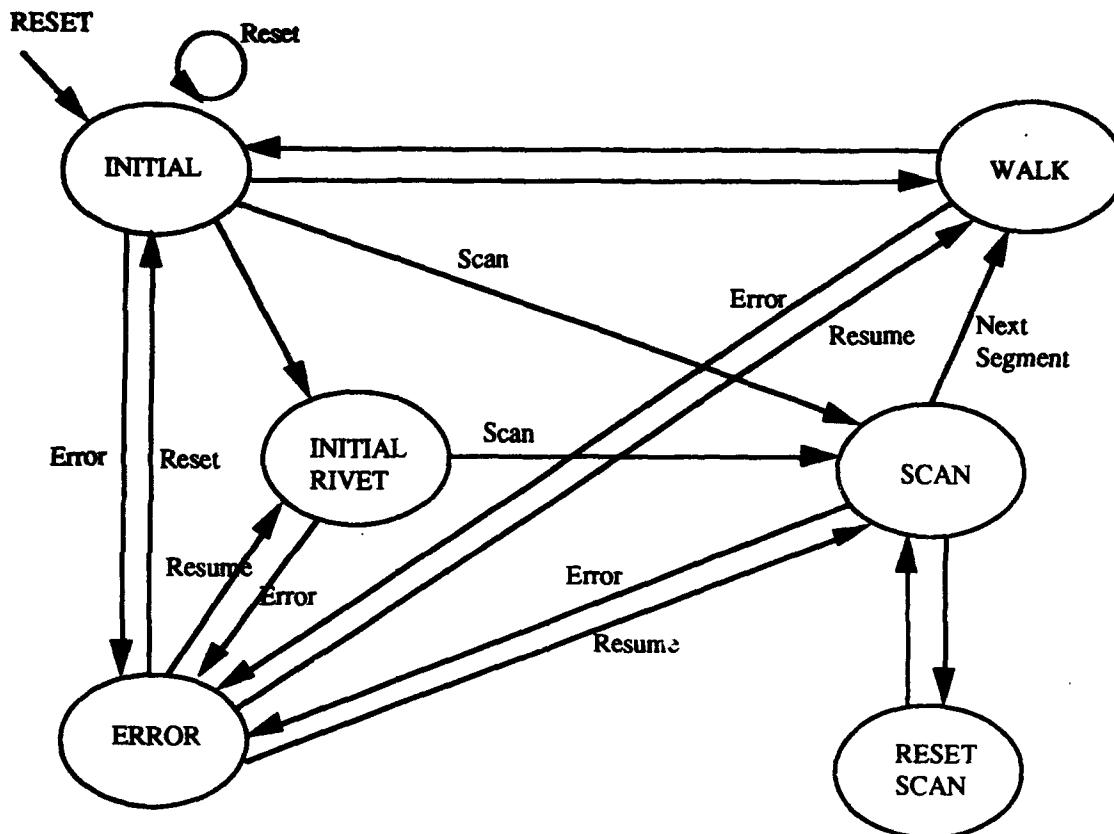
FIGURE 37. ROBOT STATES
