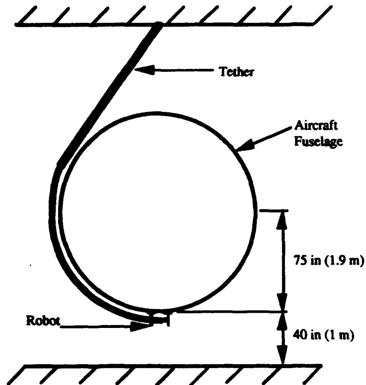
FIGURE 28. ROBOT TETHERED TO BOTTOM OF AIRCRAFT;
