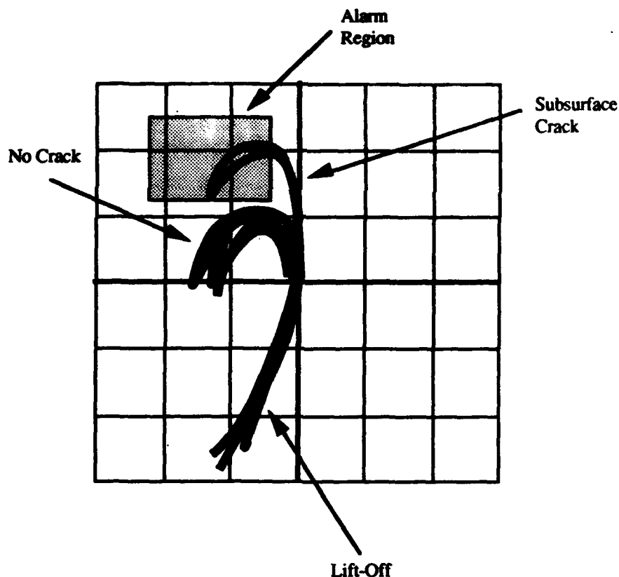
FIGURE 41. ALARM REGION ON AN IMPEDANCE-PLANE DISPLAY
