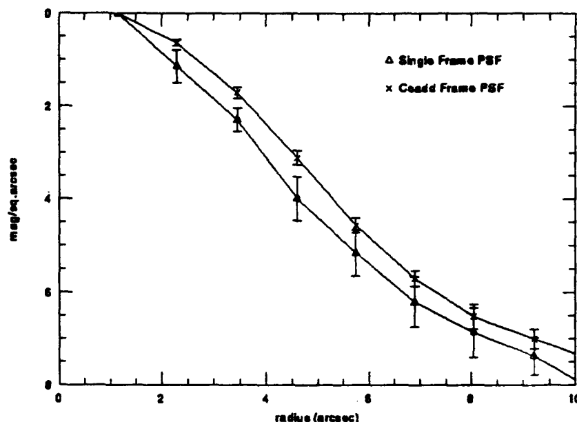
Fig. 2. The point spread function in the combination of 5 frames and the PSF extracted from the individual frames. The average PSF is much more stable than the undersampled data in any one frame and leads to accurate photometry. The average PSF is broadened in the prototype camera due to variations of the PSF across the focal plane.
