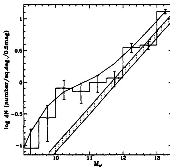
Fig. 5. The surface density of galaxies in the ( l = 135^\circ , b = -25^\circ ) field (histogram) compared with surface densities of field galaxies from Broadhurst et al. 1992 (shaded line). The large excess of galaxies at K_r < 11 mag. appears to be caused by the large number of galaxies concentrated at z \sim 0.017 . A model of field counts plus supercluster members (solid line) is described in the text.
