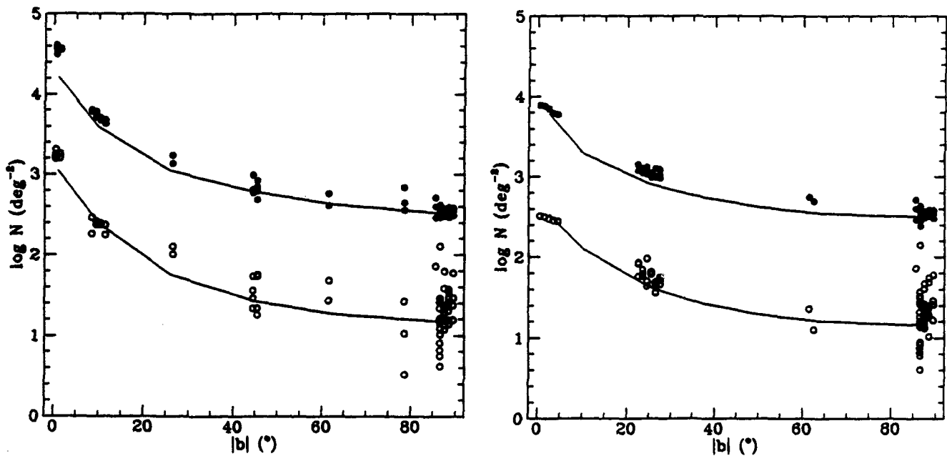
Fig. 3. Left: Surface density of stars brighter than K_s=14 mag. (filled symbols) and stars brighter than K_s=10 mag. (open symbols), for a narrow range of galactic longitude near l=53^\circ . Right: Same as the figure on the left for l=130^\circ . The solid curve corresponds to a simple exponential disk model incorporating reddening.
