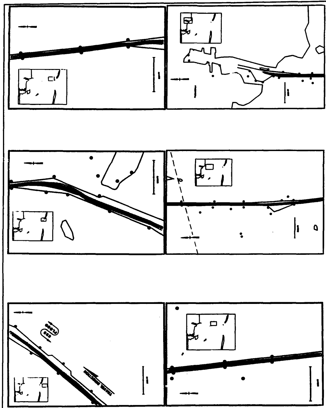
Figure 12. Inbound composite pilot tracklines 450/250 channel, LASH ship (694x100x36), maximum cross current, 15 knot easterly wind
