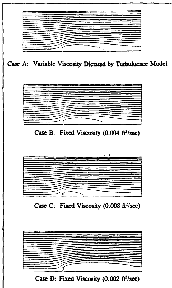
Figure 1. Flow past a dike (streamlines)
