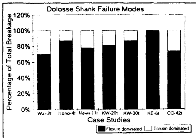
Figure 2. Dolos failure modes
