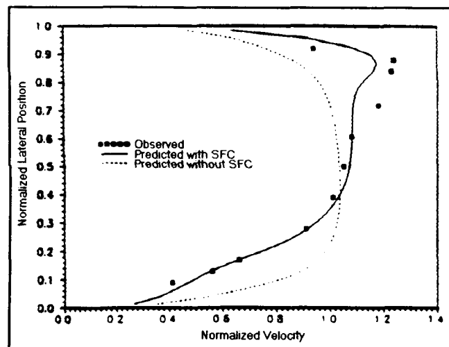
Figure 3. Observed and predicted normalized velocity distribution downstream of a 90-deg bendway
