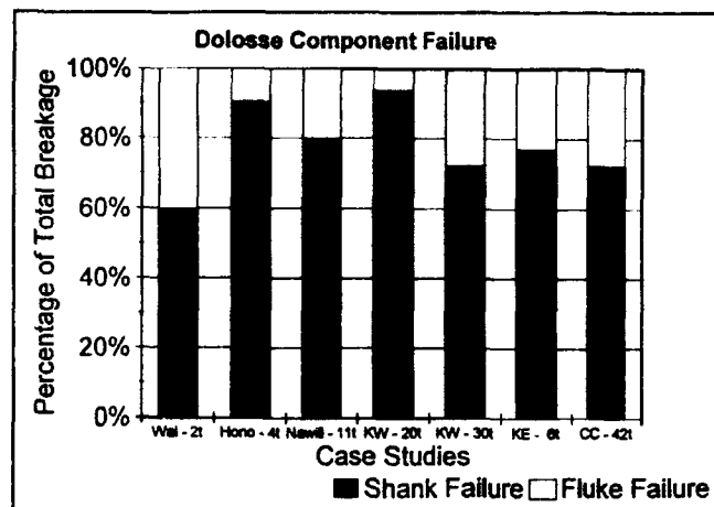
Figure 3. Dolos component failure
