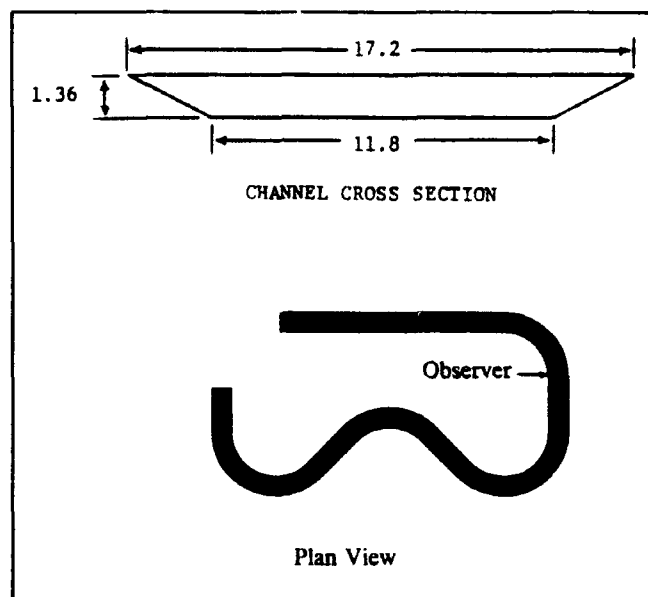
Figure 2. Riprap test facility
