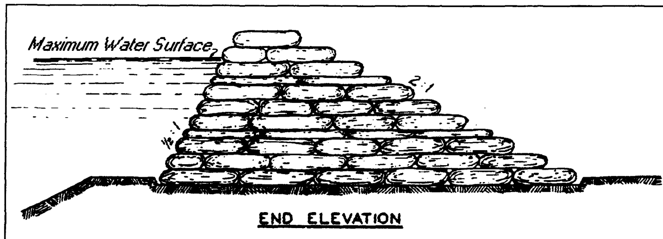
Figure 1. Properly stacked sandbags
