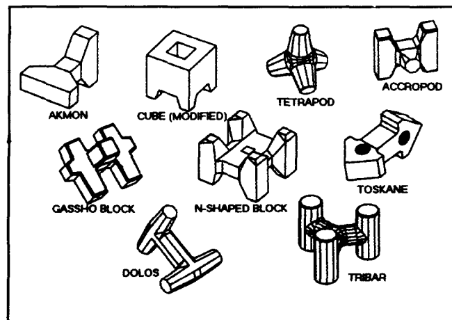
Figure 1. Various concrete armor unit shapes
