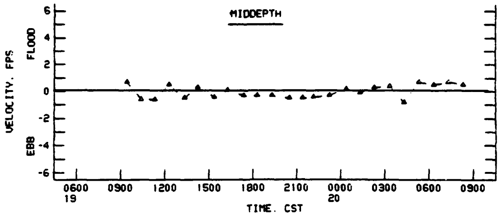
VELOCITIES AT STATION R4.0C SURFACE, ONE-QUARTER DEPTH, AND MIDDEPTH
