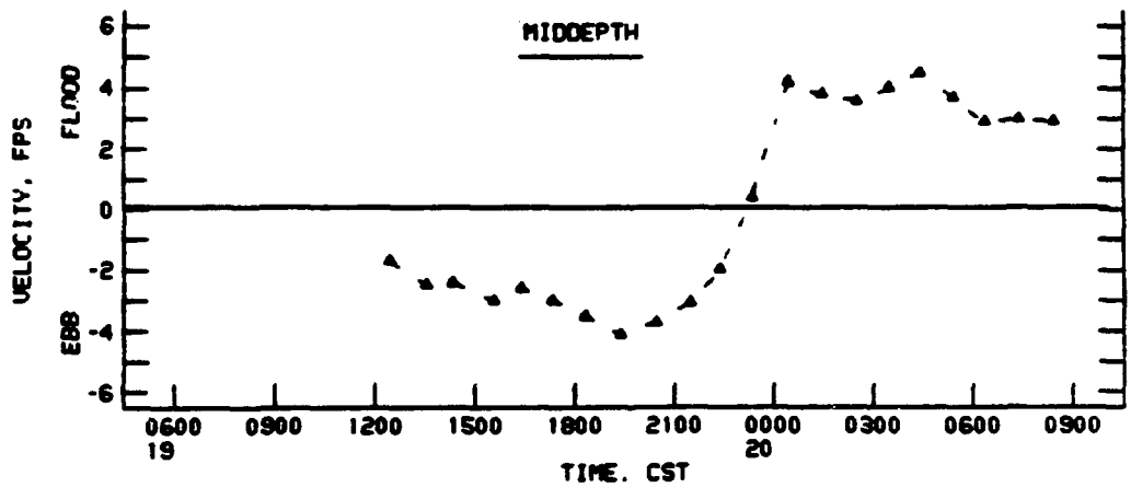
VELOCITIES AT STATION R1.0C SURFACE, ONE-QUARTER DEPTH, AND MIDDEPTH 19-20 JULY 1990
