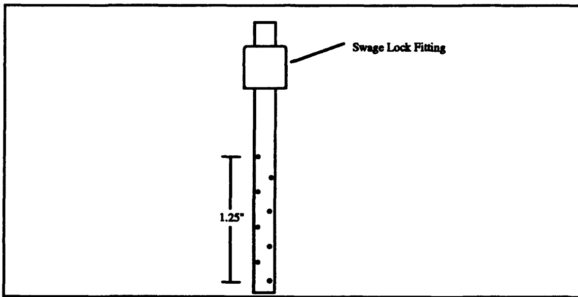
Figure II-7 Fuel-tube Atomizer
