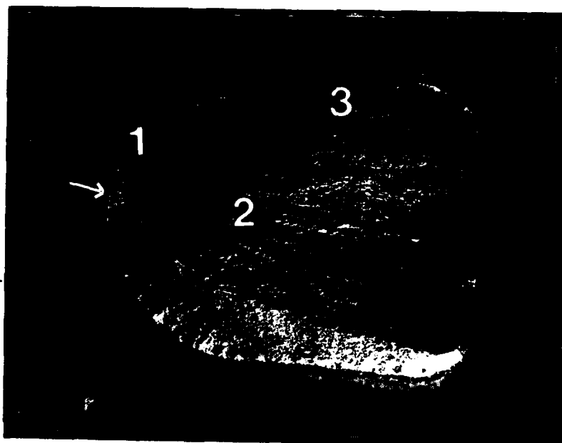
Figure 6 Macrograph of representative fracture half of a failed lug. 7.5X
