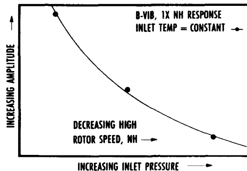
Fig. 4. Effects of inlet pressure on bearing maximum vibratory response.
