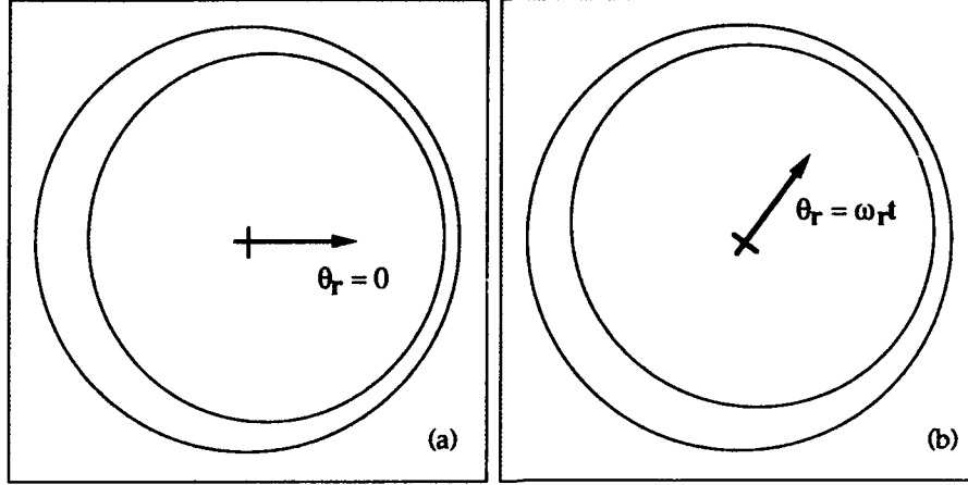
Figure 5. Depiction of air gap eccentricity.
