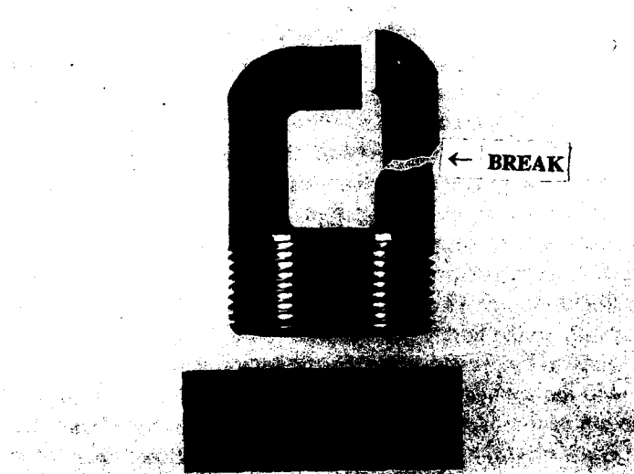
Figure 2 The second failed suspension lug shown in the as-received condition. Reduced 30%
