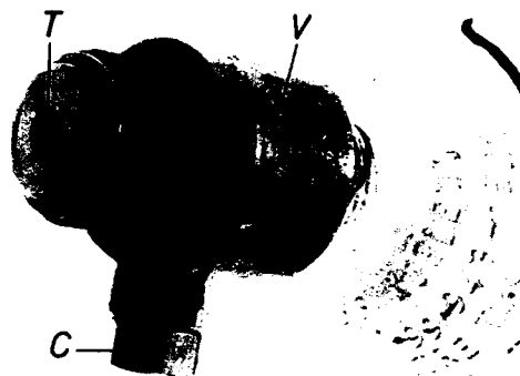
Figure 2 1.3:1 Valve body (V) with adjusted tap- pet washer inset (T), thread cap (C) and drilled hole
