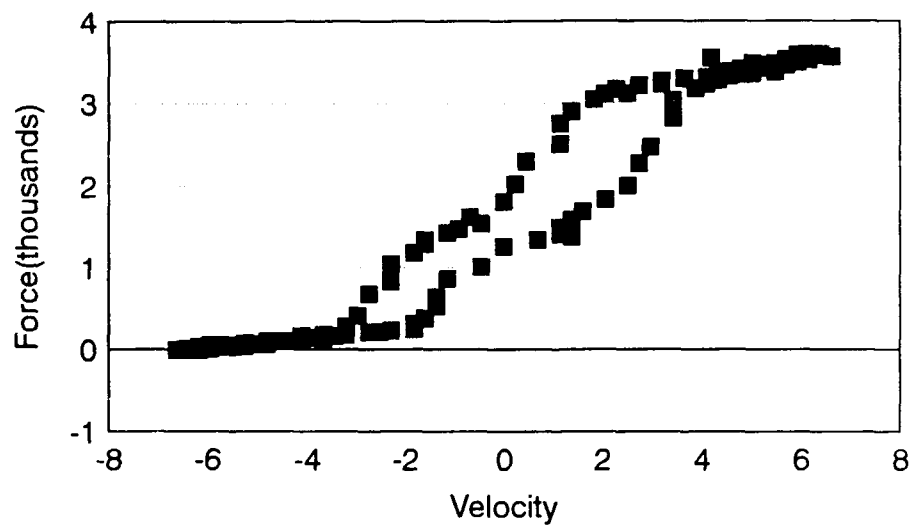
Figure 2. Force vs. Velocity Plot of Shock Absorber Data
