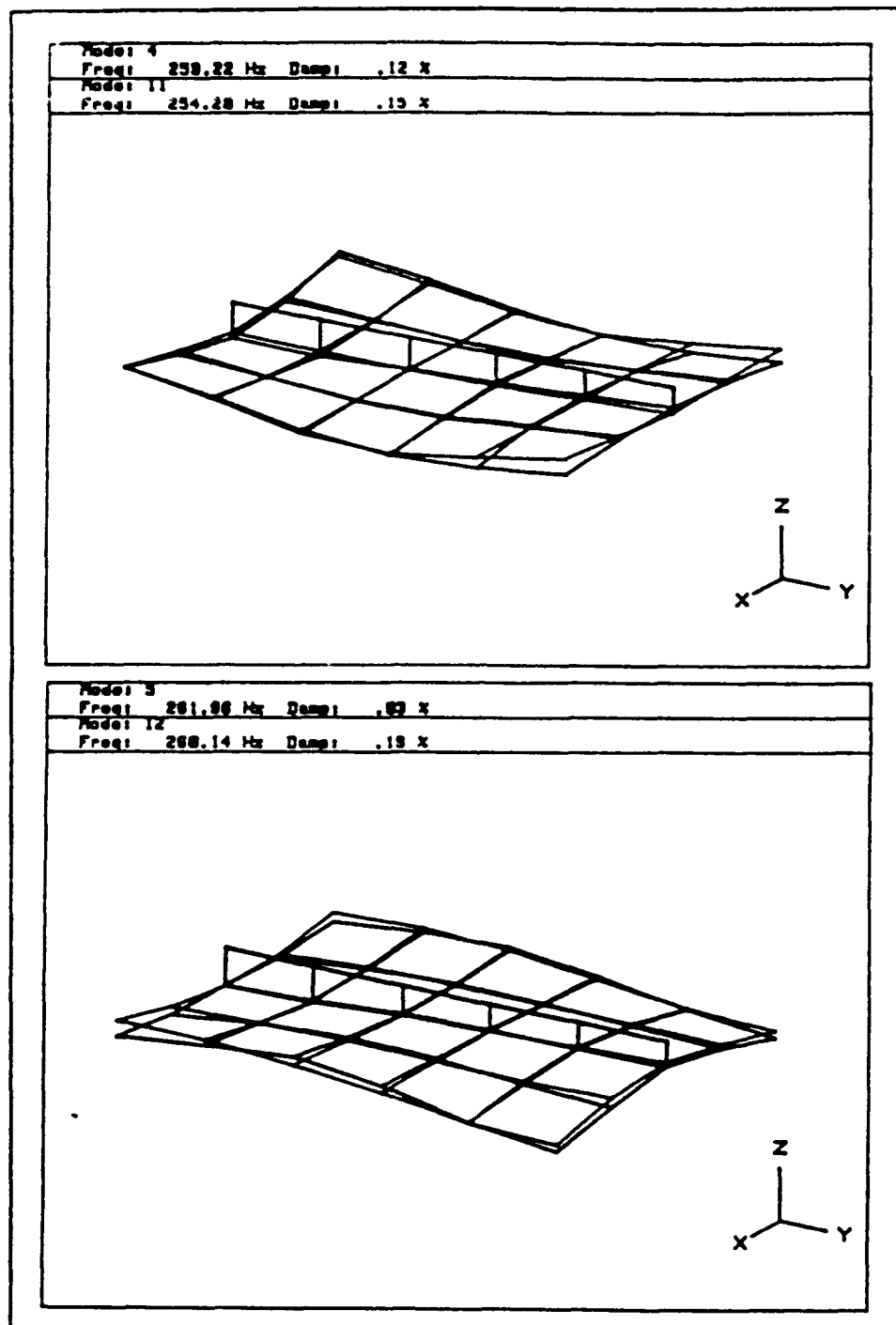
Figure 5. Mode Shapes of Modes 4 & 5 Before and After Center Bolt Removal.
