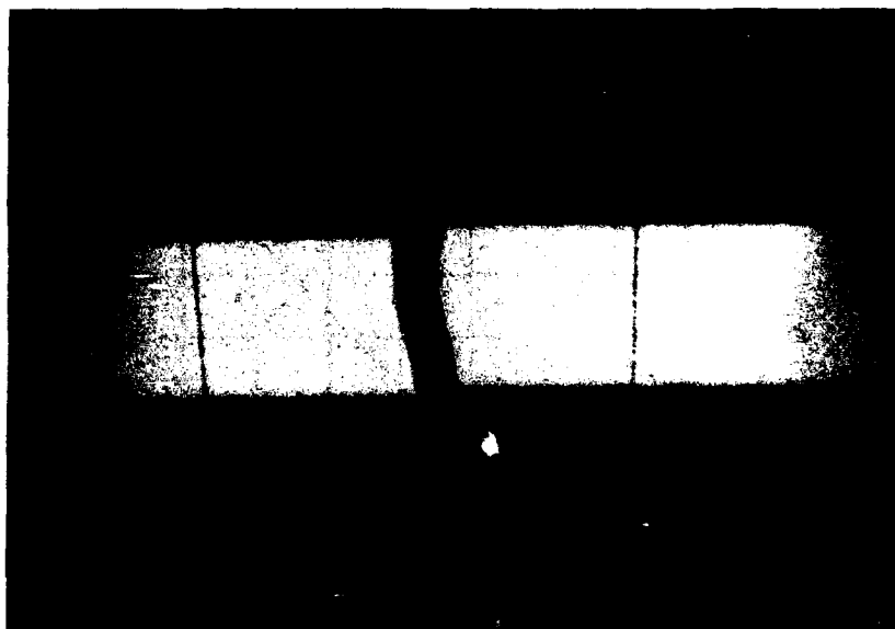
FIGURE 6. CRACK PROGRESS IN FLEXURE FOR 20 LBS/FT 3 RIGID POLYURETHANE FOAM.
