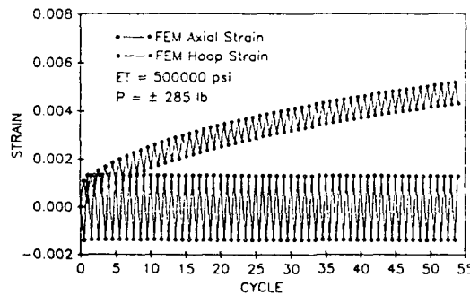
Fig. 8 Elastic-plastic finite element analysis of ratcheting with an internal pressure of 3,000 psi and the geometry of Figure 4.
