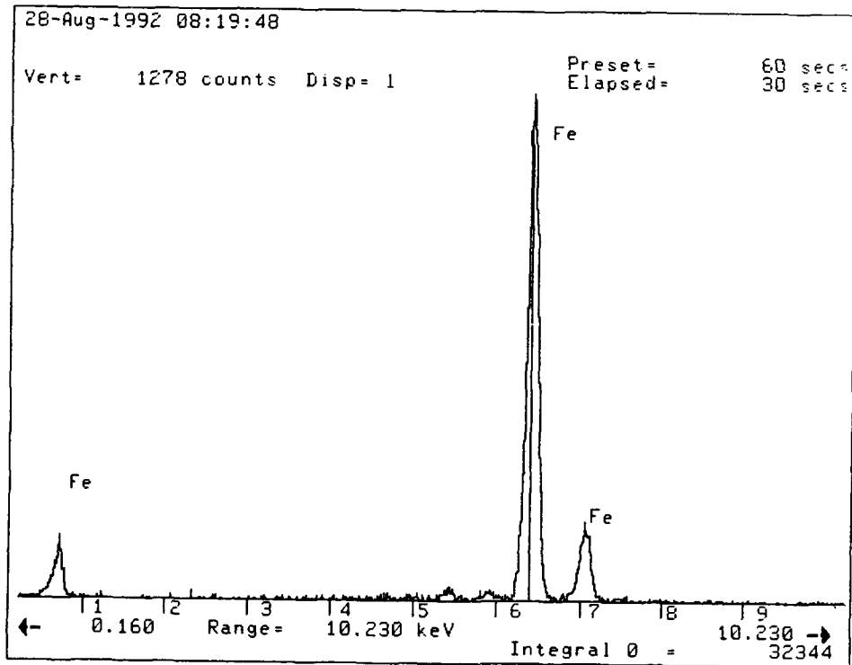
Figure 5 Representative EDS spectrum obtained from an area of the fracture surface away from the crack initiation sites.
