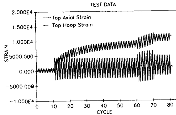
Fig. 6 Specimen 3, Carbon Steel, Strain -\mu\text{in./in.} Pressure = 3,000 psi, Loading 1, Displacement = 0.25", Center Deflection = 0.533 Loading 2, Displacement = 1.0", Center Deflection = 2.676" Loading 3, Displacement = 1.5", Center Deflection = 3.911", Maximum Load = 1,698 lbs. Loading 4, Displacement = 1.0", Center Deflection = 2.531"
