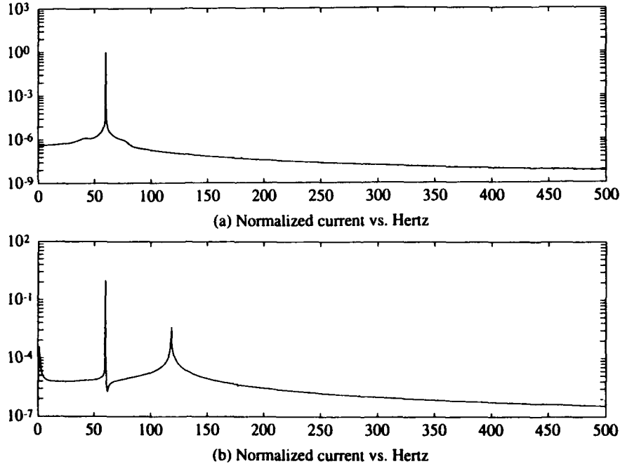
Figure 2. Normalized current spectrum for (a) constant load and (b) sinusoidally varying load.
