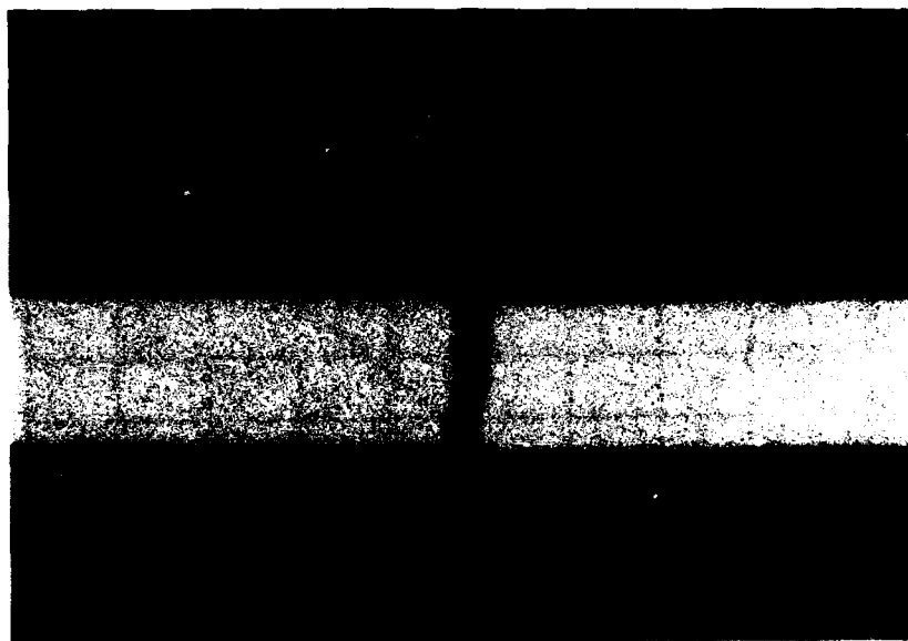
FIGURE 5. CRACK PROGRESS IN FLEXURE FOR 16.8 LBS/FT 3 RIGID POLYURETHANE FOAM.
