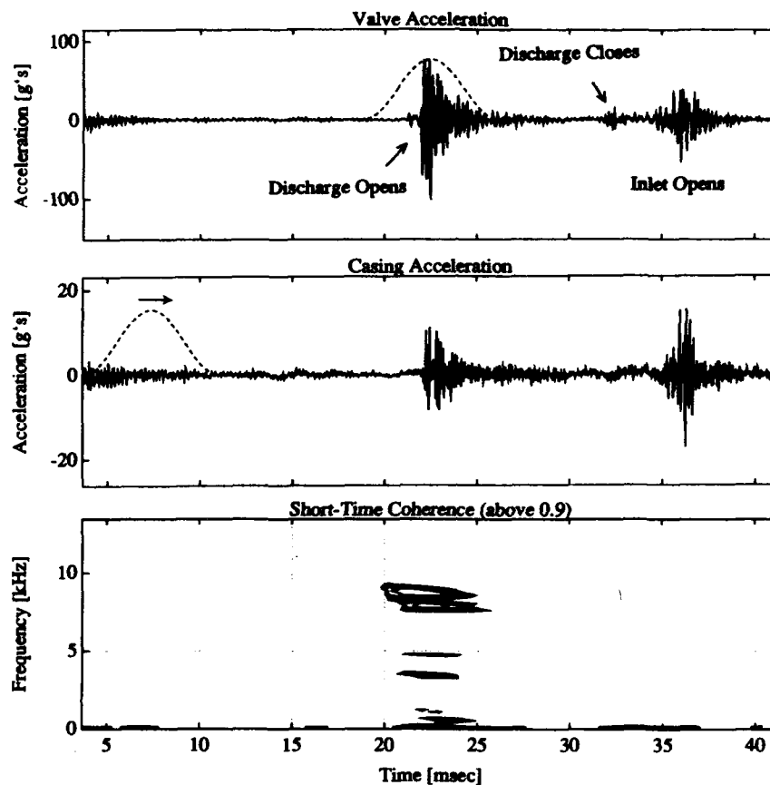
Figure 8: A. Valve body acceleration with analysis window; B. Casing acceleration with first analysis window; C. Short-time coherence (above 0.9).
