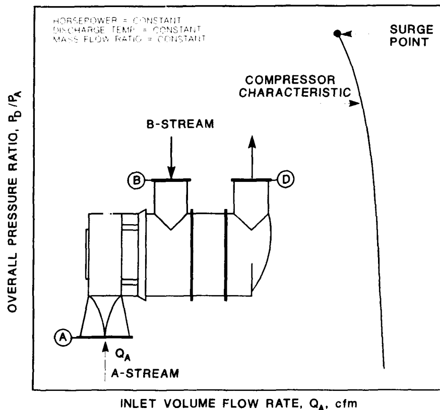
Fig. 1. Typical GDP compressor characteristic
