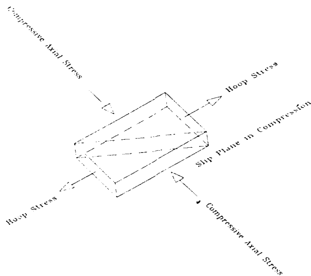
Fig. 2 Slip planes with axial compressive stresses
