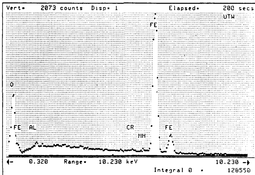
Figure 6. EDS Spectrum of Black Oxide
