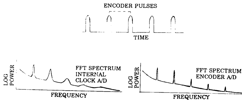
FIG. 3 THE UPPER PLOT SHOWS PULSES FROM A SHAFT ENCODER. THE LOWER LEFT PLOT SHOWS THE COMMON FFT SPECTRUM FOR A MACHINE WITH VARYING RPM. THE LOWER RIGHT PLOT SHOWS THE SPECTRUM OF THE SAME MACHINE WITH AN ENCODER DRIVEN A/D.
