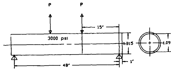
Fig. 5 Four point loading used in both experimental and analytical work.
