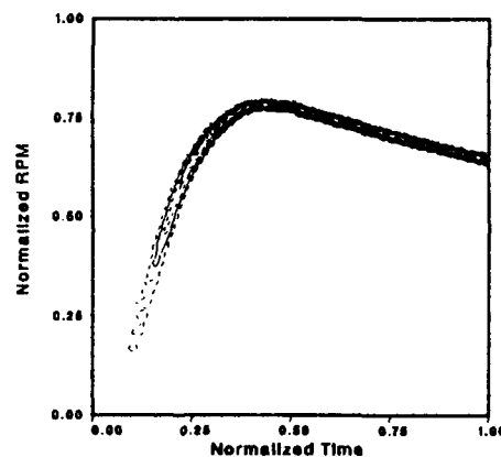
Figure 8. Pseudo Wigner-Ville Distribution of Transient Speed of the Pump
