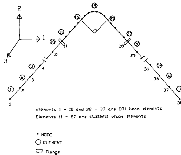
Fig. 13 Finite element model.
