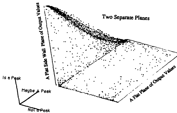
Figure 3 Neural Scalar Outputs Plotted Against Actual Values from One Data Set. Showing Non-linear Clustering Along One Plane Diagonal.
