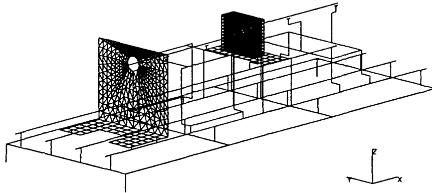
Fig. 1. Finite element model of a laboratory test arrangement consisting of a shaft, a gearbox and a supporting structure.
