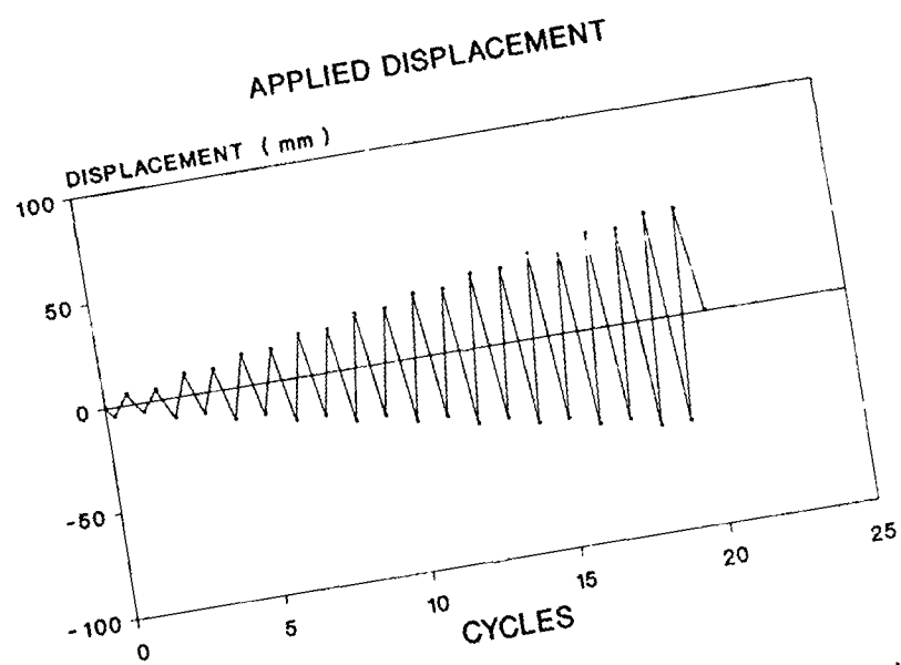
Fig. 12 Applied cyclic displacement.
