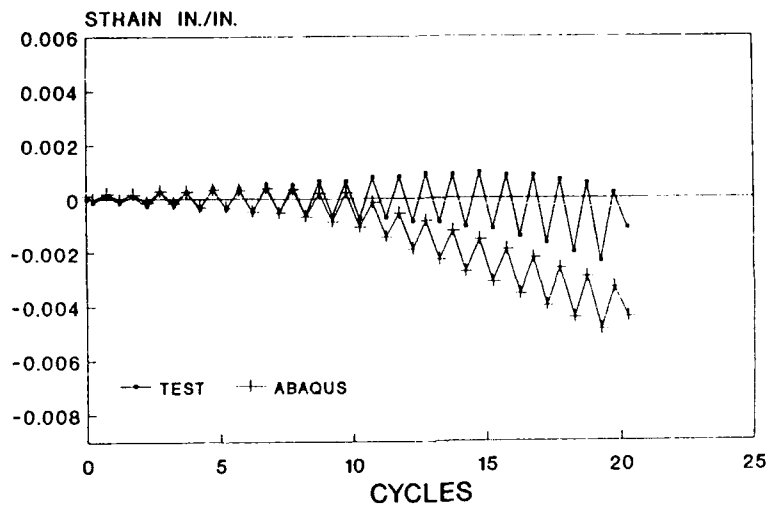
Fig. 15 Calculated and measured axial strains at 30°.
