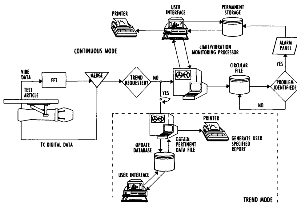
Fig. 1. Health Monitoring System (HEMOS) overview.
