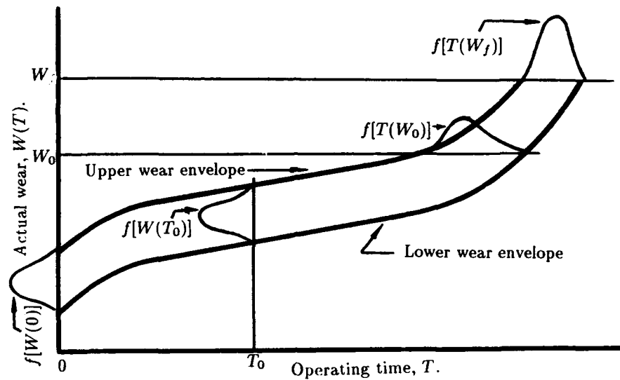
Fig. 4—Wear-life distribution families demonstrating the stochastic behavior of the wear process.
