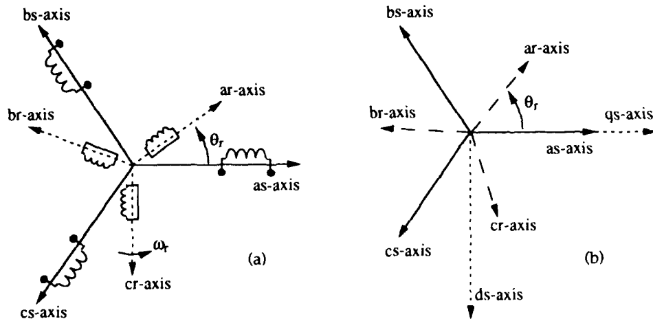
Figure 1. (a) Three phase equivalent windings, (b) abc- and dq-coordinate axis.
