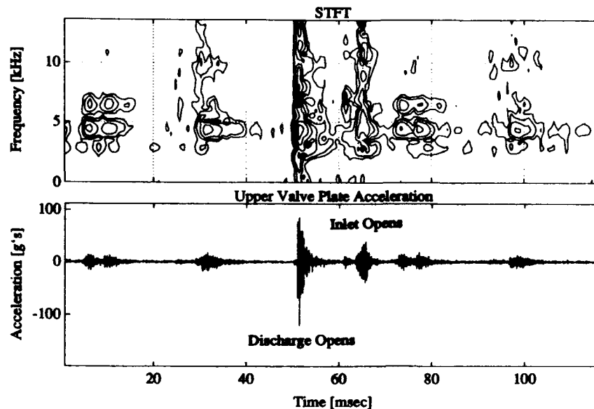
Figure 5: STFT and time-waveform of the valve body acceleration.
