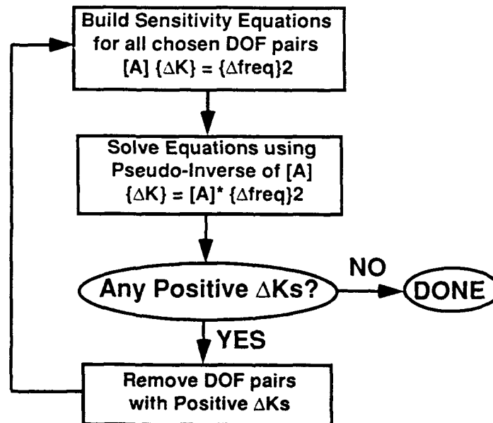
Figure 11. Maximum Negative Stiffness Search Method.
