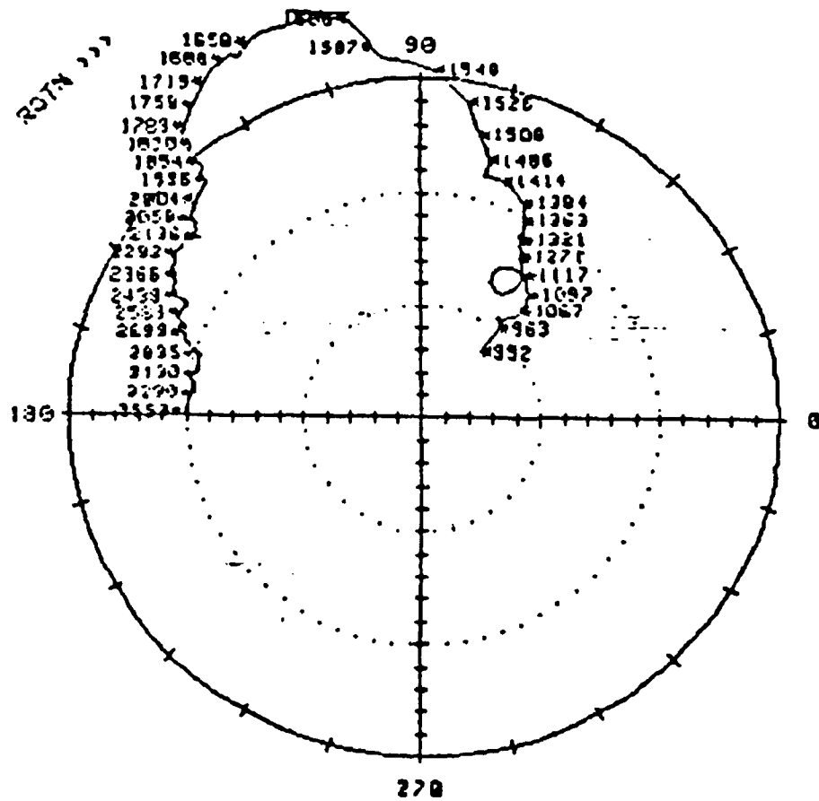
FIG 2A POLAR PLOT OF SYNCHRONOUS RESPONSE (IX) OF A CRACKED TURBOGENERATOR ROTOR. (SEE FIG. 2B FOR 2 DAYS LATER).
