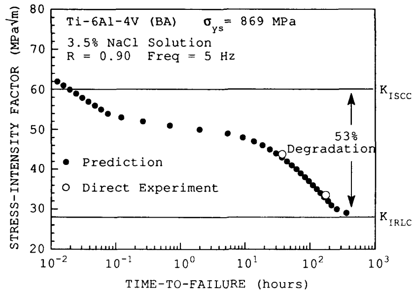
Figure 4. Ripple-load degradation in beta-annealed Ti-6Al-4V
