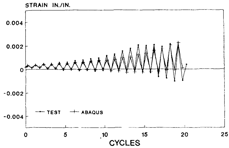
Fig. 17 Calculated and measured axial strains at 90°.
