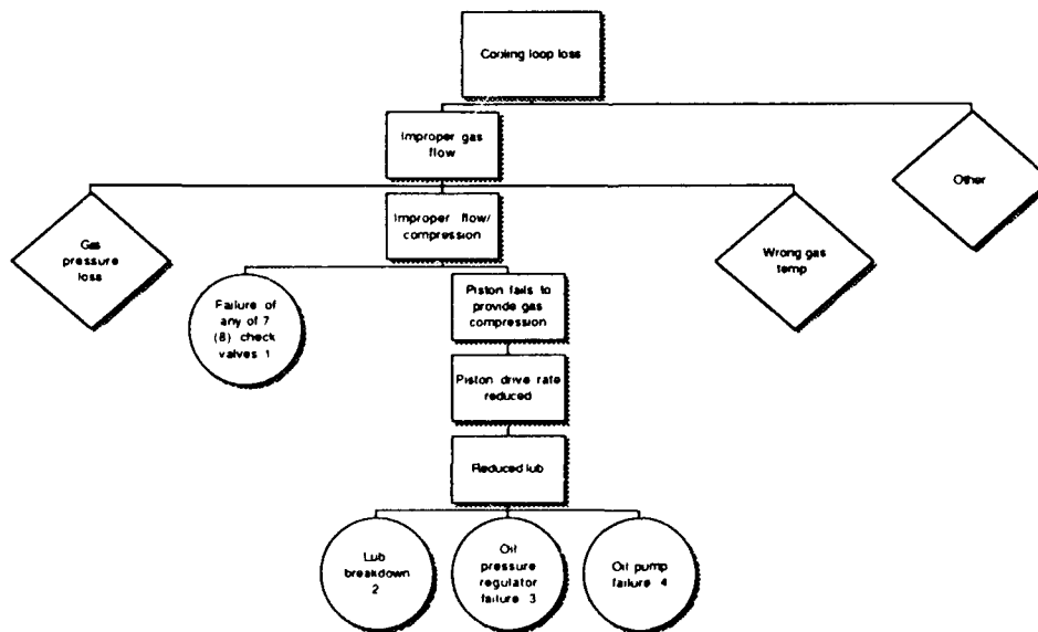
Figure 2 Fault Tree Example For Refrigerator
