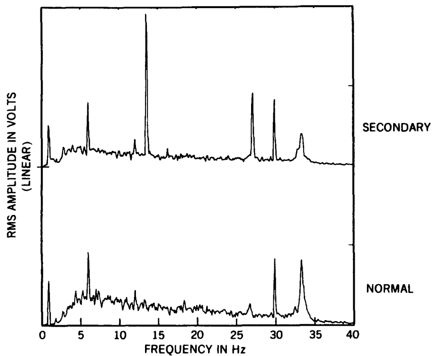
Fig. 6. AM demodulated motor-current spectra.
