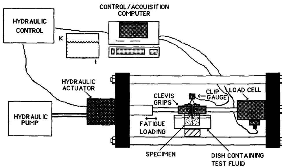
Figure 3. Corrosion-fatigue test machine
