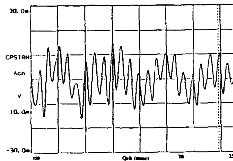
Fig. 7a. Cepstrum at the beginning.
