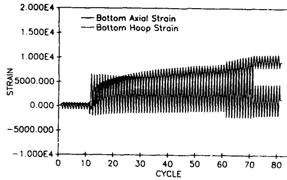
Fig. 7 Specimen 4, 304 SS, Strain -\mu\text{in./in.} Pressure = 3,000 psi, Loading 1, Displacement = 0.25", Center Deflection = 0.533" Loading 2, Displacement = 1.0", Center Deflection = 2.570" Loading 3, Displacement = 1.5", Center Deflection = 3.911", Maximum Load = 1,645 lbs. Loading 4, Displacement = 1.0", Center Deflection = 2.422"
