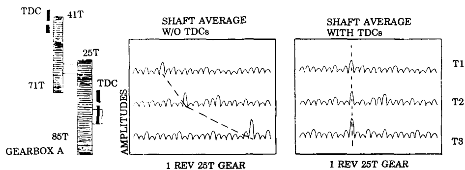
FIG. 4 COMPARISON OF SHAFT AVERAGES WITH AND WITHOUT MULTIPLE TDCs ILLUSTRATES TOOTH TRACKING AT TIMES T1, T2, AND T3
