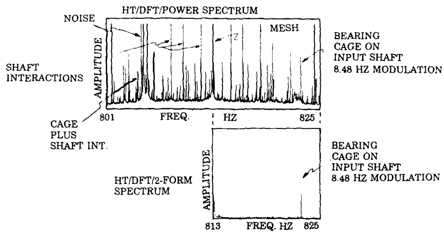
FIG. 10 THE HT/DFT/POWER SPECTRUM IS COMPARED TO THE HT/DFT/2-FORM SPECTRUM (WITH DELETION OF SHAFT INTERACTIONS).
