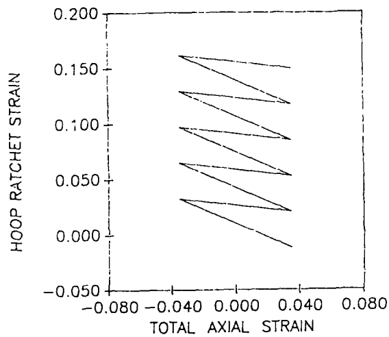
Fig. 3 Hoop ratcheting plotted against the cyclic axial strain based on the Edmunds-Beer model [5].
