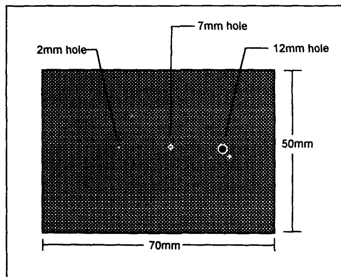
Figure 6. Plate Structure Showing Holes to Scale.
