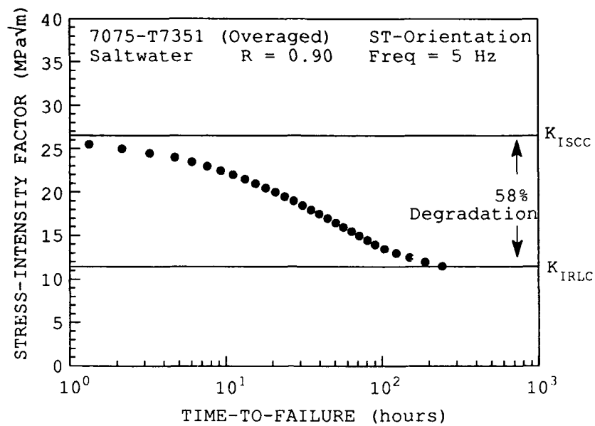
Figure 6. Ripple-load degradation in ST-oriented, overaged 7075-T7351
