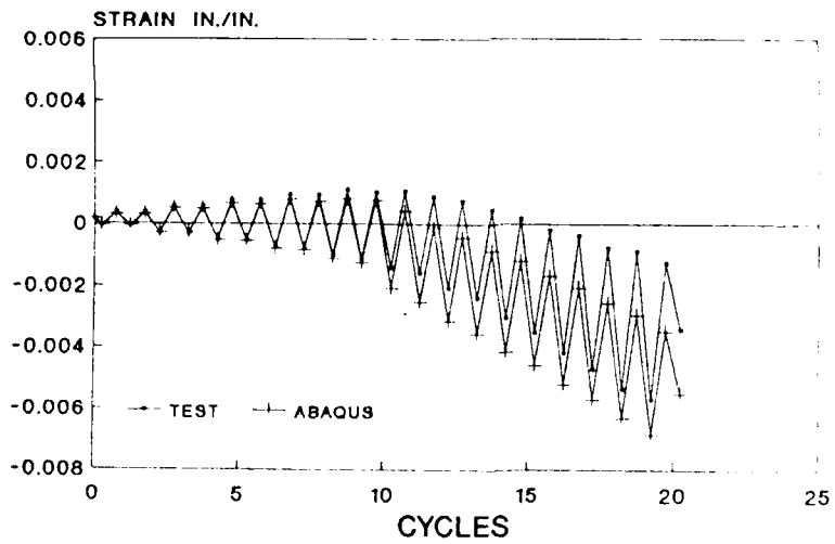
Fig. 16 Calculated and measured axial strains at 60°.
