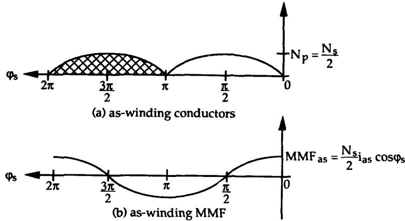
Figure 4. Stator phase (a) winding distribution and (b) produced MMF.
