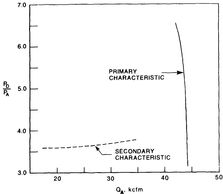
Fig. 2. Primary and secondary operating characteristics.
