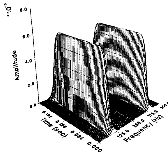
Fig. 2 Pseudo Wigner-Ville distribution of 100 and 400 Hz Pure Sine Waves ( f_s=1000 Hz, N=256 and Smoothing Window Size=10x10)
