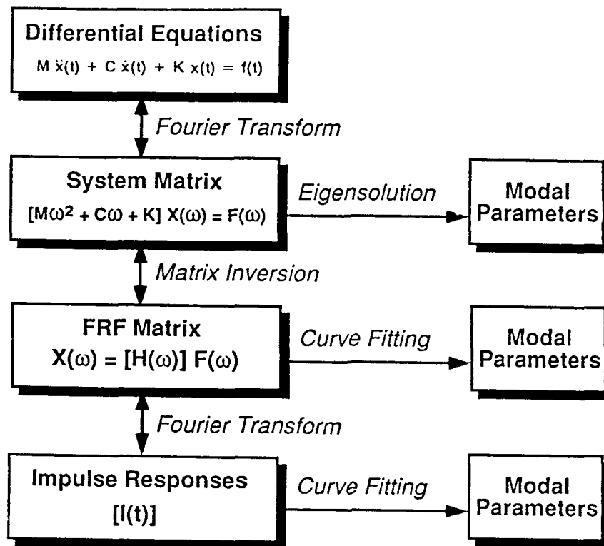
Figure 1. Equivalent Representations of Structural Dynamics.
