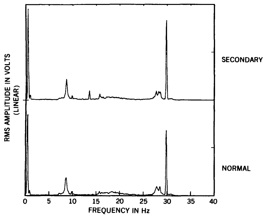
Fig. 5. Spectra of compressor coupling flange displacement probe signals.
