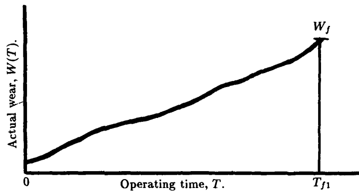
Fig. 1— The sample function ( sf ) of wear W(T) to failure at W_f .
