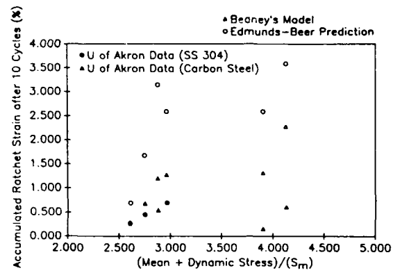
Fig. 9 Comparison of hoop ratcheting strain with predictions.
