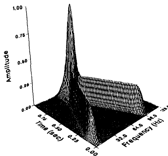
Fig. 4 Composite Signal with Two Frequency Components at Each Time;
