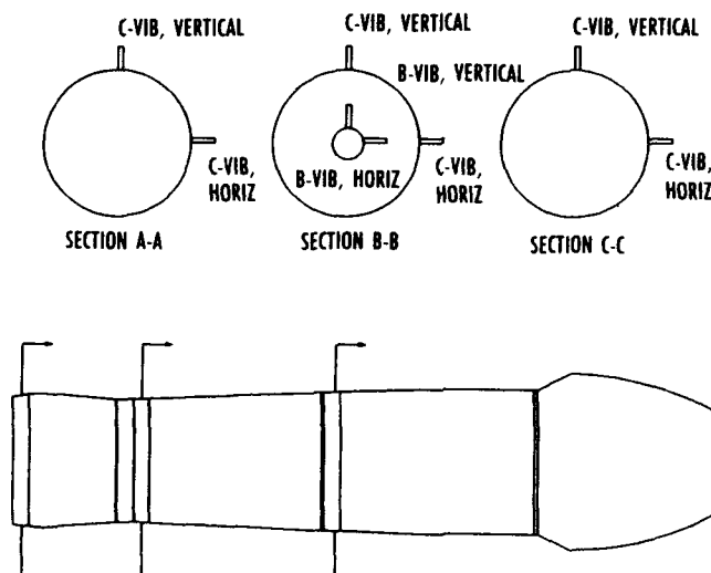
Fig. 2. Typical vibration sensor array for an altitude test article. (Bearing sensors may/may not be located in each plane show).
