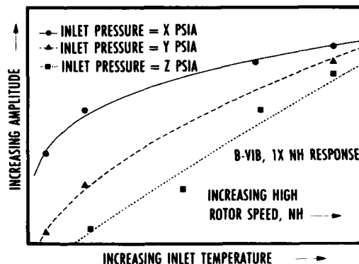
Fig. 5. Effects of inlet temperature on bearing maximum vibratory response.
