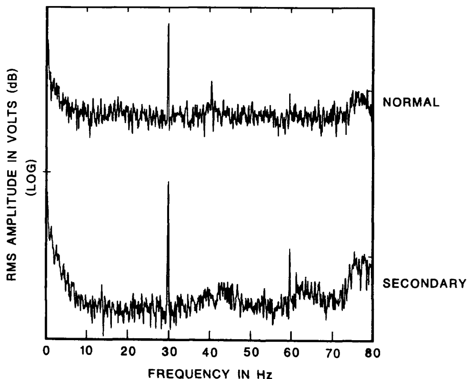
Fig. 4. Spectra of load-bearing, vertical-axis accelerometer signals
