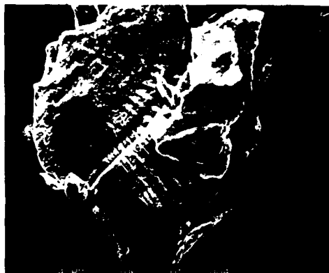
Figure 6 Significant particle illustrates the form due to spalling wear (magn. plug orange 110.25h)
