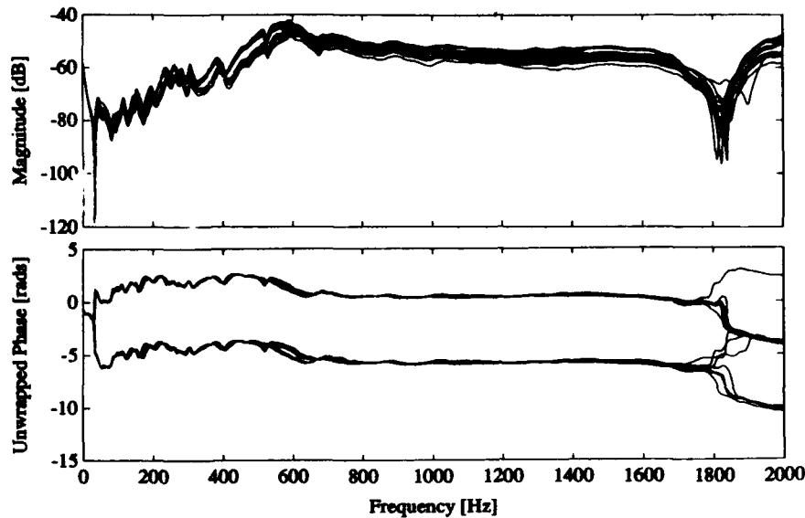
Figure 1: Variations in transfer function magnitude and phase due to changes in temperature (75°F to 210°F).
