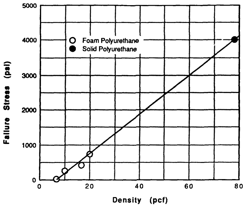
FIGURE 7. GRAPH OF FAILURE STRESS VS. DENSITY FOR SOLID AND FOAM POLYURETHANES.
