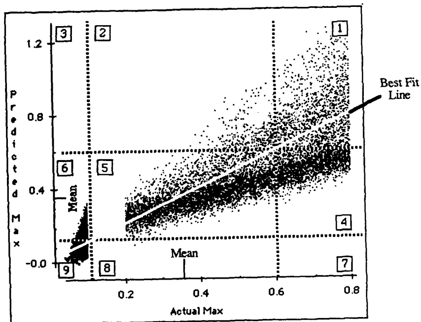
Figure 4 Multi-variable Statistical Fit from One Sample Data Set
