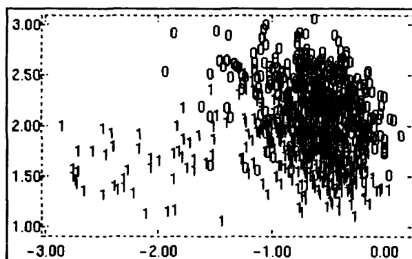
Figure 2. PCA - Nominal Range of Weld Currents (0=Unacceptable, 1=Acceptable)
