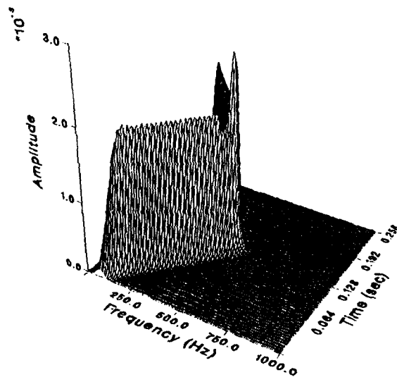
Fig. 5 Linear Chirp Signal with One Frequency Component at Each Time ( f_s=2000 Hz, N=512 and Smoothing Window Size= 16 \times 16 )
