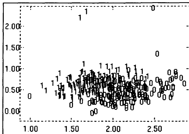
Figure 4. PCA - Medium Current Weld (0=Unacceptable, 1=Acceptable)
