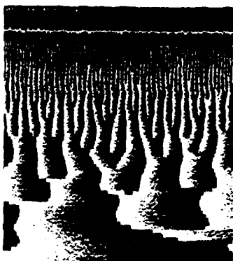
Figure 3. Wavelet transforms of white noise and transient signals.
