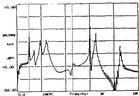
Fig. 6a. Spectrum at the beginning.
