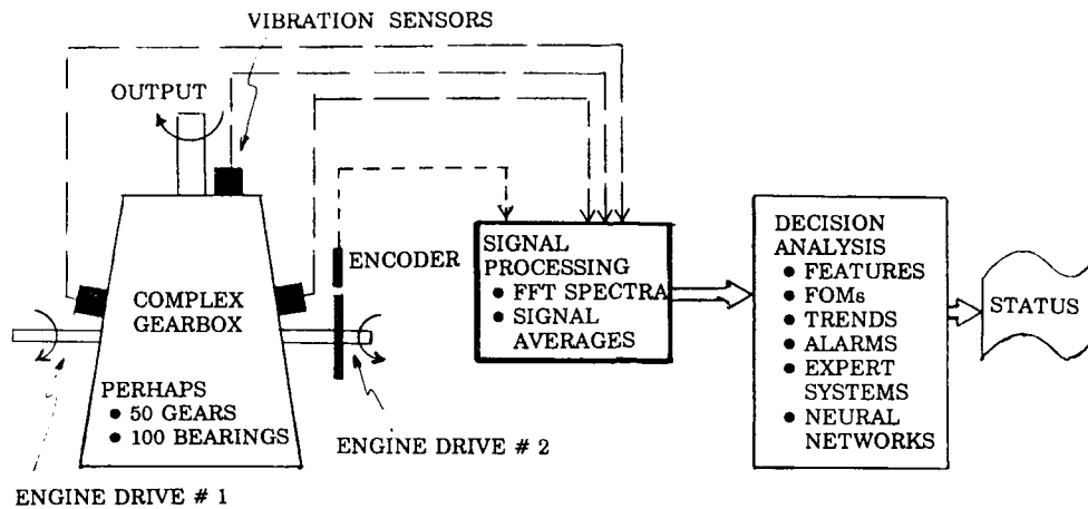
FIG. 1 CONVENTIONAL VIBRATION MONITORING SYSTEM FOR ON-LINE GEARBOX FAULT DETECTION
