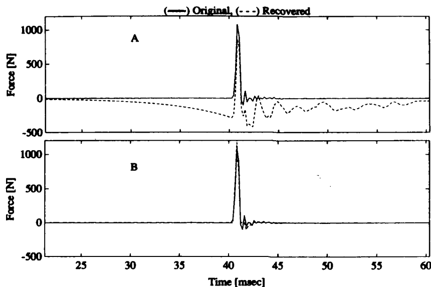
Figure 2: Recovery of impulsive source waveforms applied to the compressor structure using an instrumented hammer: A. Basic inverse filtering; B. Inverse filtering in conjunction with minimum-phase processing and cepstral-smoothing.
