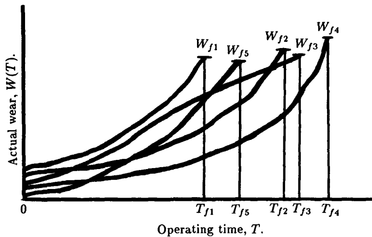
Fig. 2— Five sf 's of wear W(T) to failure at W_f .
