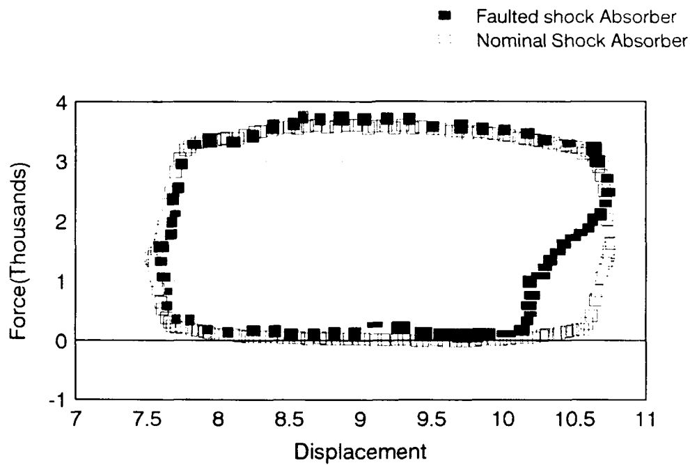
Figure 4. Force vs. Displacement Plot of Shock Absorber Data
