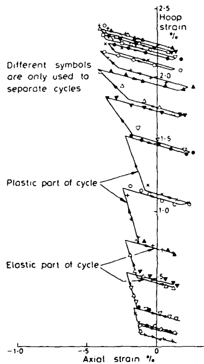
Fig. 4 Hoop ratcheting plotted against the cyclic axial strain based on the experimental work of Beaney.
