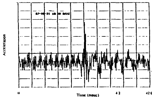
Fig. 4a. Measured time domain signal.
