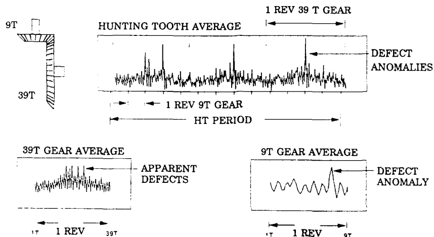
FIG. 8 COMPARISON OF HUNTING TOOTH AVERAGE TO EACH OF THE SHAFT AVERAGES FOR SINGLE DEFECT ON PINION GEAR
