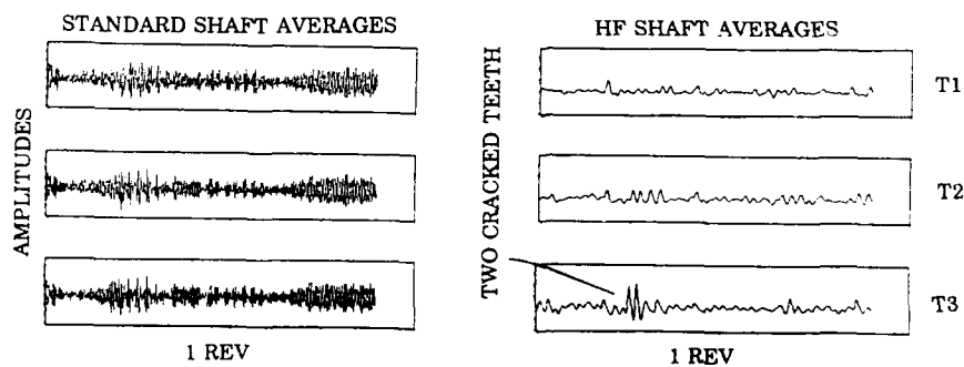
FIG. 9 COMPARISON OF STANDARD SHAFT AVERAGES AND HIGH FREQUENCY SHAFT AVERAGES FOR TOOTH FAULT DETECTION AT TIMES T1, T2, T3
