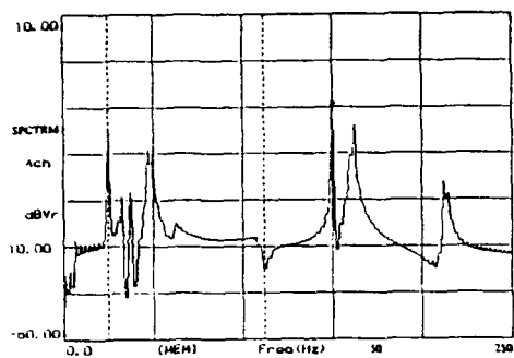
Fig. 6b. Spectrum 2.6% of lifetime remaining.
