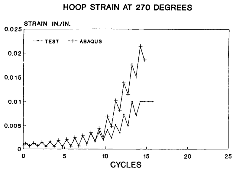
Fig. 19 Calculated and measured hoop strains at 270°.
