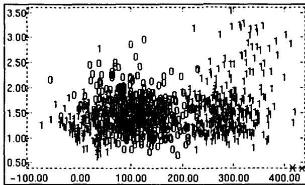
Figure 3. CDA - Nominal Range of Weld Currents (0=Unacceptable, 1=Acceptable)
