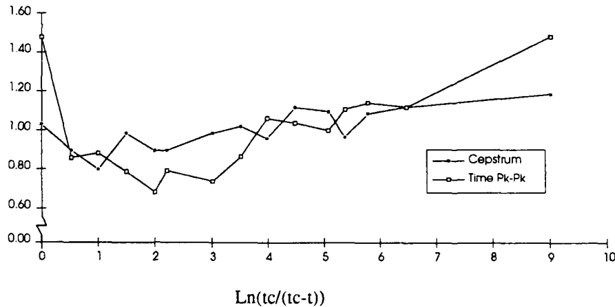
Fig. 3. Normalized cepstral running speed component of the input shaft and normalized peak-to-peak value of synchronized time domain acceleration signal.
