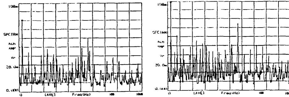
Fig. 5a. Spectrum 2.6% of lifetime remaining. Fig. 5b. Spectrum 0.2% of lifetime remaining.
