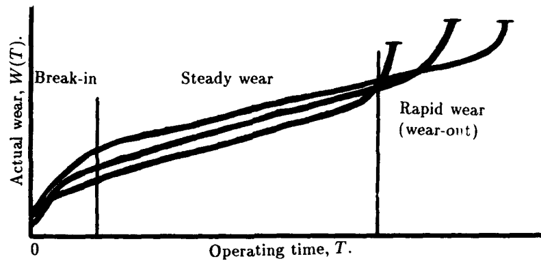
Fig. 3— A typical wear process for mechanical components.
