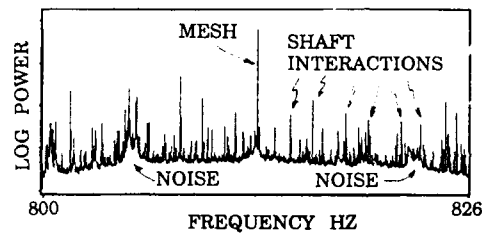
FIG. 2 NARROW-BAND HIGH RESOLUTION POWER SPECTRUM OF GEARBOX A
