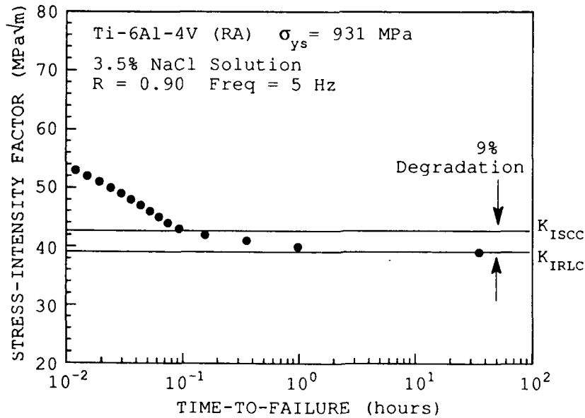
Figure 5. Ripple-load degradation in recrystallization-annealed Ti-6Al-4V
