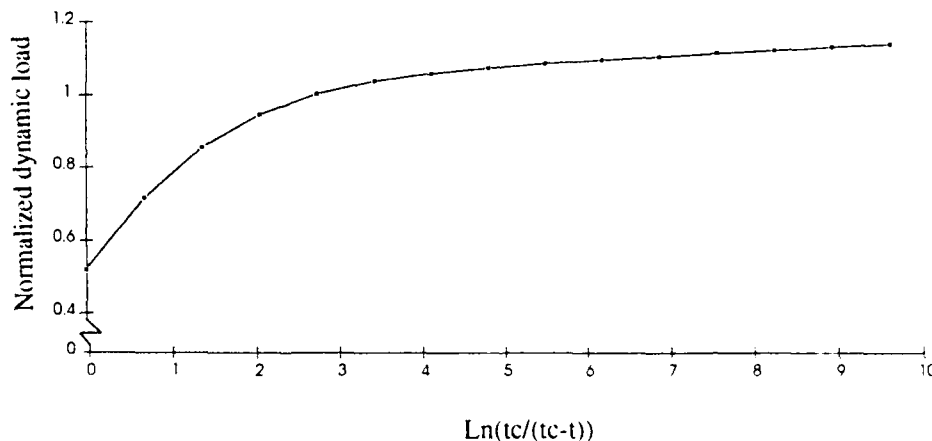
Fig. 2. Normalized sum of dynamic loads on gear teeth.
