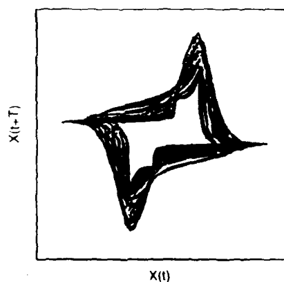
Figure 4. Power spectrum and time delay representation of the van der Pol equation.
