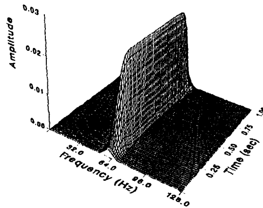
(a) s(t) = \cos(2\pi 60 t)
