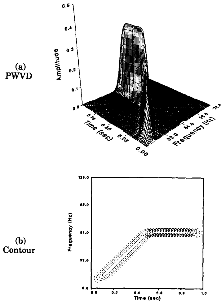
Fig. 6 PWVD of a Composite Signal of Sweeping-up and Steady Frequency (f_g = 256 \text{ Hz}, N = 256 \text{ and Smoothing Window Size} = 10 \times 10)
