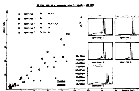
Figure 7 The data show the distribution of wear particle size (length x-axis, width y-axis) and composition (magnetic plug black, 109.55 h operating time)
