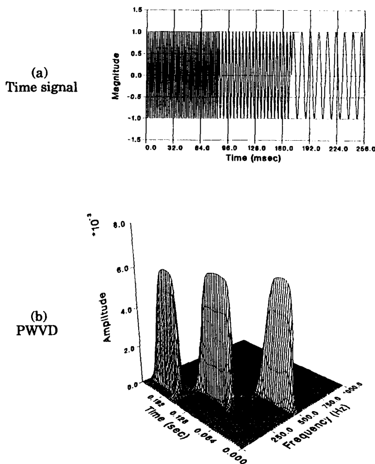
Fig. 3 Sine Wave with Stepwise Frequency Changes: 100, 250 and 500 Hz ( f_s=2000 Hz, N=512 and Smoothing Window Size= 10 \times 10 )
