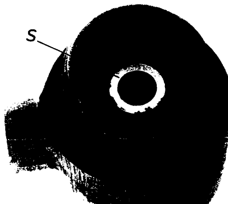
Figure 4 2.1:1 Valve body without tappet washer inset; corrosive attacked con- tact surface (S)
