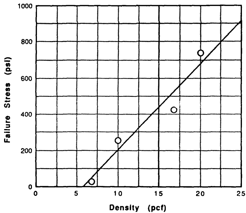
FIGURE 8. GRAPH OF FAILURE STRESS VS. DENSITY FOR POLYURETHANE FOAMS.
