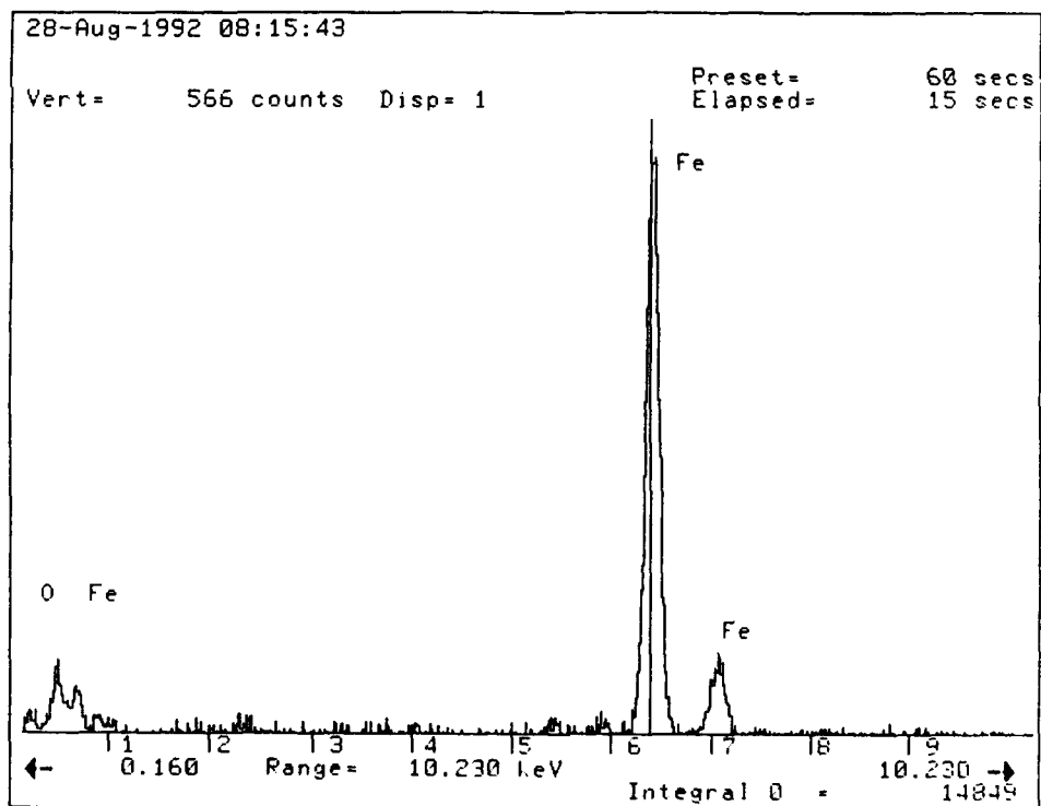
Figure 4 Representative EDS spectrum obtained from the blackened regions at the crack initiation sites.
