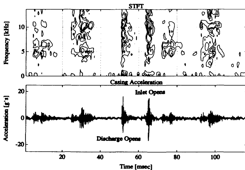
Figure 7: STFT and time-waveform of the casing acceleration.
