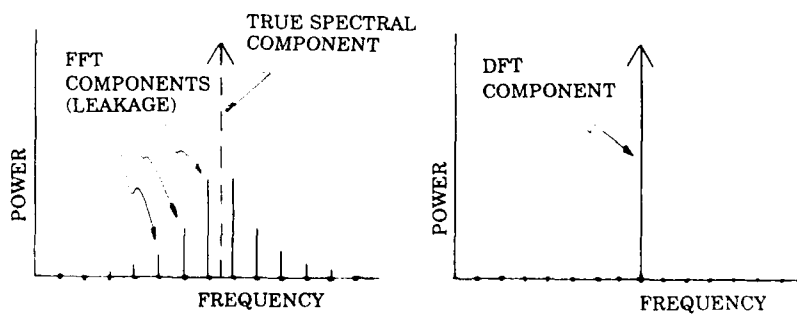
FIG. 6 COMPARISON OF FFT SPECTRUM AND PROPERLY CHOSEN DFT SPECTRUM FOR A SINGLE SPECTRAL COMPONENT
