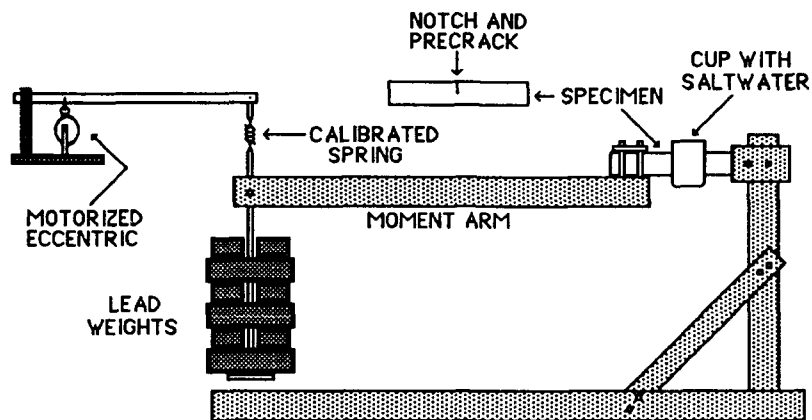
Figure 1. Ripple-load "direct experiment"
