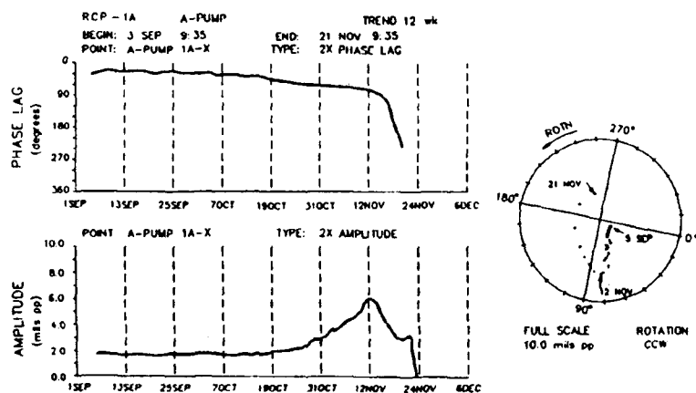
Fig 6 The A mplitude P hase vs T ime plot. This is a trend plot of nX Amplitude and Phase, with x=2 in this figure.
