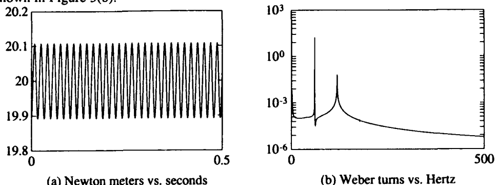
Figure 3.(a) Electromagnetic torque and (b) rotor flux linkage spectrum for a sinusoidally varying load.
