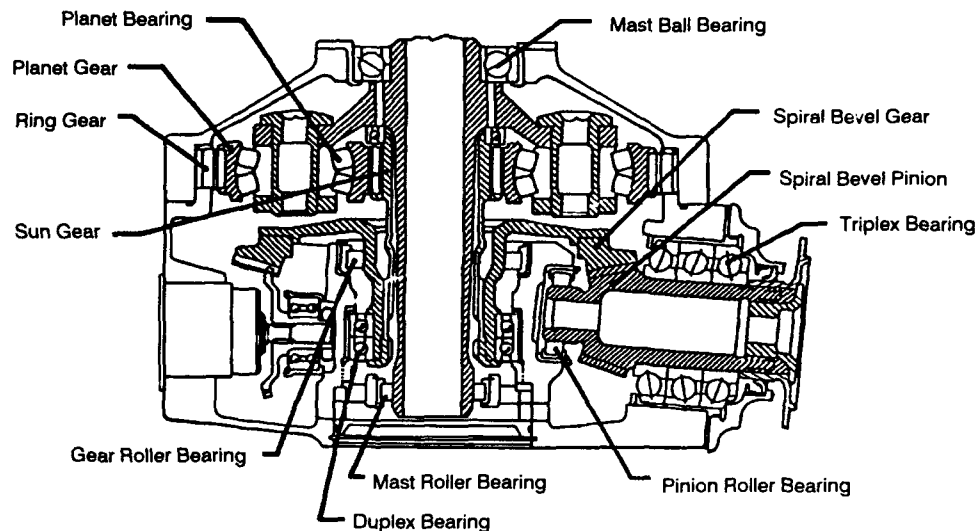
Figure 4: Configuration of the OH-58A main rotor transmission gearbox.
