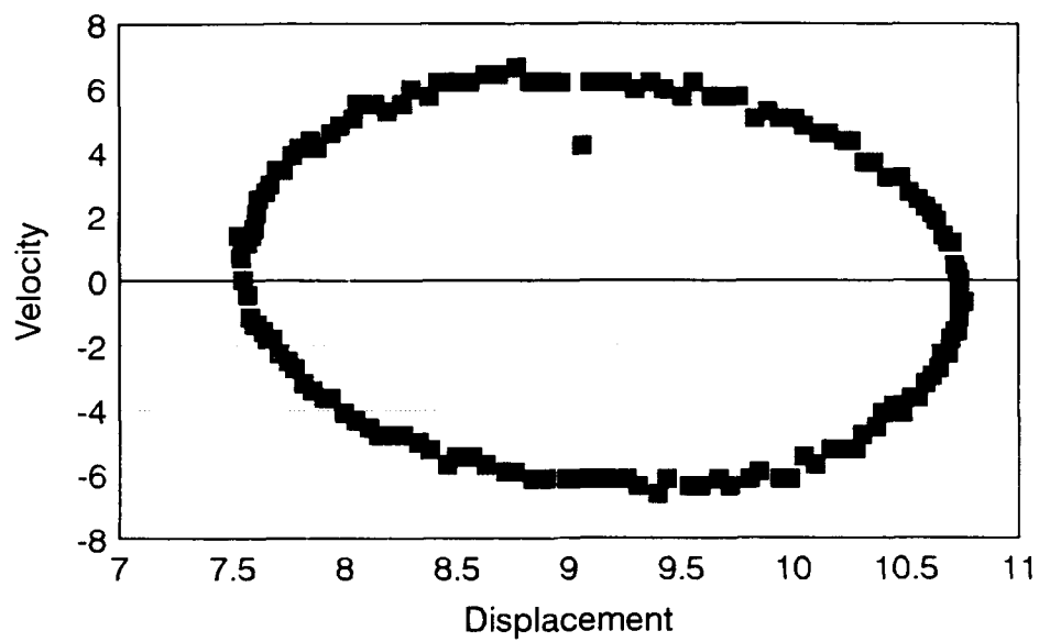
Figure 3. Velocity vs. Displacement Plot of Shock Absorber Data
