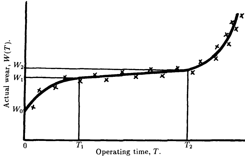
Fig. 5— One envelope of the wear process.
