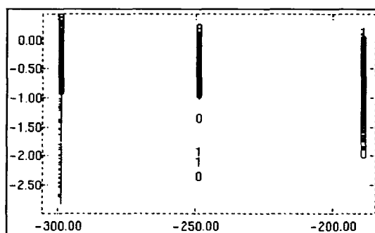
Figure 6. PCA - Nominal Range of Weld Current with Weld Current as Input Parameter (0=Unacceptable, 1=Acceptable)
