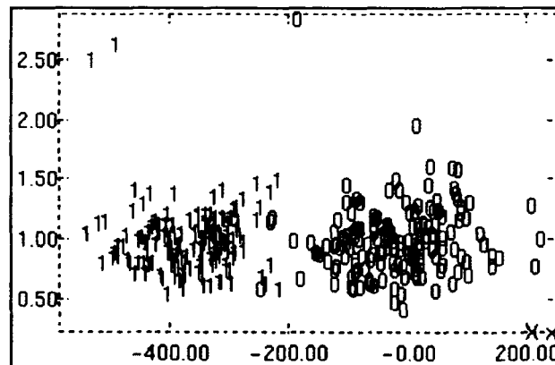
Figure 5. CDA - Medium Current Weld (0=Unacceptable, 1=Acceptable)
