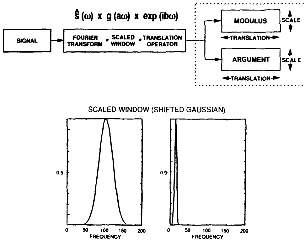
Figure 2. Schematic representation of the continuous wavelet transform calculation.
