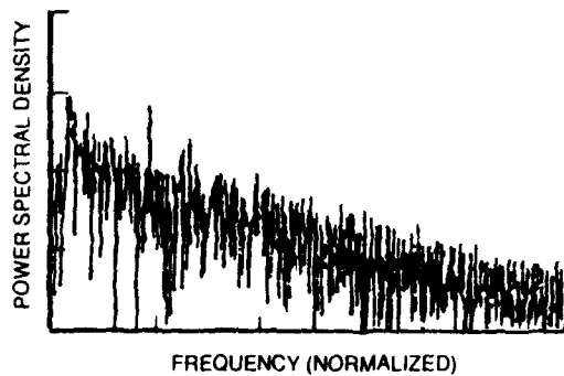
Figure 4. Power spectrum and time delay representation of the van der Pol equation.
