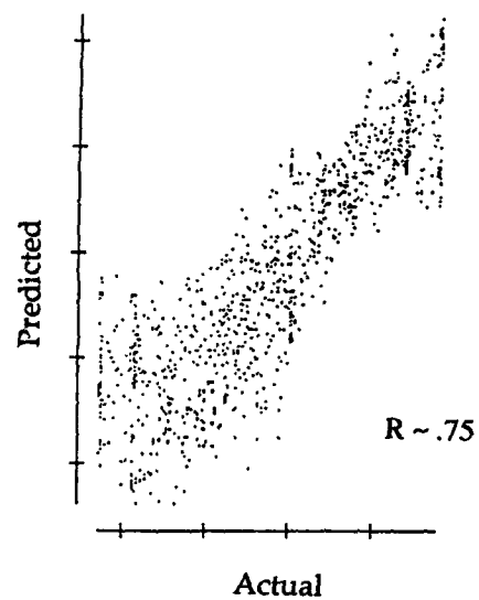
Figure 5 A Statistical Fit - Predicted Versus Actual
