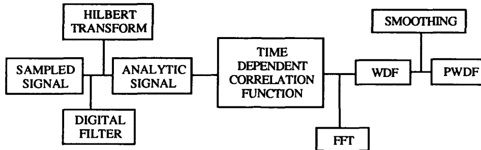
Fig. 1 Computational block diagram of Pseudo Wigner-Ville Distribution
