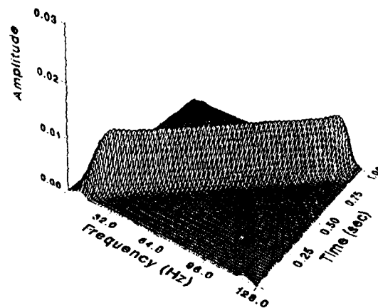
(c) s(t) = \cos(2\pi 64 t^2)
