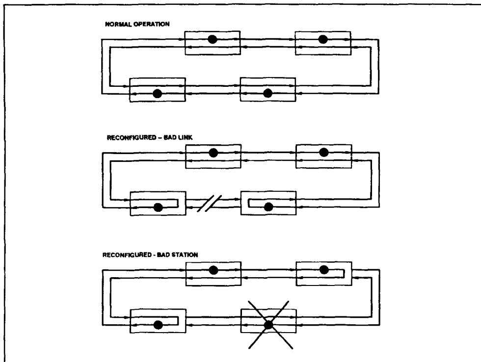
Figure 3. FDDI Counter Rotating Ring Fault Tolerant Examples
