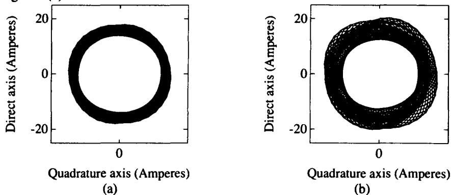
Figure 7. Direct-axis stator current vs. quadrature-axis stator current for (a) eccentric air gap and (b) eccentric air gap
