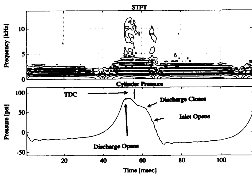
Figure 6: STFT and time-waveform of the cylinder pressure.
