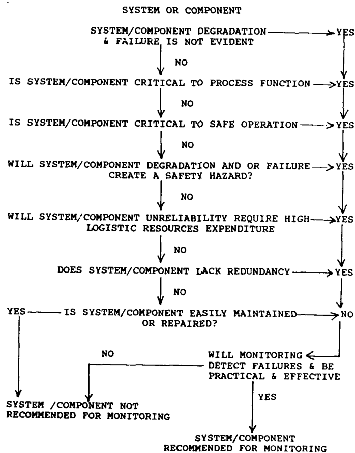
Figure I FLOW DIAGRAM FOR RECOMMENDED MONITORING
