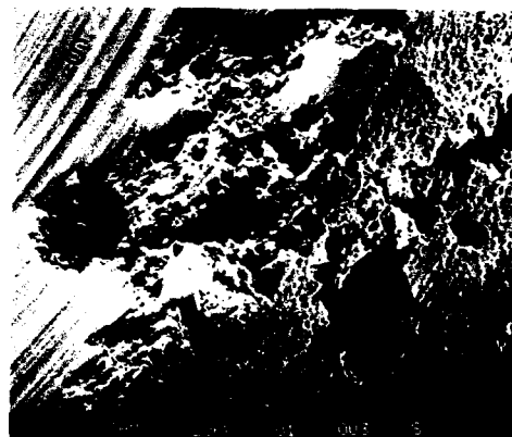
Figure 6 The contact surface 5 (S) and the adjacent surface (AS) were attacked by crevice corrosion
