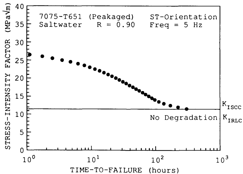
Figure 7. Ripple-load effect in ST-oriented, peak-aged 7075-T651
