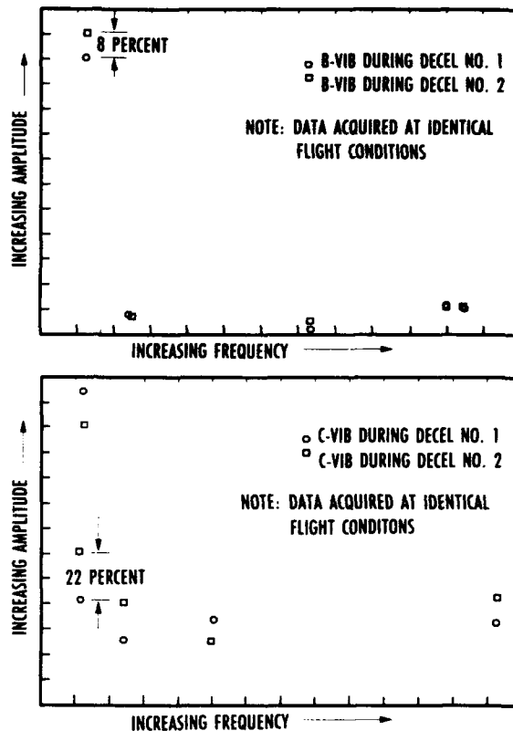
Fig. 6. Response amplitude repeatability versus frequency for bearing (top) and case (bottom) accelerometers.
