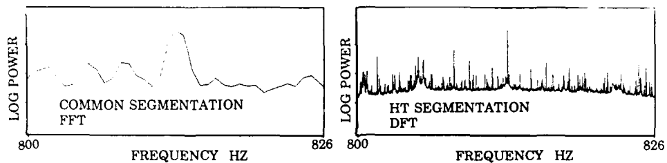
FIG 7. COMPARISON OF STANDARD FFT SEGMENTATION SPECTRUM (4096 PTS) AND HT SEGMENTATION DFT SPECTRUM (175,015 PTS)
