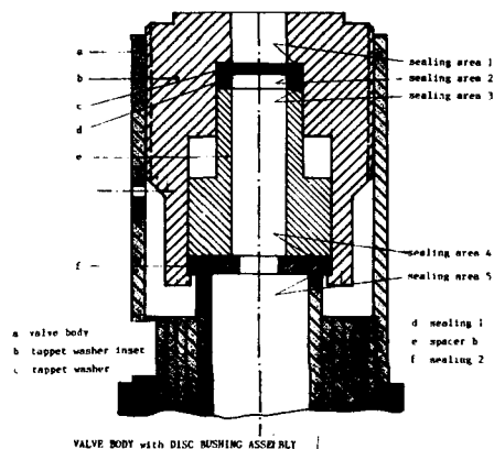
Figure 3 Schematic representation of the valve body with tappet washer inset
