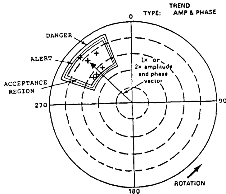
FIG. 1 ACCEPTANCE REGION FOR 1\times AND 2\times RESPONSE VECTORS IN THE POLAR PLOT FORMAT. ACCEPTANCE REGIONS CAN BE DEFINED WITH VARIOUS BOUNDARIES, DEPENDING UPON THE VIBRATION CHARACTERISTICS OF EACH MACHINE UNDER ALL NORMAL OPERATING CONDITIONS
