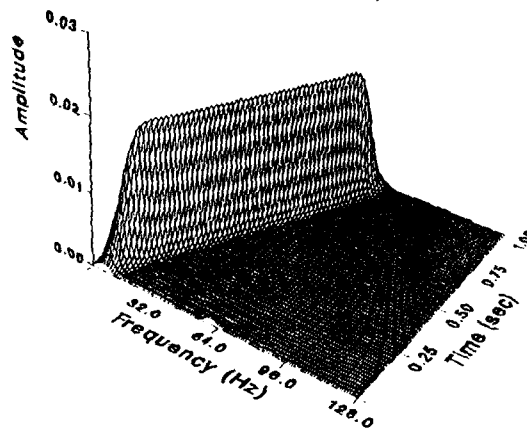
(b) s(t) = \cos(2\pi 32 t^2)
