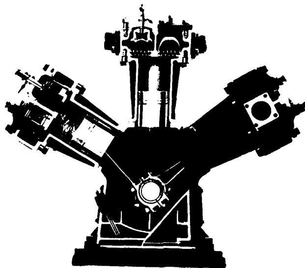
Figure 3: Cutaway view of the compressor.
