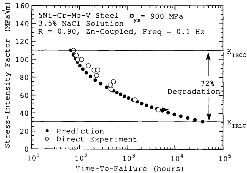
Figure 2. Ripple-load degradation in 5Ni-Cr-Mo-V steel
