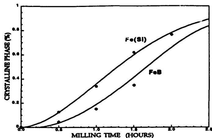
Fig. 3 Crystallization rate for both phases for Spex milling experiment
