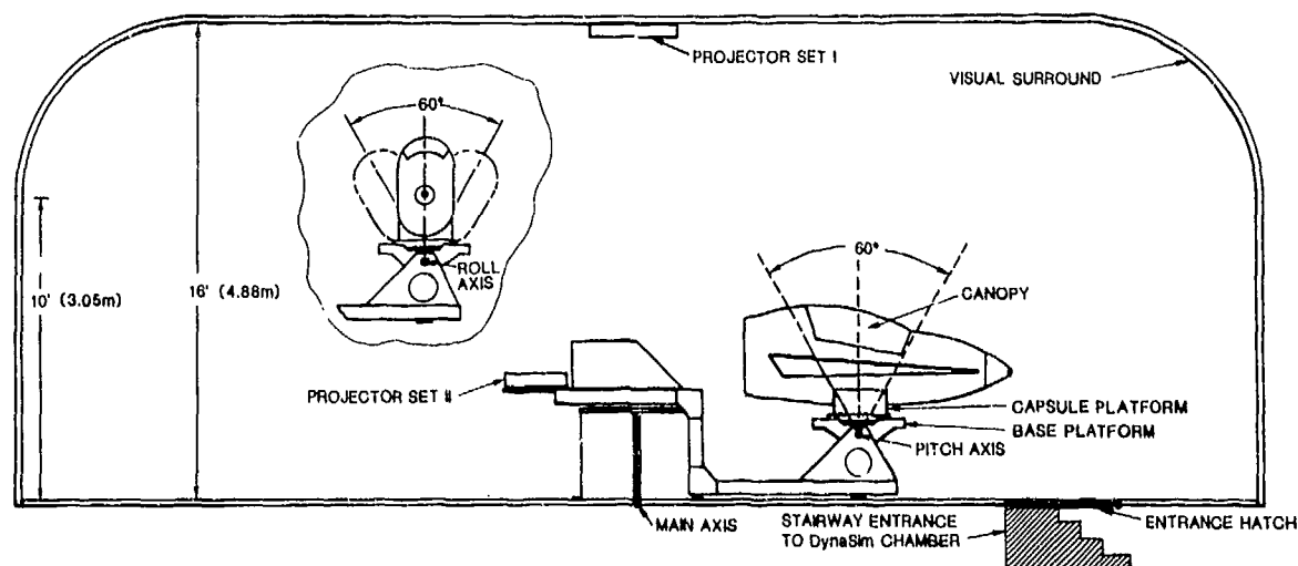
Figure 2. Elevation sketch showing chamber, Vertifuge fuselage (in centrifugal configuration), Projector Set I (overhead projectors), Projector Set II (onboard projectors) and entrance way.
