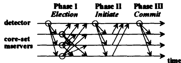
Figure 29: Election and Change-processing Protocol
