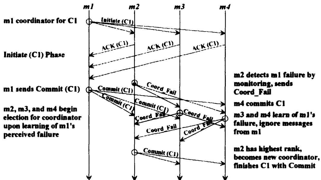
Figure 35: Coordinator Failure In Commit Phase
