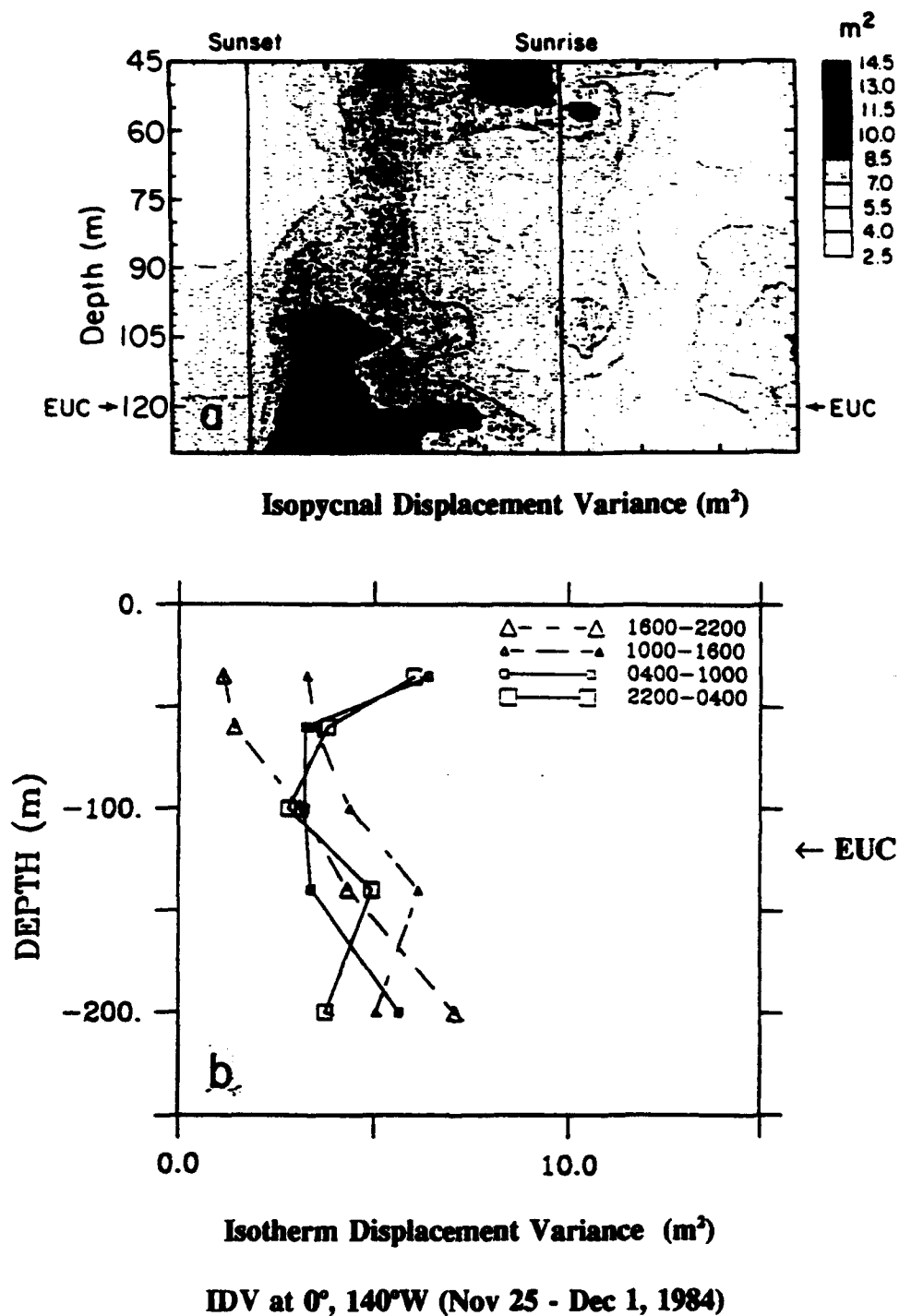
Figure 3.10. Comparison between a) mean isopycnal displacement variance from TROPIC HEAT microstructure measurements by Wijesekera and Dillon (1991) during November 25-December 1, 1984 at 0°, 140°W, and b) mean isotherm displacement variance (IDV) for four six-hour time bins using moored buoy data from the same time period and location.
