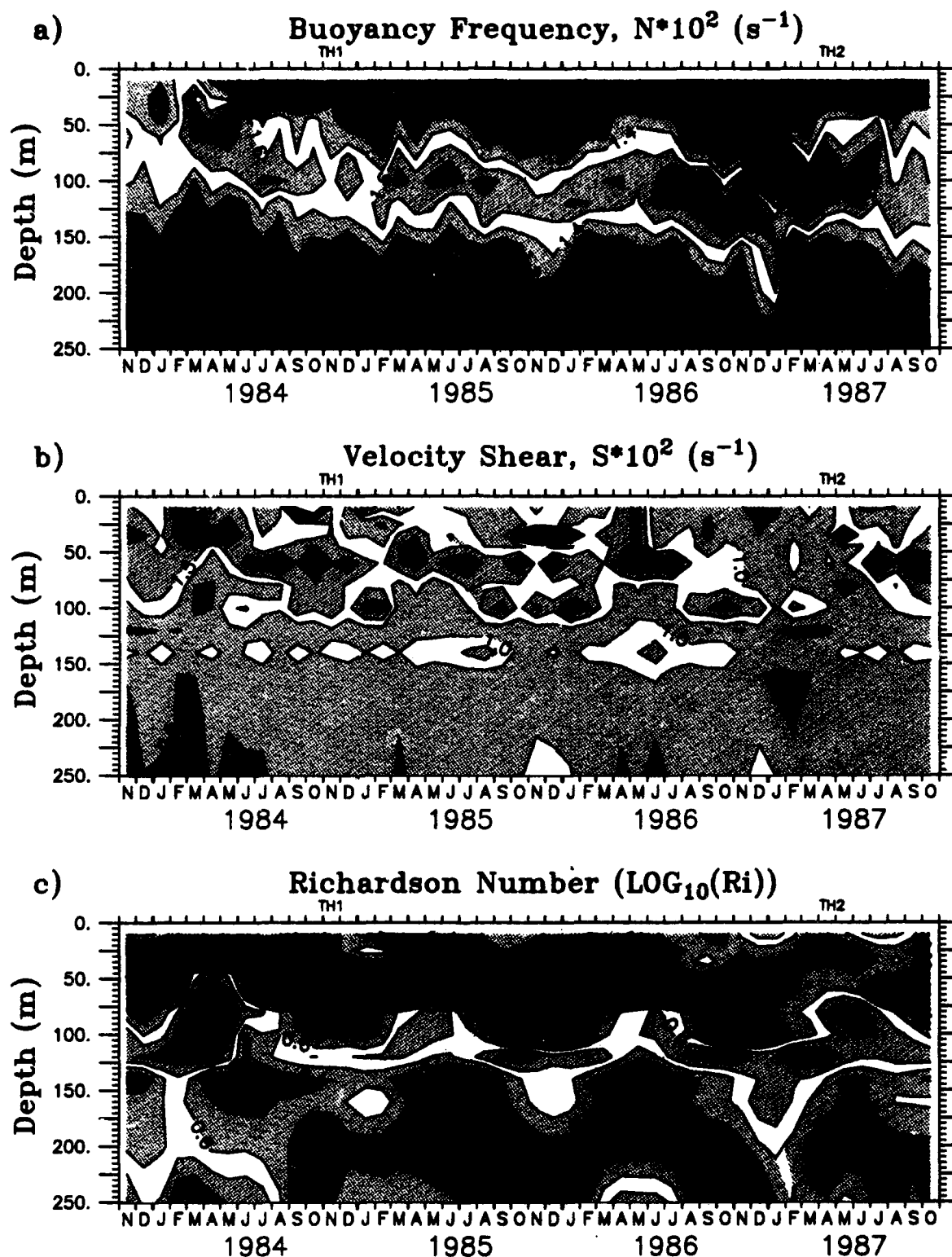
Figures 4.6a-c. Time-depth contour plots of monthly mean values of a) buoyancy frequency, N b) velocity shear, S and c) gradient Richardson number, Ri , from 10 m to 250 m over the period November 1983 - October 1987. TH1 and TH2 at the top of each plot indicate the approximate time of the TROPIC HEAT experiment microstructure measurements.
