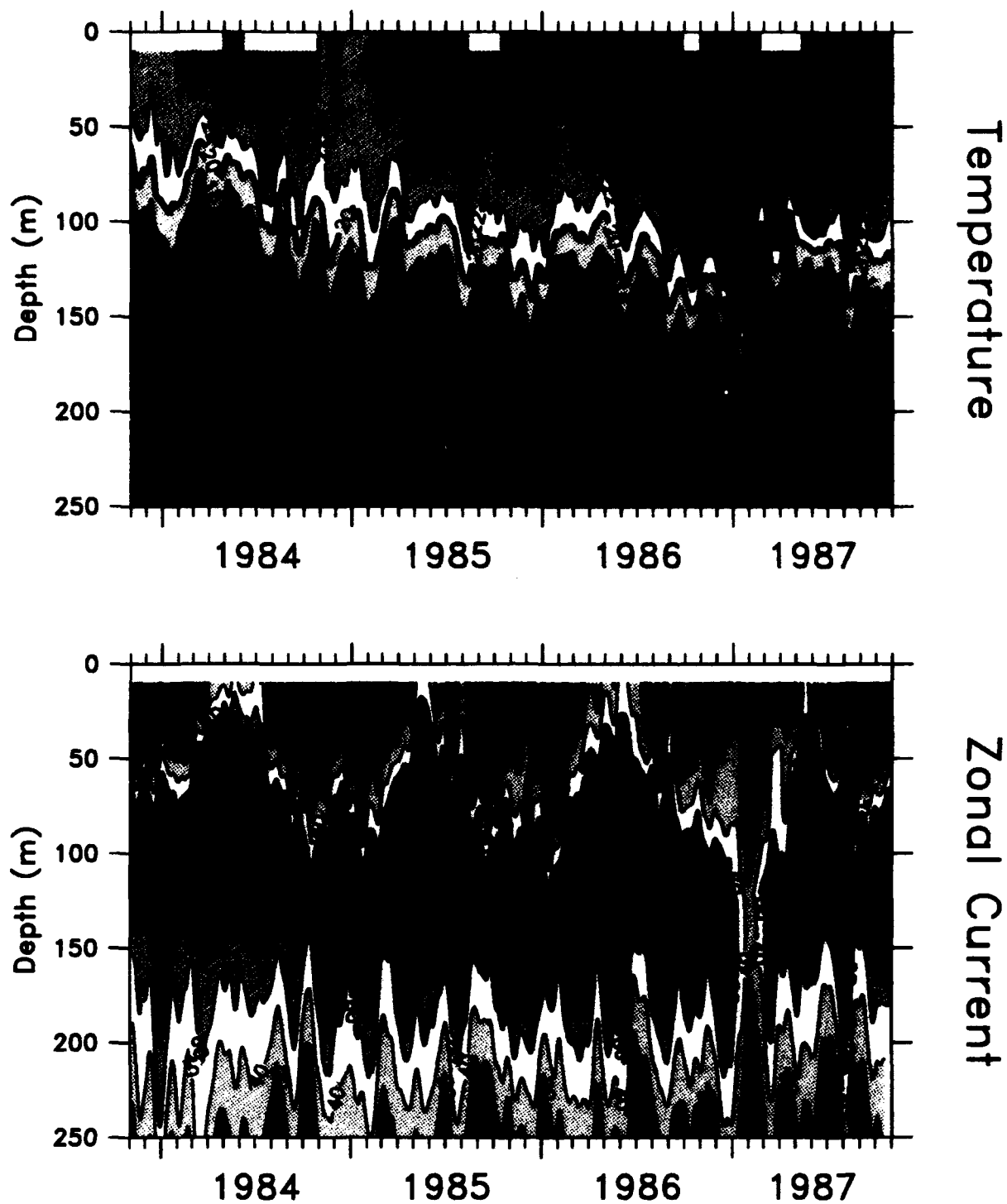
Figure 4.5. Time series measurements of a) temperature and b) zonal current velocity at 0^\circ , 140^\circ\text{W} for the period November 1983 - October 1987. These plots were computed from daily mean values which were then smoothed using a 17-day triangular low-pass filter.
