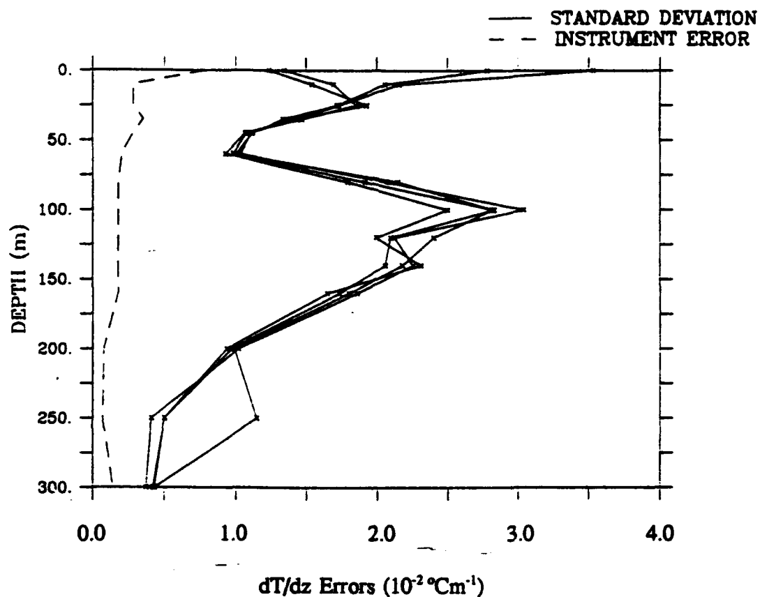
Temperature Gradient Error at 0^\circ, 140^\circ\text{W} (Nov 84)
