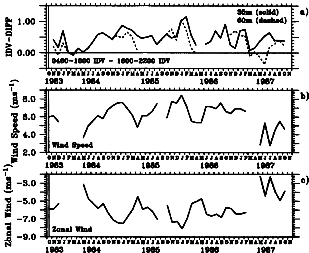
Figure 6.6. Time series of monthly mean diurnal differences of isotherm displacement variance ( \Delta\text{IDV}_{\text{m}} ) at 35 m and 60 m, wind speed, and zonal wind during November 1983-October 1987. \Delta\text{IDV} computed as 0400-1000 IDV minus 1600-2200 IDV normalized by the mean IDV.
