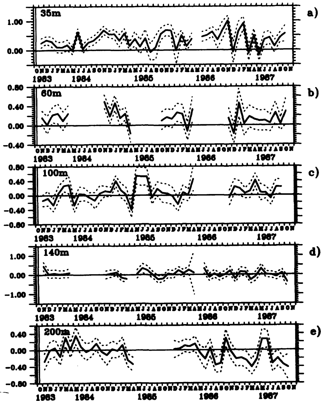
Figure 6.2. Monthly mean diurnal differences of isotherm displacement variance ( \Delta IDV_m ) computed from daily values of 2200-0400 IDV minus 1000-1600 IDV normalized by the mean of the two IDV values at a) 35 m, b) 60 m, c) 100 m, d) 140 m, and e) 200 m. Dashed lines indicate \pm one standard error of the mean.
