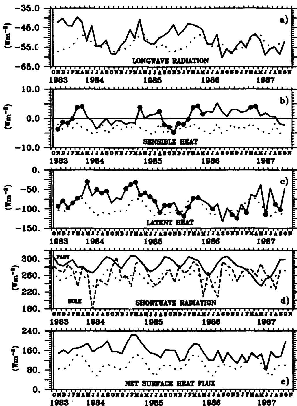
Figure 4.2. Monthly mean surface heat flux terms at 0°, 140°W for the period November 1983 -October 1987: a) longwave radiation, Q_l , b) sensible heat flux, Q_h , c) latent heat flux, Q_e , d) shortwave radiation, Q_s , by FAST radiative scheme (solid line) and BULK formula (dashed line), and e) net surface heat flux, Q_{net} . Climatological values are given by dotted lines. Downward fluxes are positive.
