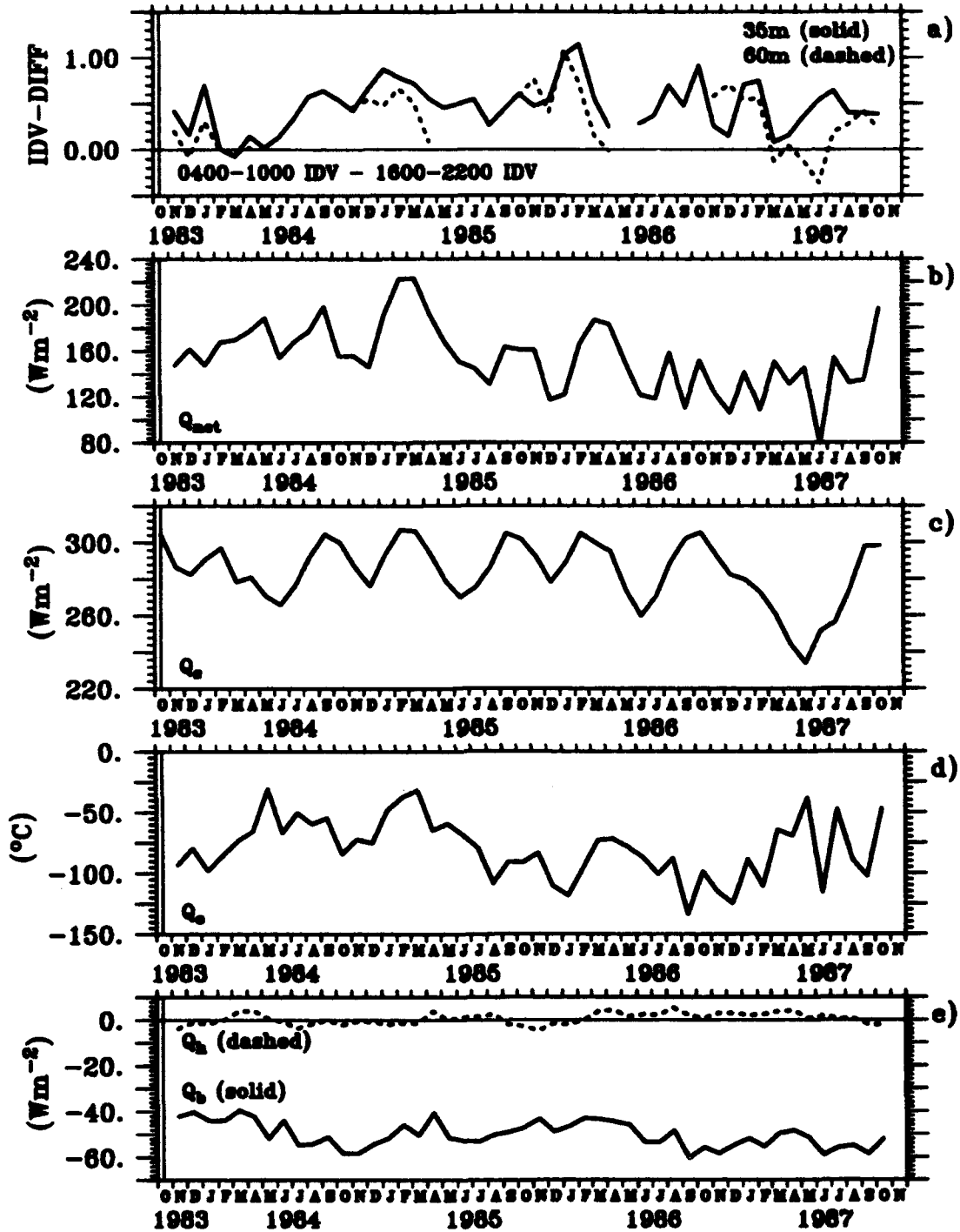
Figure 6.7. Time series of monthly mean a) diurnal differences of isotherm displacement variance ( \Delta IDV_{mc} ) at 35 m and 60 m, b) net surface net flux, Q_{net} , c) shortwave radiation, Q_s , d) latent heat flux, Q_e , and e) longwave radiation, Q_b , and sensible heat flux, Q_h , during November 1983-October 1987. \Delta IDV_{mc} computed as 0400-1000 IDV minus 1600-2200 IDV normalized by the mean IDV.
