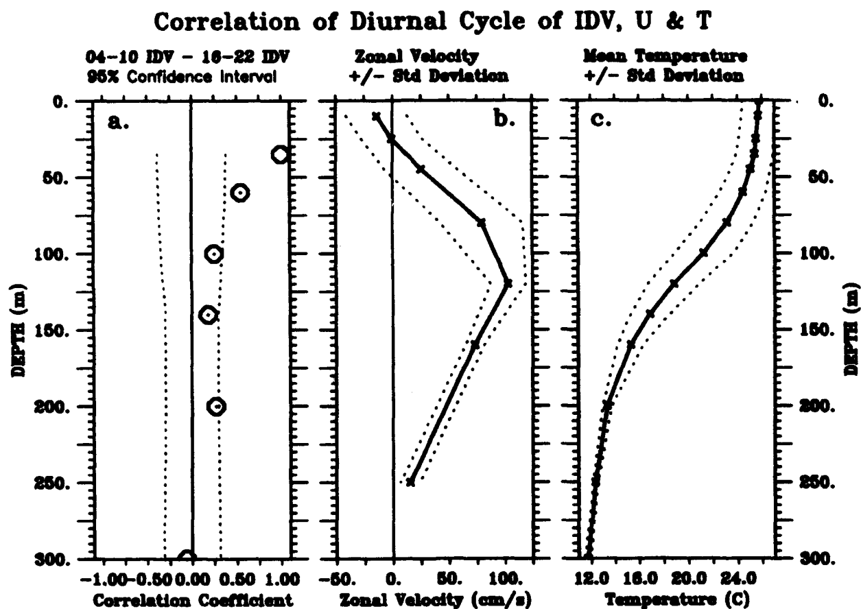
Figure 6.4. Vertical profiles of a) correlation coefficients between monthly mean diurnal differences of isotherm displacement variance ( \Delta IDV_m ) at 35 m and those at 60 m, 100 m, 140 m, 200 m, and 300 m, b) long-term mean zonal velocity, and c) long-term mean temperature. Dashed lines indicate a) 95% confidence intervals based on integral time scales between time series (Davis, 1976), and b) and c) standard deviations.
