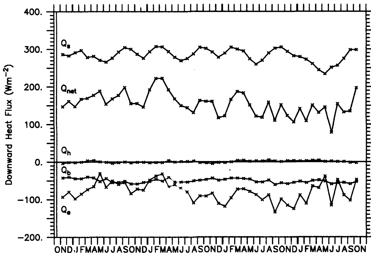
Surface Heat Balance at 0,140W (Nov83 – Oct87)
