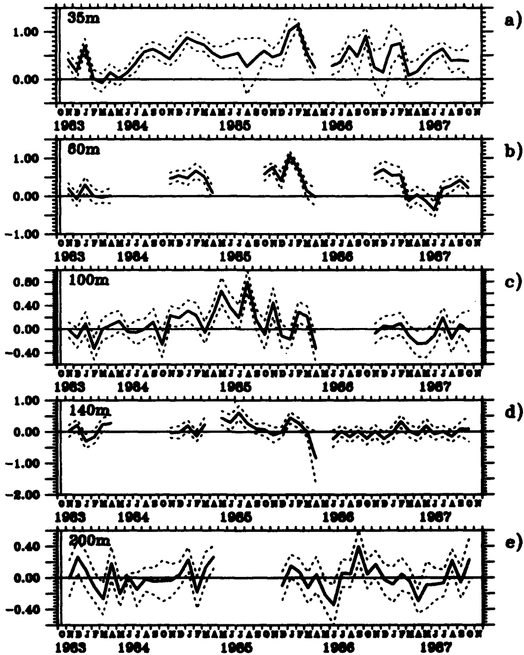
Figure 6.1. Monthly mean normalized diurnal differences of isotherm displacement variance ( \Delta IDV_m ) computed from daily values of 0400-1000 IDV minus 1600-2200 IDV at a) 35 m, b) 60 m, c) 100 m, d) 140 m, and e) 200 m. Daily diurnal differences were normalized by the mean of the morning and evening IDV values for each day. Dashed lines indicate \pm one standard error of the mean.
