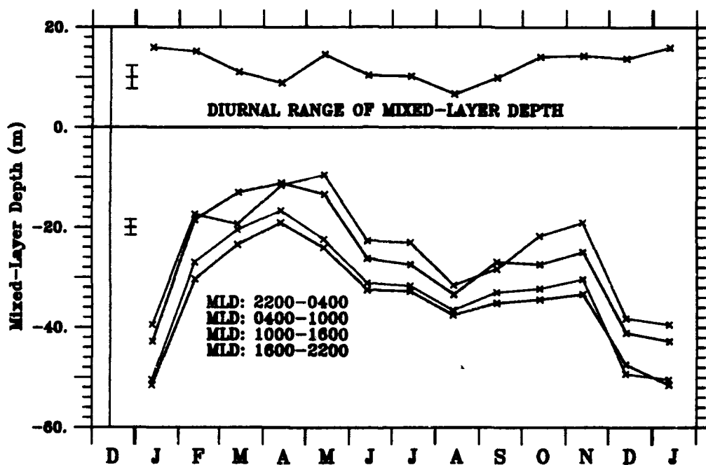
SEASONAL CYCLE OF MIXED-LAYER DEPTH & DIURNAL RANGE
