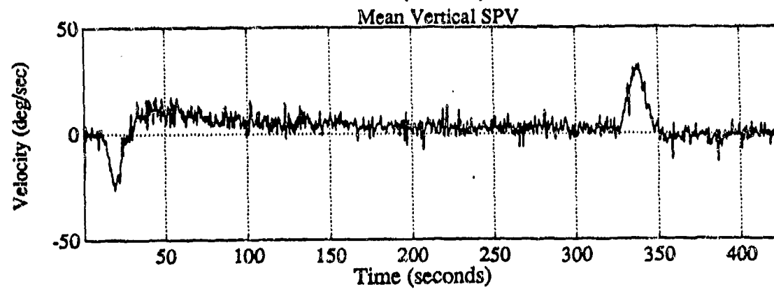
Figure 5.43: Subject 6 Average SPV a. Clockwise b. CounterClockwise
