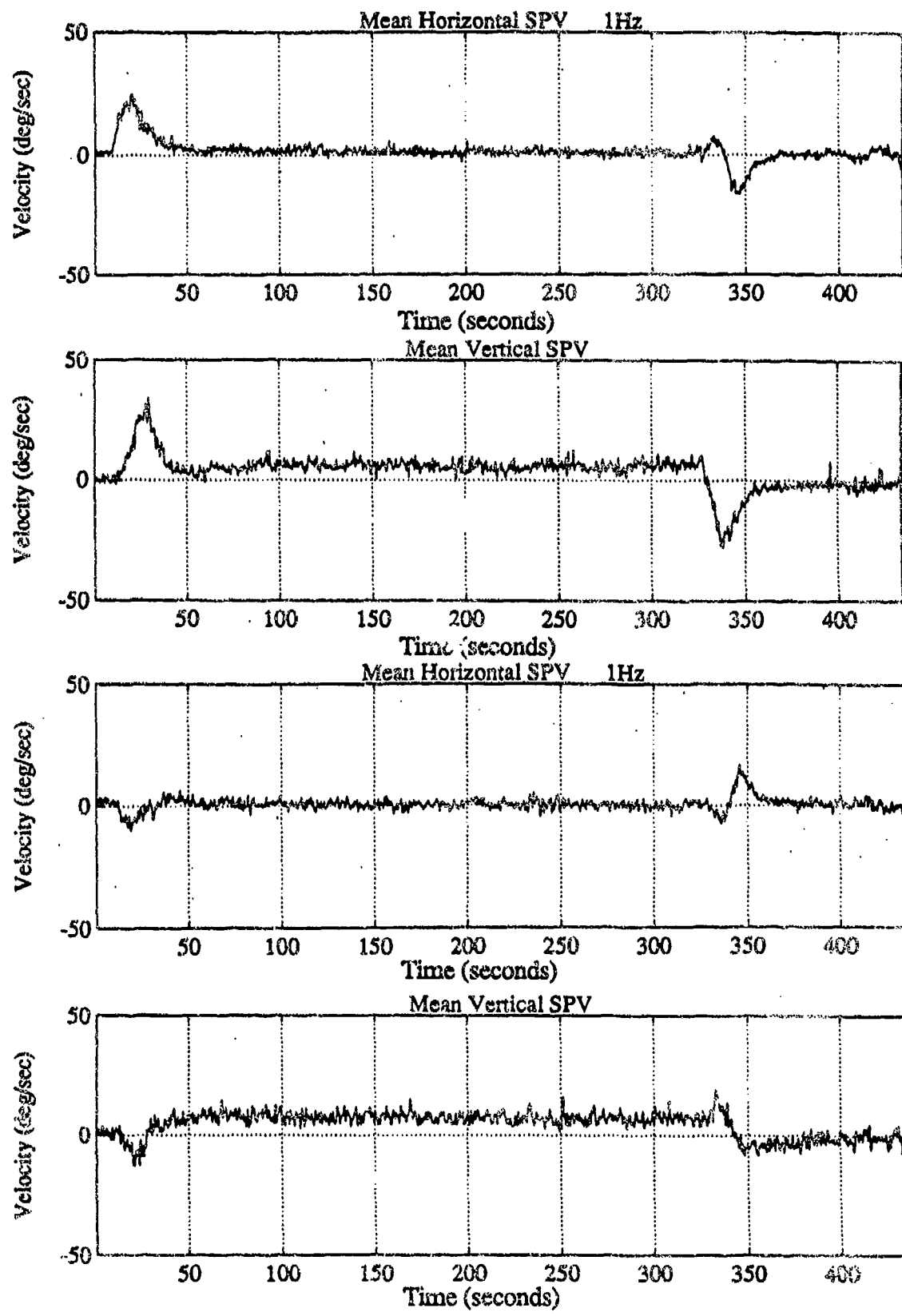
Figure 5.46: Subject 10 Average SPV a. Clockwise b. CounterClockwise
