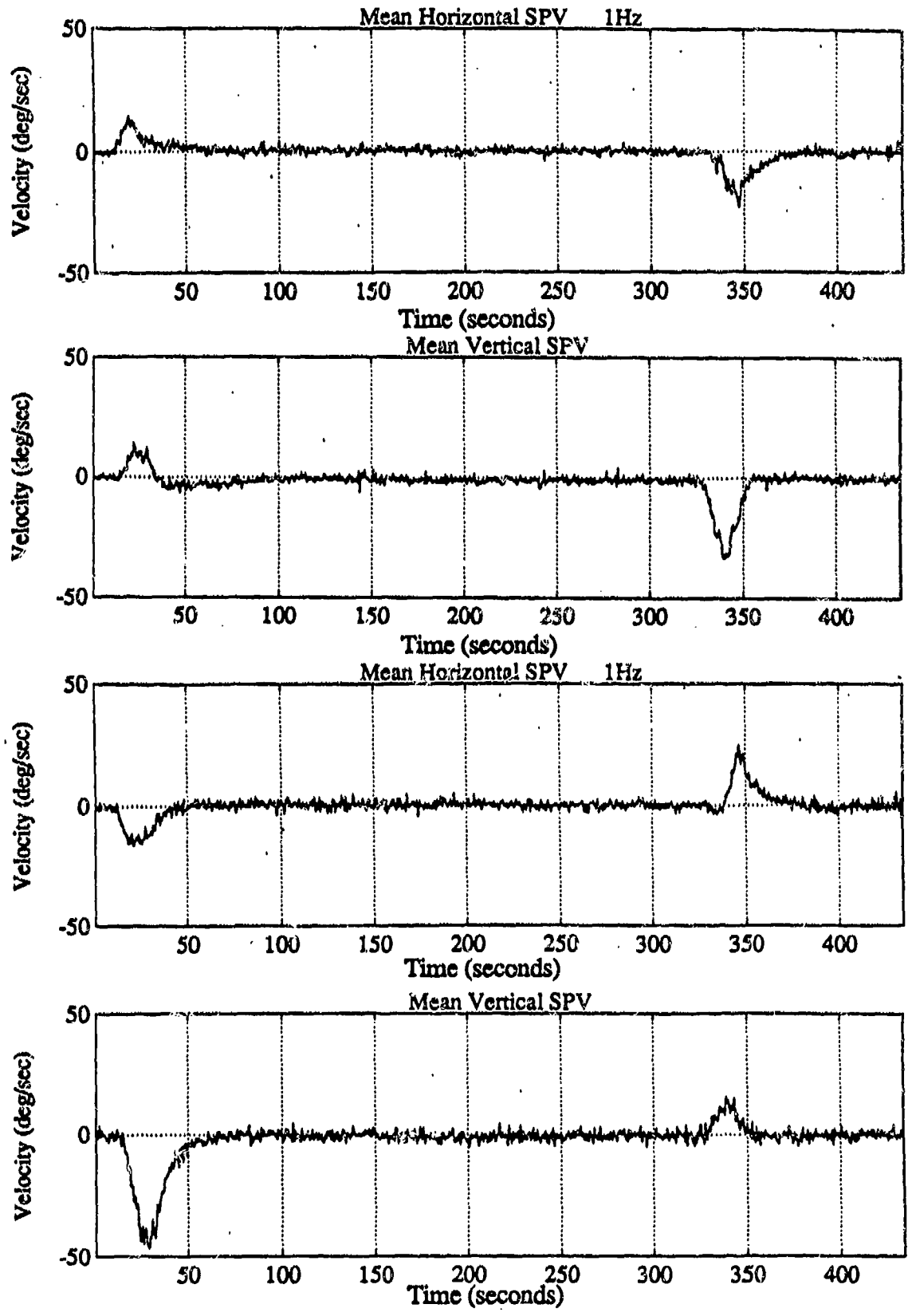
Figure 5.49: Subject 18 Average SPV a. Clockwise b. CounterClockwise
