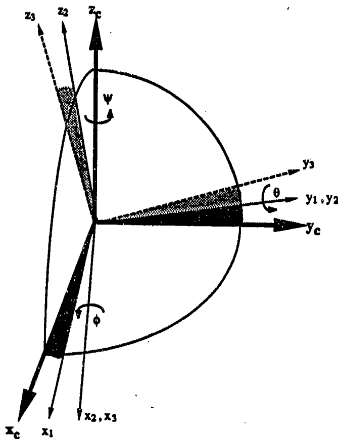
Figure 4.3: Definition of Euler Angles.
