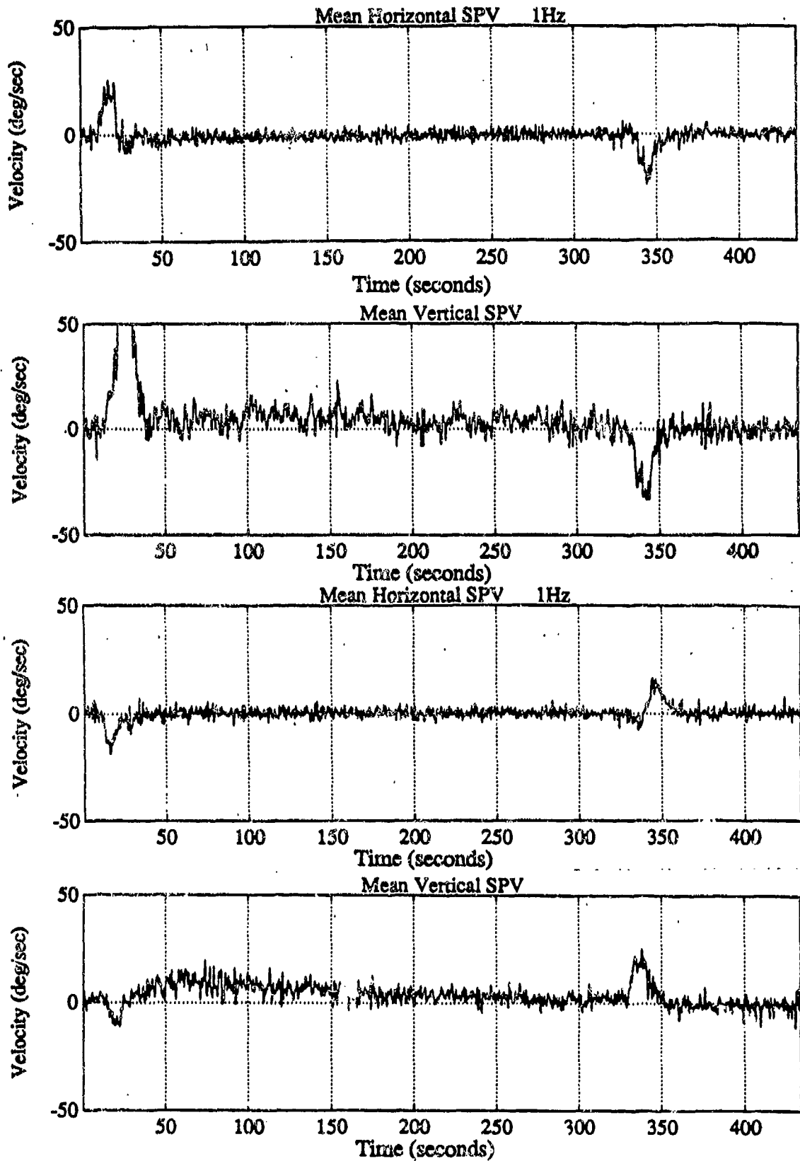
Figure 5.42: Subject 5 Average SPV a. Clockwise b. CounterClockwise
