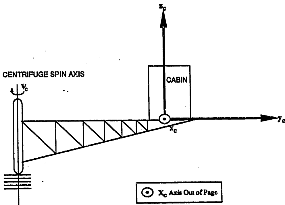
Figure 4.2: Capsule Fixed Coordinate System.
