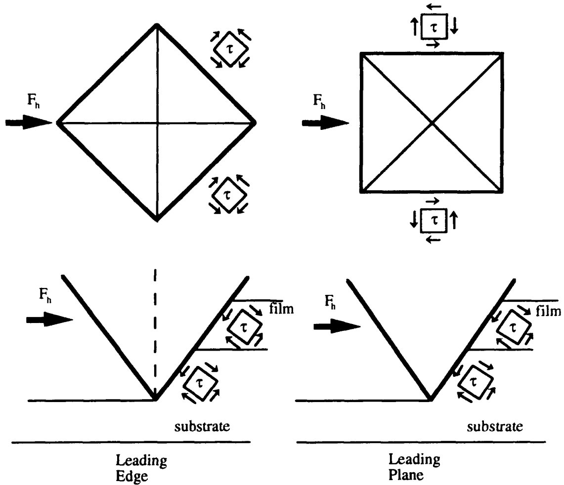
Figure 1.2: Orientation of Shear Stresses with Respect to Indenter Motion.
