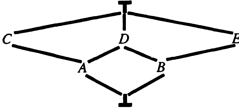
Figure 2.1: An Example of a Lattice.
