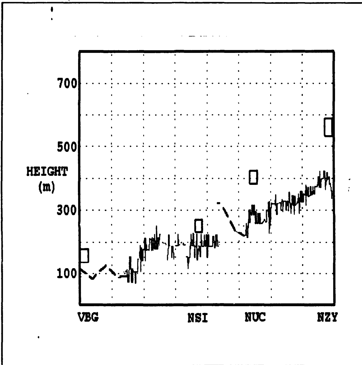
Figure 19: Offshore satellite-derived boundary layer height transect. The vertical axis is height in meters. Boxes represent depth of trapping layer from radiosonde measurements. Black dashed lines = IR Duct Technique.
