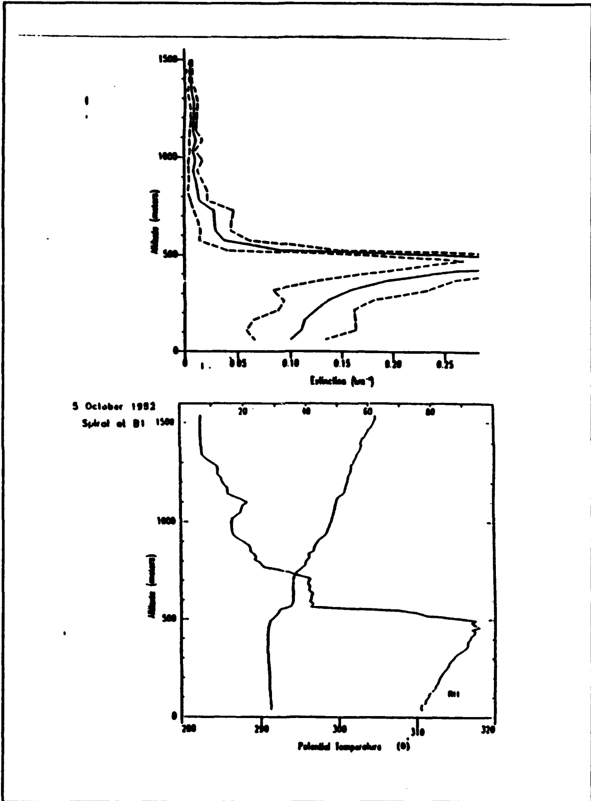
Figure 7: Profiles of extinction, potential temperature and relative humidity: Case B1 from Durkee (1984).
