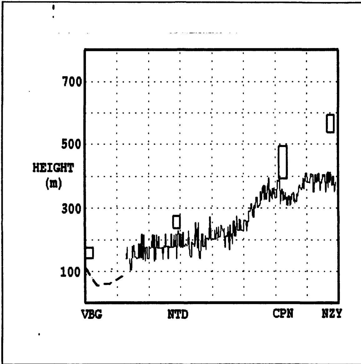
Figure 17: Coastal satellite-derived boundary layer height transect. The vertical axis is height in meters. Boxes represent depth of the trapping layer from radiosonde measurements. Black dashed line = the IR Duct Technique.
