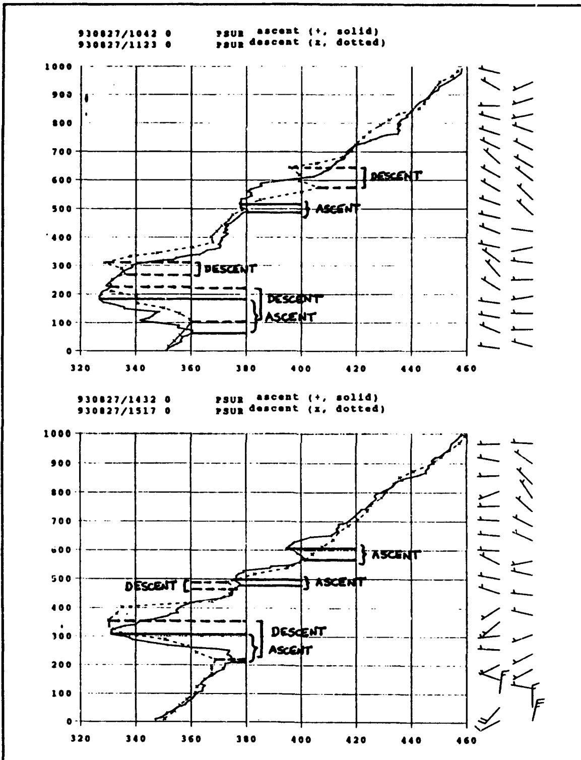
Figure 21: Consecutive up/down soundings from the Pt. Sur on 27 Aug. Times: (a) ascent - solid line @ 1042z, descent - dotted line @ 1123z. (b) ascent - solid line @ 1432z, descent - dotted line @ 1517z. Trapping layers shown.
